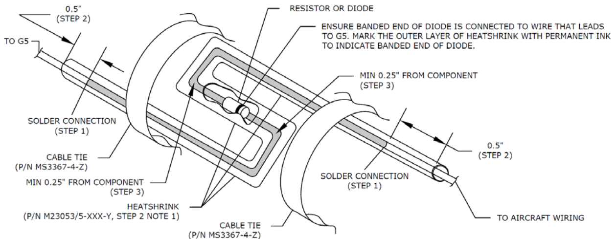
Figure 3-8 G5 Component Installation
