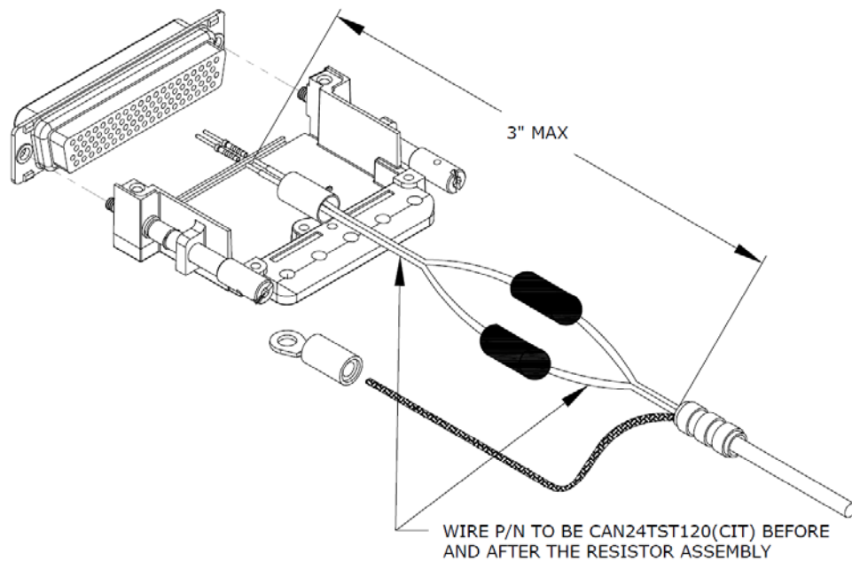
Figure 3-9 Placement of G5 CAN bus resistors using wire P/N CAN24TST120(CIT)
