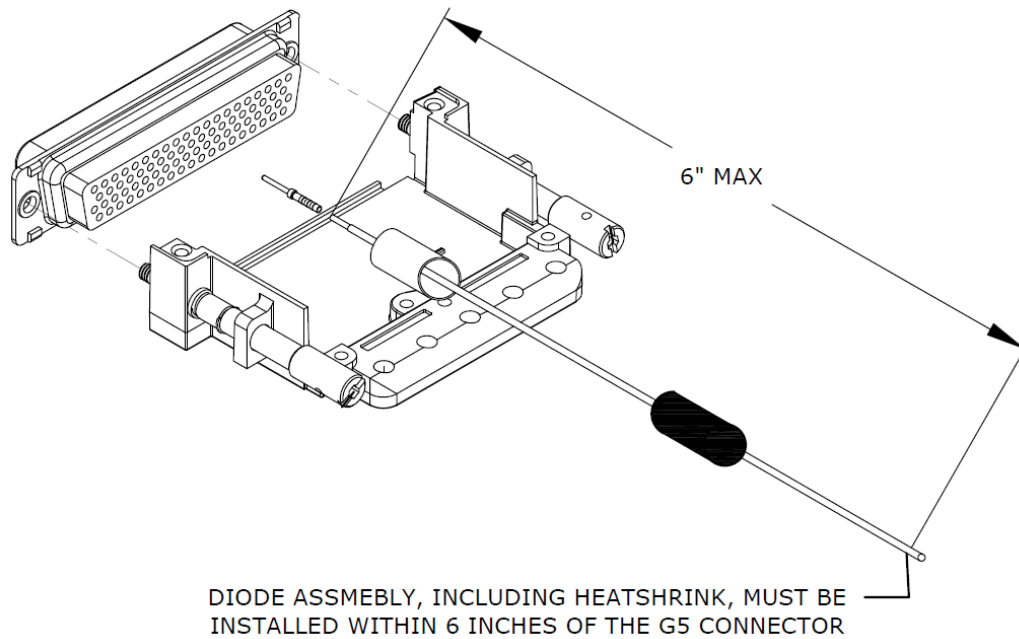
Figure 3-12 Placement of G5 power diode
