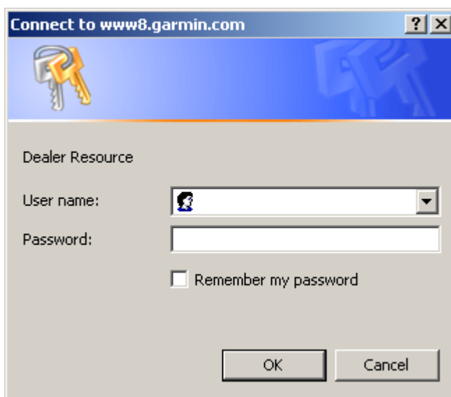
Figure 3.1 – Dealer Login
