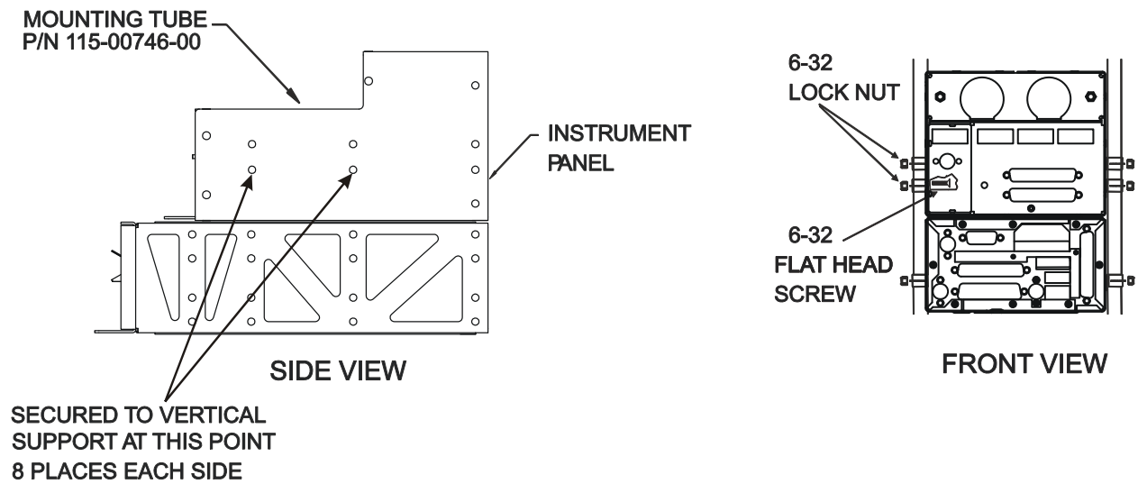
Figure D-5. Sample GNS 480 and GMX 200 Mounting with GNS 480
