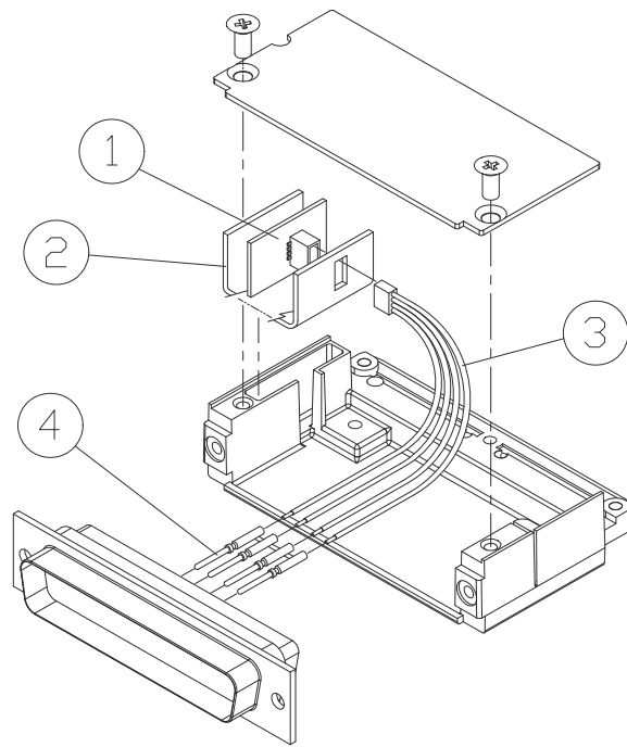
Figure 3-3. Configuration Module Installation
