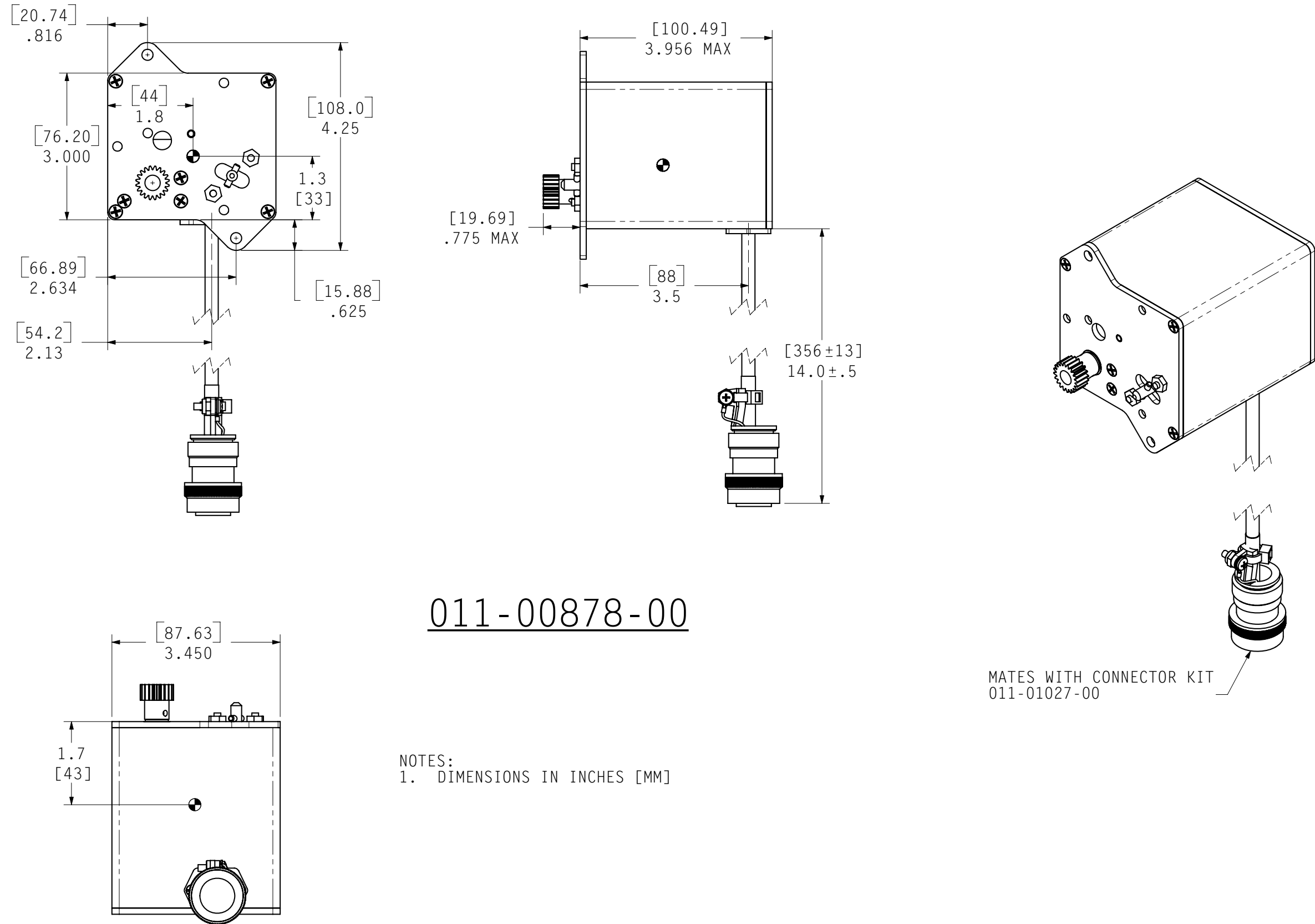
Figure A-2. GSA 81 (-00) Outline Drawing
