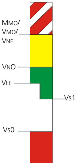
Typical Airspeed Tape Markings
