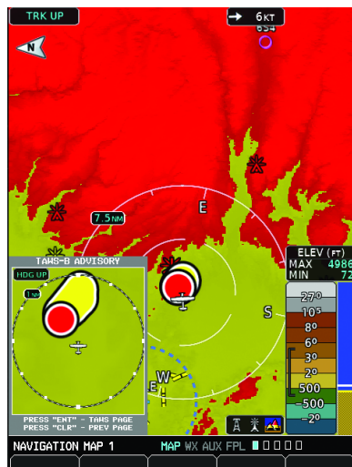
TAWS-B Pop-Up Alert on MFD
