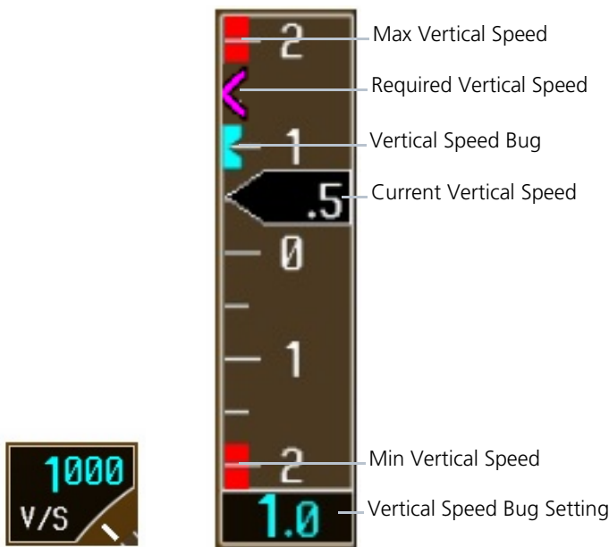
Vertical Speed (V/S) Tape and Window
