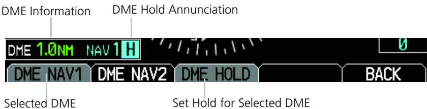
DME Indication
