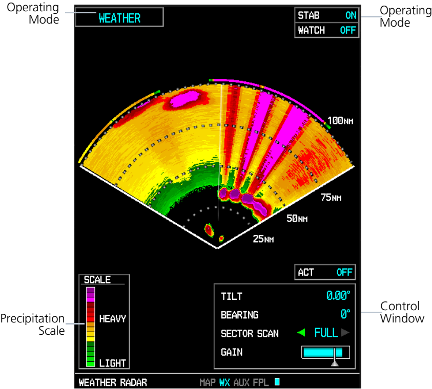
Weather Radar Display (GWX 75)
