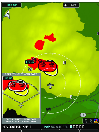
TERRAIN-SVT Pop-Up Alert on MFD
