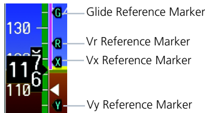
Reference Speeds
