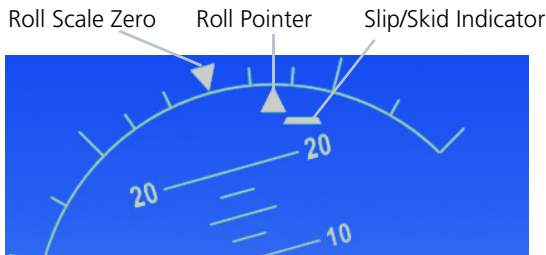
Slip/Skid Indicator
