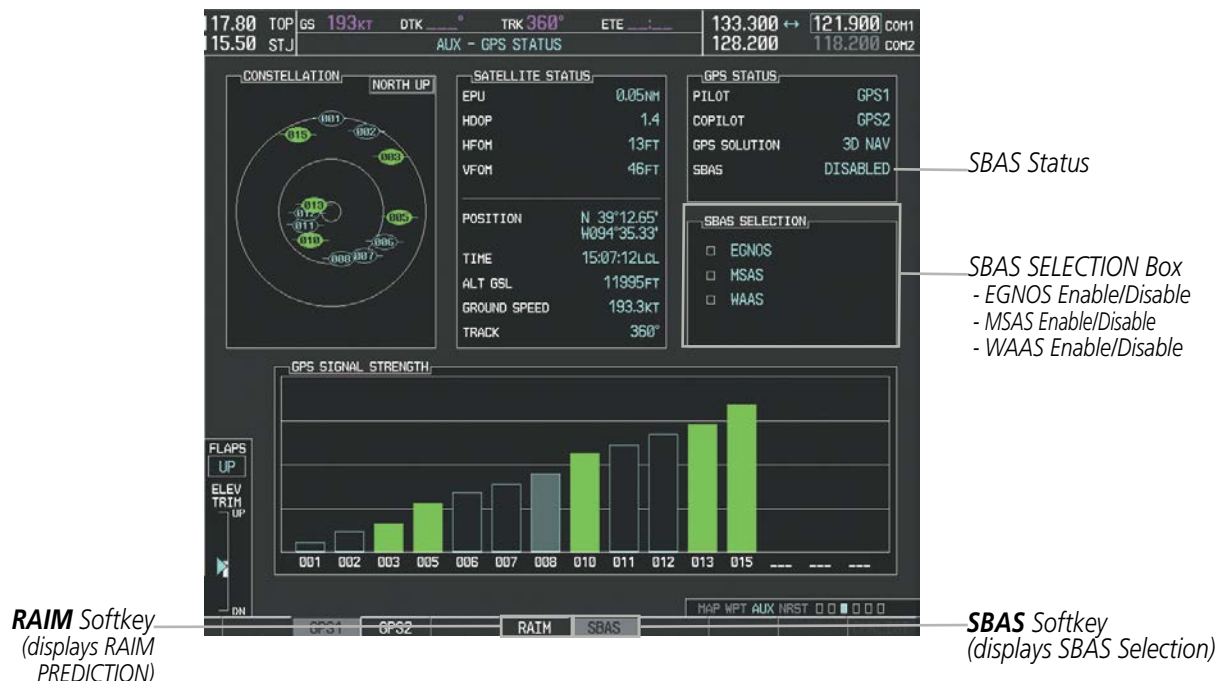
Figure 5-111 SBAS Display - Disabled
