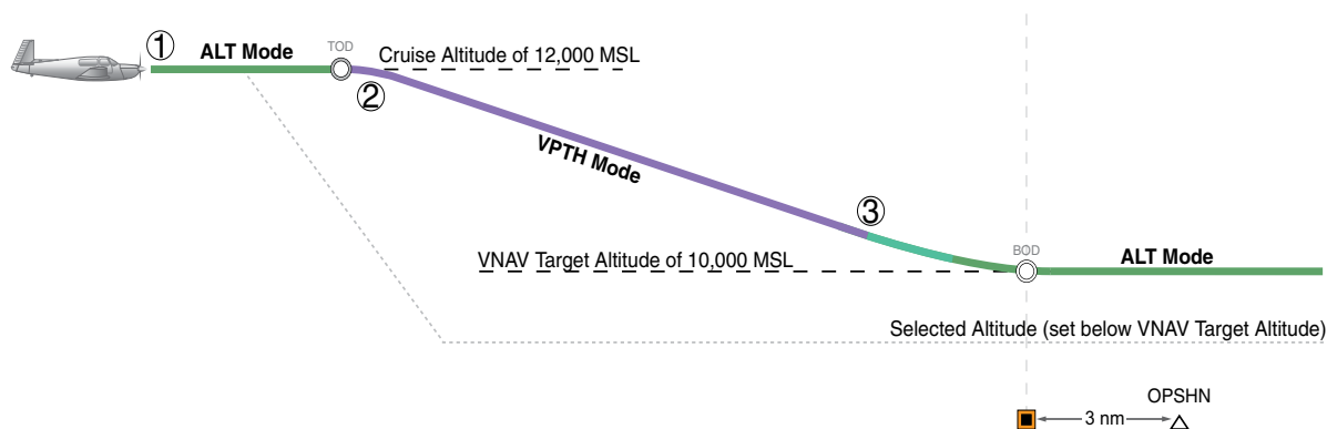
Figure 7-35 VPTH Descent
