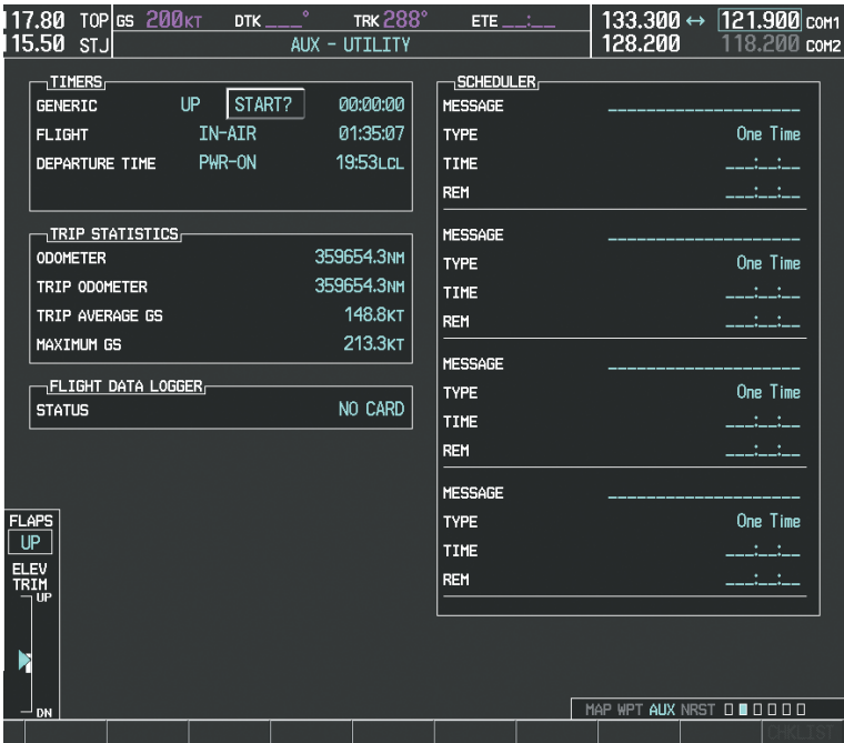
Figure 1-38 Utility Page
