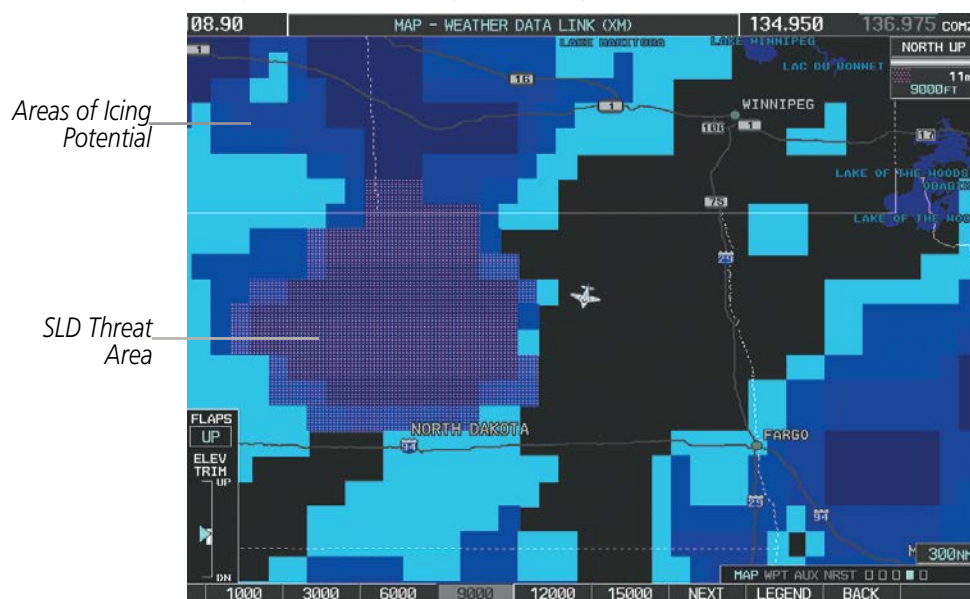
Figure 6-42 Icing Data at 9,000 Feet
