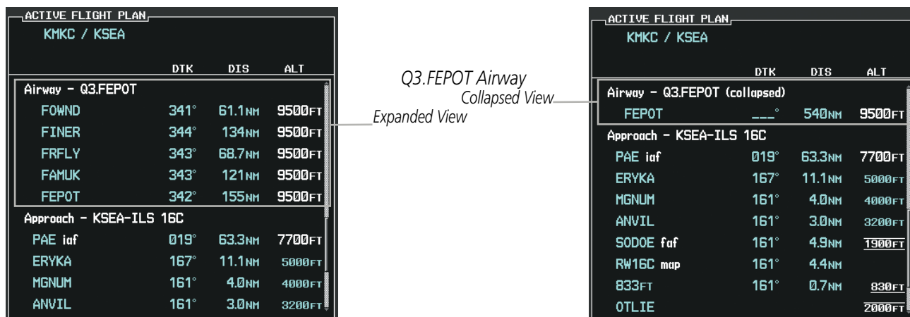
Figure 5-88 Expanded/Collapsed Airways
