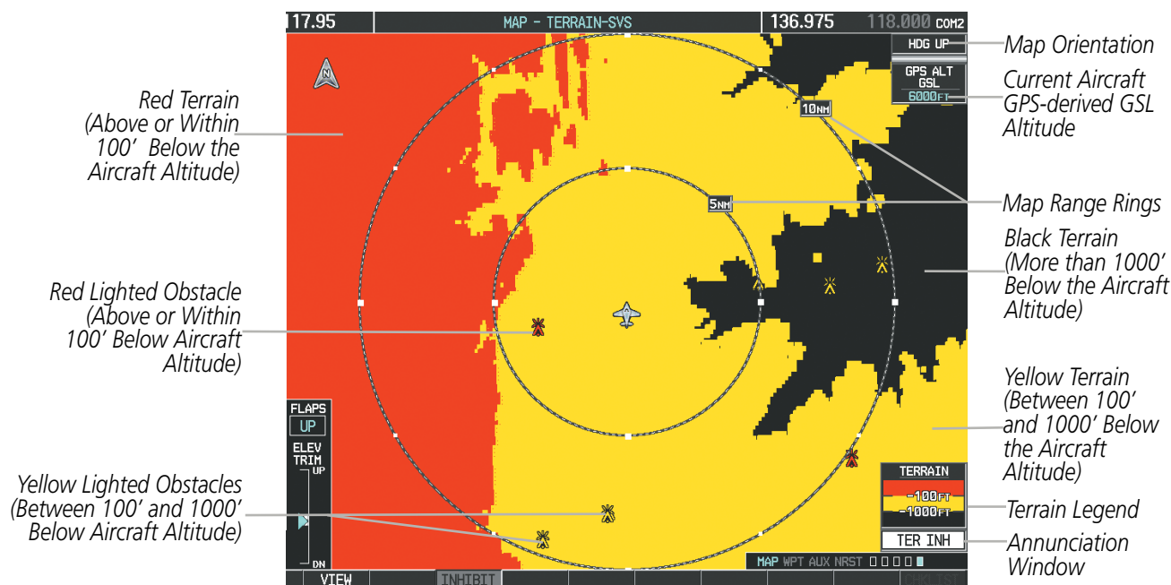
Figure 6-78 Terrain-SVS Page
