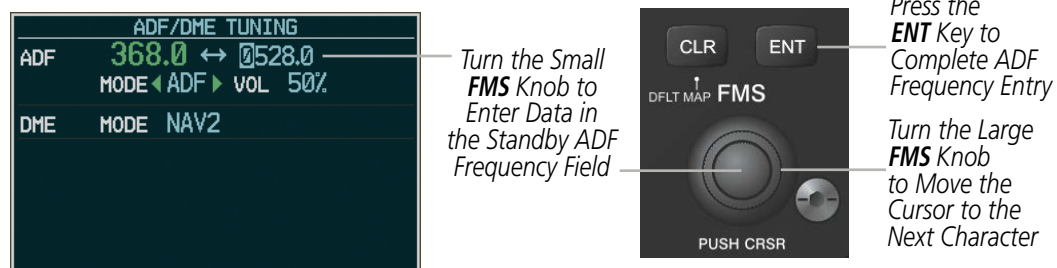
Figure 4-30 Entering ADF Standby Frequencies
