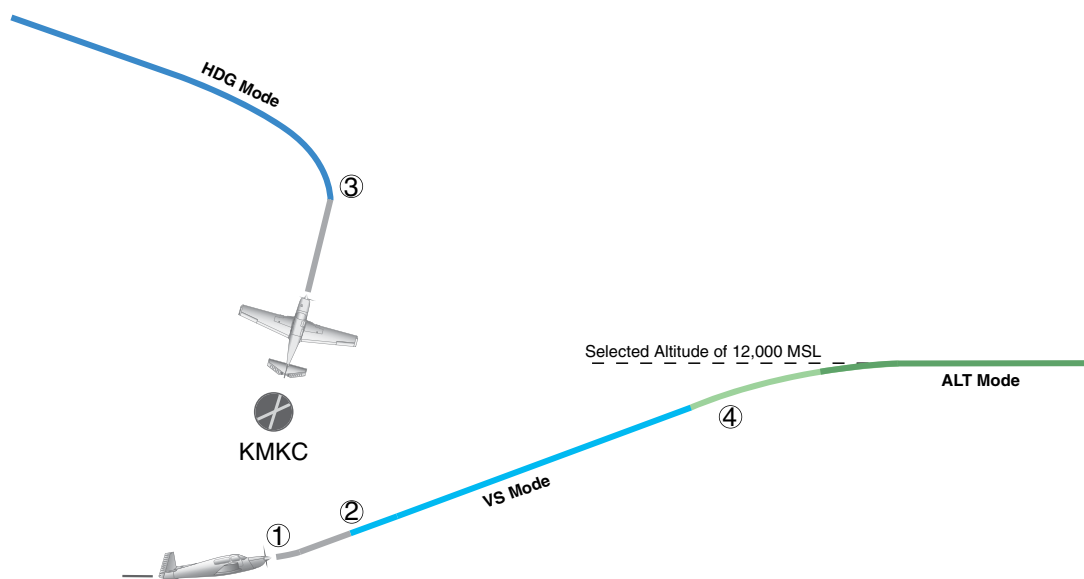
Figure 7-31 Departure
