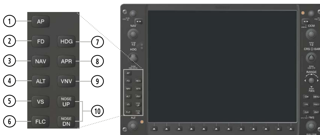
Figure 7-1 Dedicated MFD AFCS Controls
