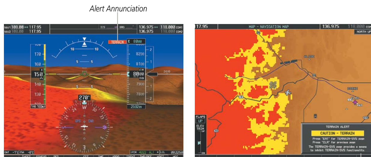
Figure 6-80 Terrain-SVS Alert Annunciations
