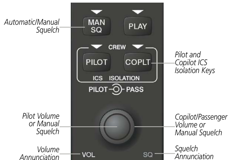
Figure 4-53 Audio Panel Controls
