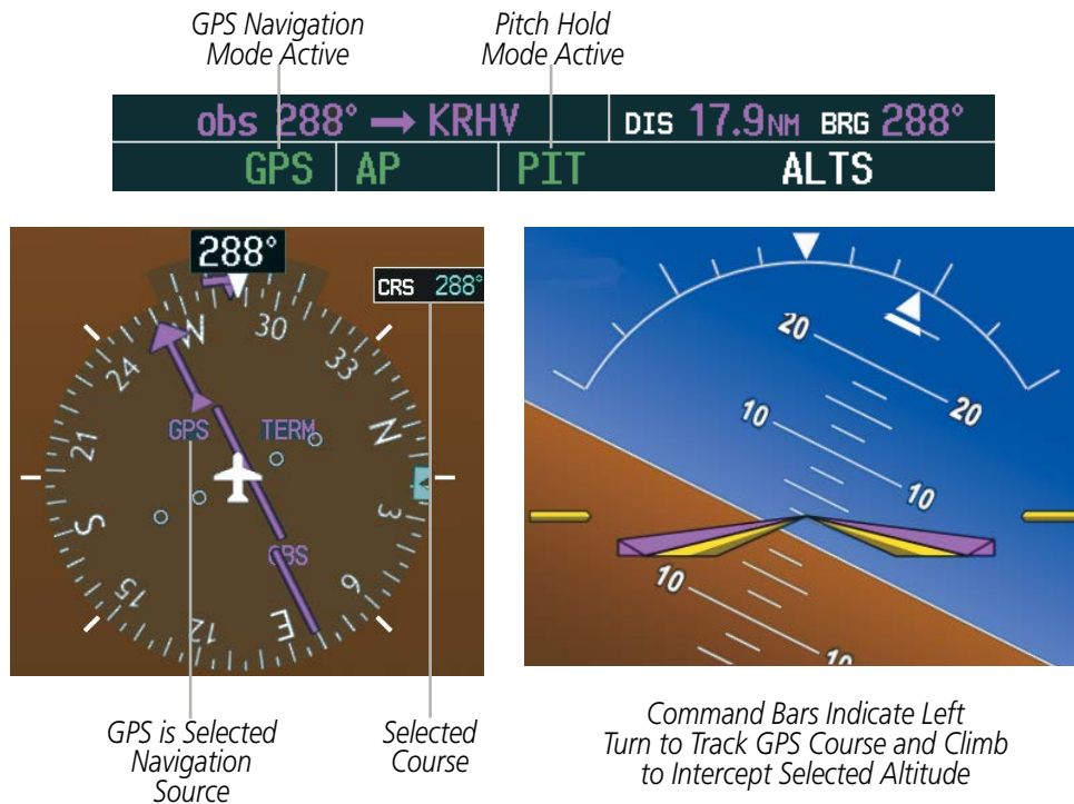
Figure 7-23 Navigation Mode
