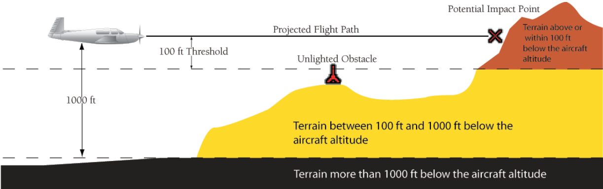
Figure 6-74 Terrain Altitude/Color Correlation for Terrain-SVS
