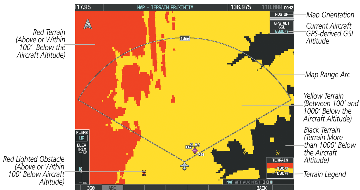
Figure 6-67 Terrain Proximity Page (ARC View)
