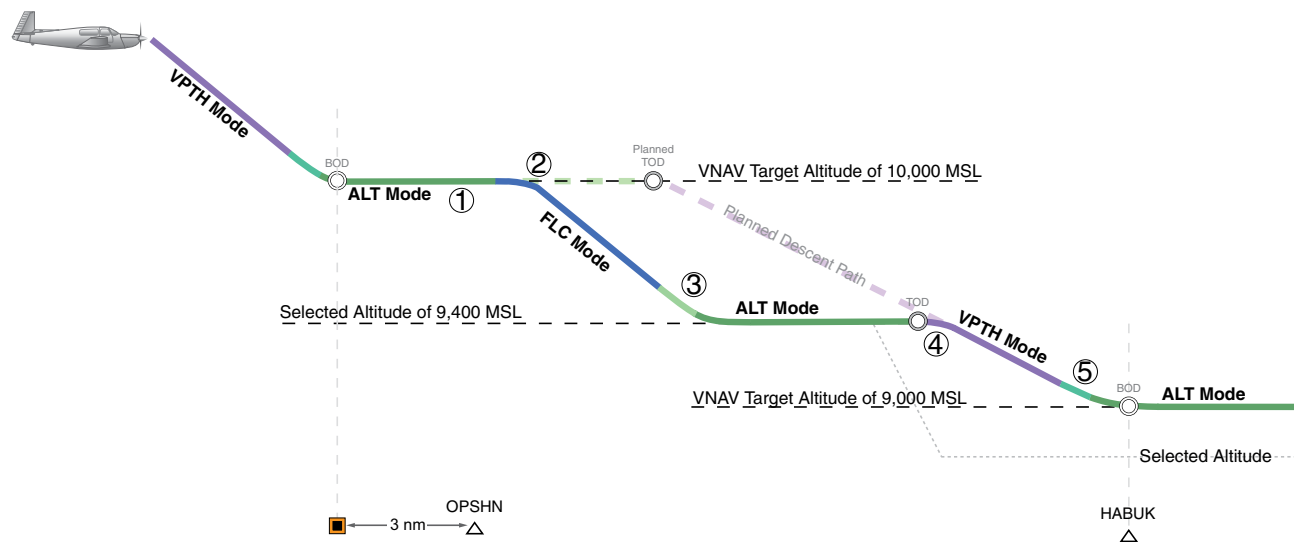
Figure 7-36 Non-path Descent
