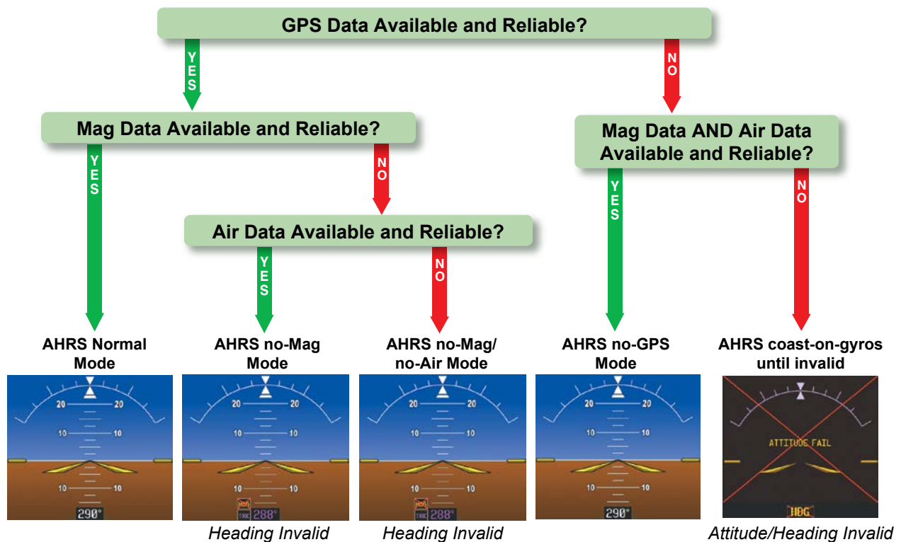
Figure 1-9 AHRS Operation
