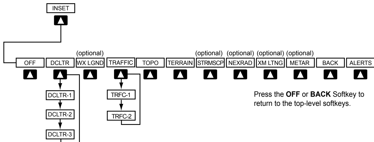
Figure 1-15 INSET Softkeys
