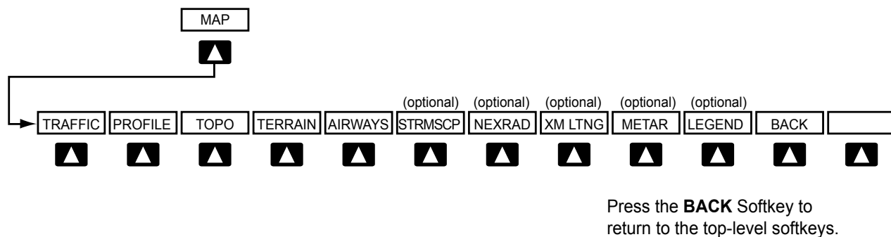
Figure 1-20 MAP Softkeys
