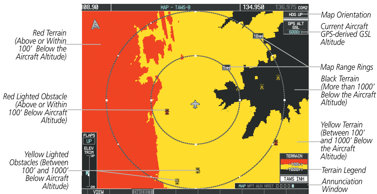
Figure 6-89 TAWS-B Page
