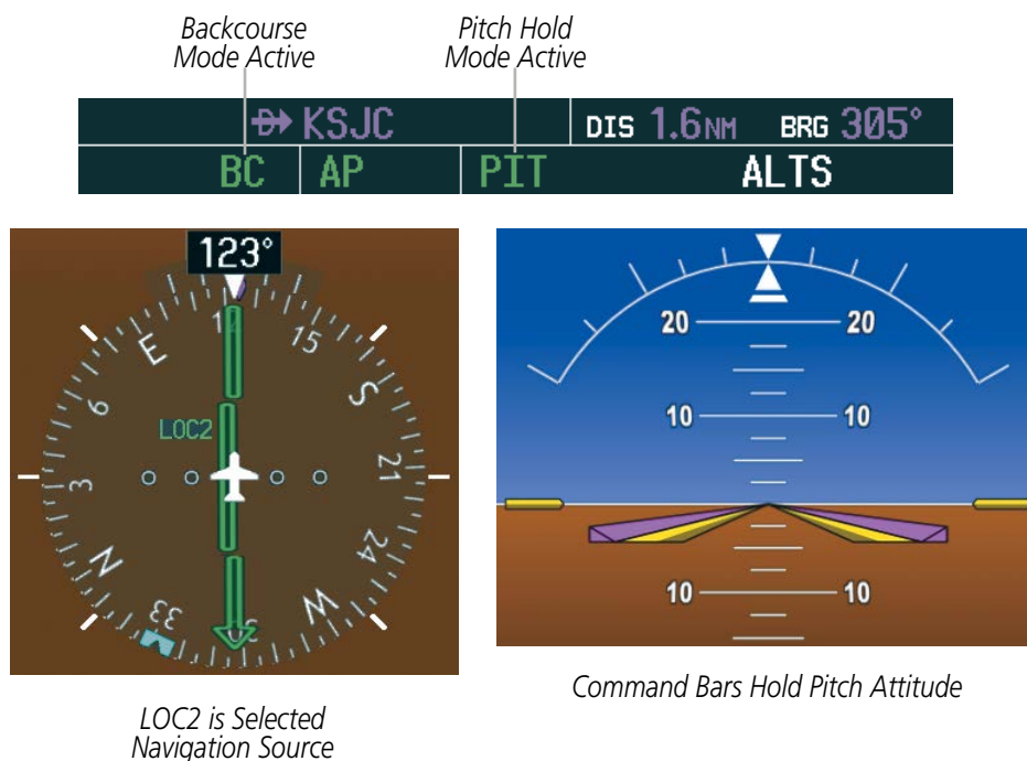
Figure 7-24 Backcourse Navigation Mode
