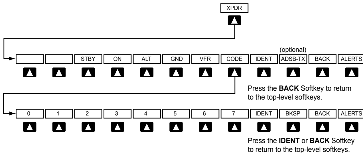
Figure 1-17 XPDR Softkeys
