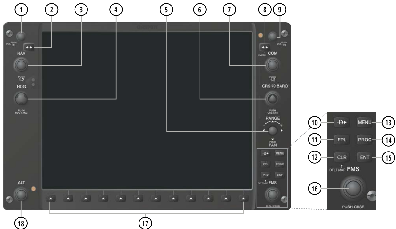
Figure 1-11 PFD/MFD Controls
