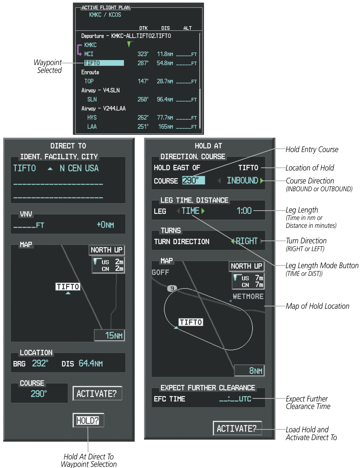
Figure 5-91 Creating a User Defined Holding Pattern at a Direct To Waypoint
