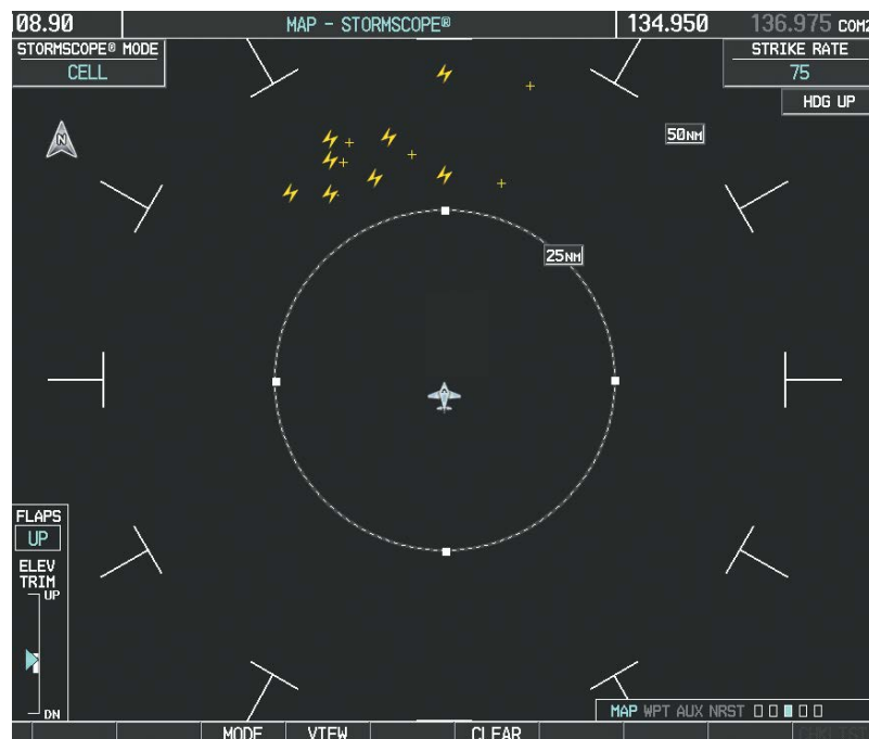
Figure 6-60 Stormscope Page
