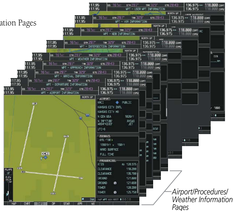
Figure 1-25 Waypoint Pages
