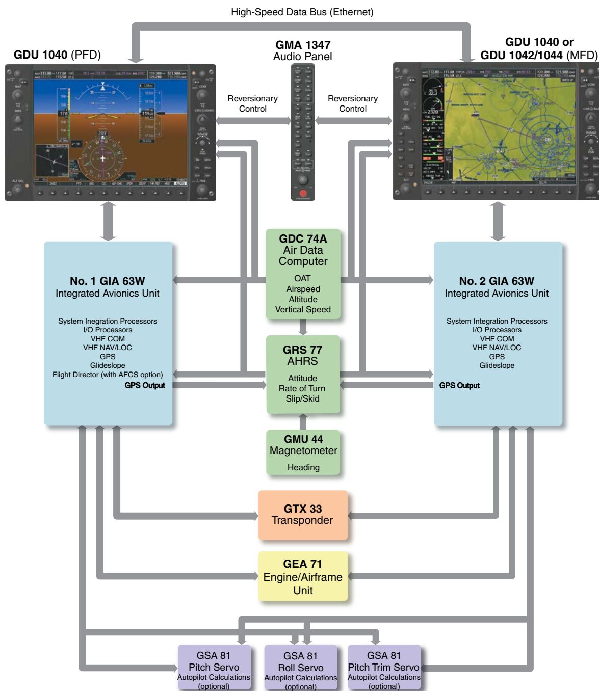
Figure 1-1 Basic G1000 System Block Diagram
