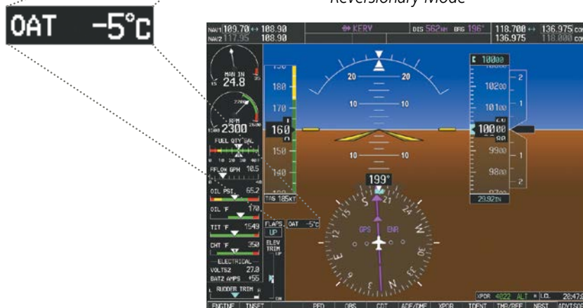
Figure 2-27 Outside Air Temperature
