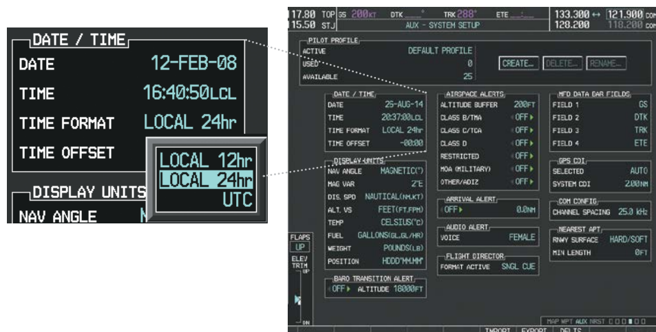
Figure 1-35 Date/Time Settings (System Setup Page)
