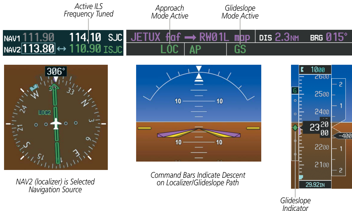
Figure 7-18 Glideslope Mode
