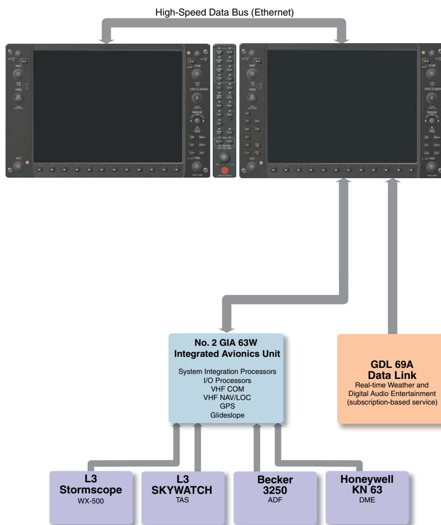
Figure 1-2 G1000 System Block Diagram With Options
