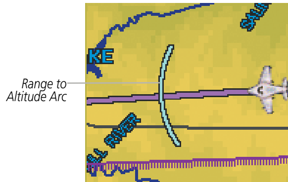
Figure 5-30 Navigation Map - Range to Altitude Arc
