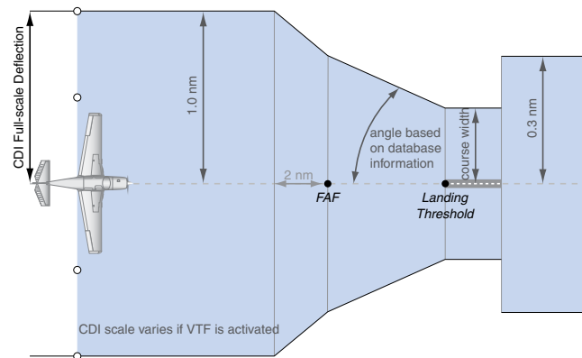
Figure 2-24 Typical LNAV/VNAV, LP, LPV, and LP+V Approach CDI Scaling
