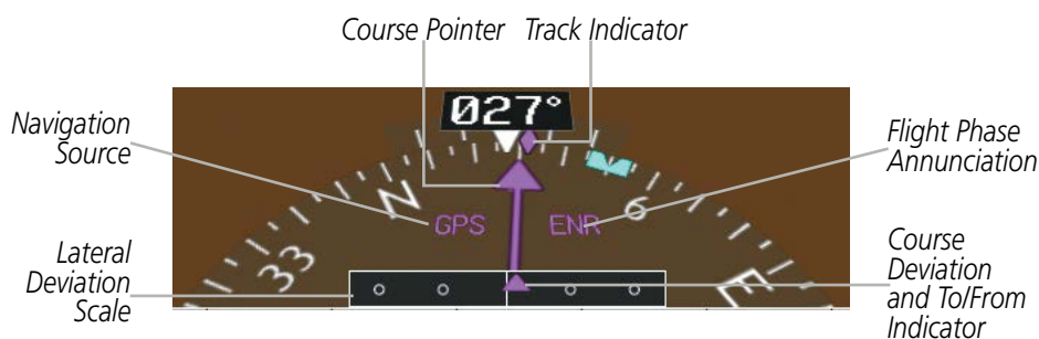
Figure 2-11 Arc HSI
