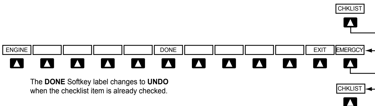
Figure 1-21 Checklist Softkeys
