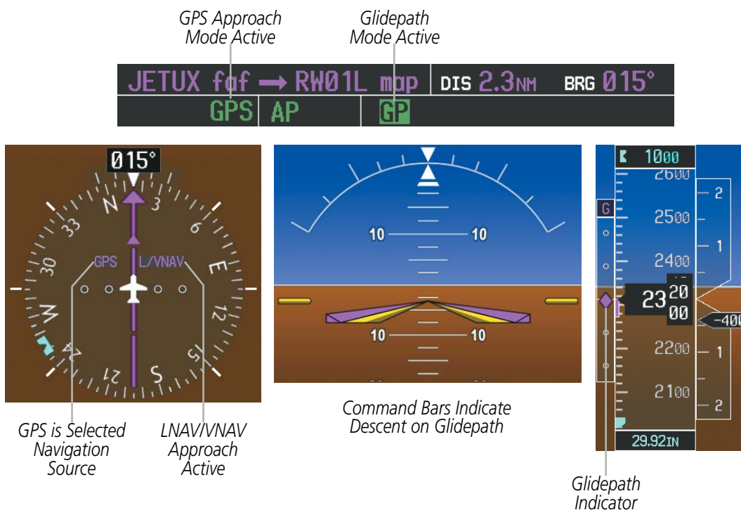
Figure 7-16 Glidepath Mode
