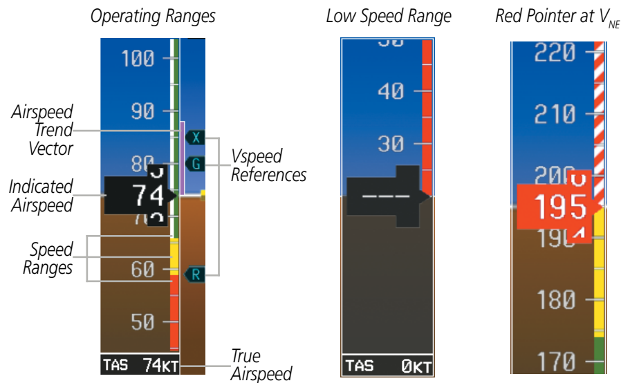
Figure 2-3 Airspeed Indicator
