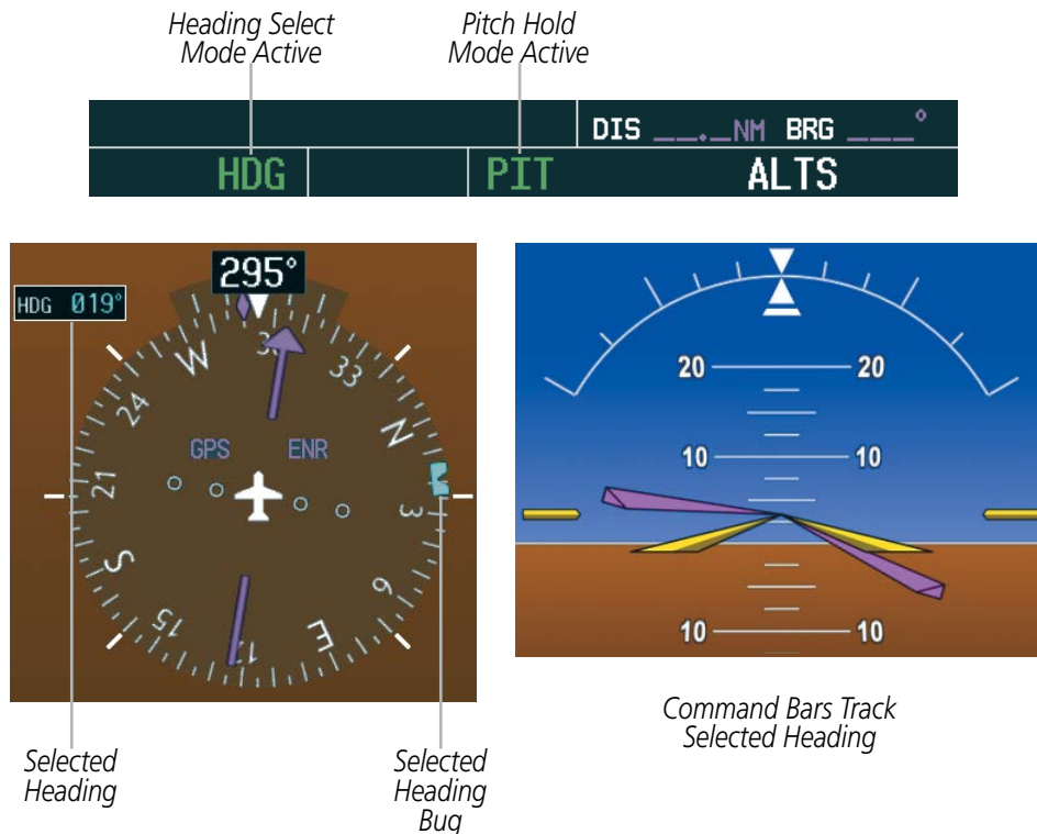
Figure 7-21 Heading Select Mode
