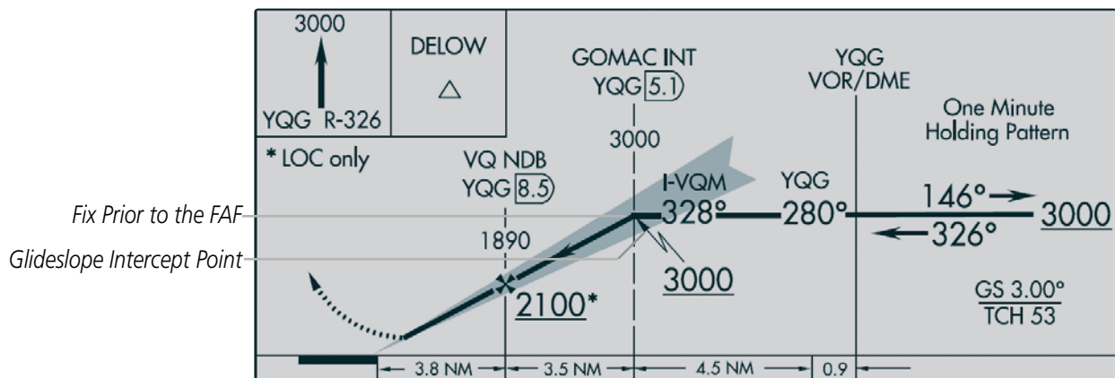
Figure 2-20 ILS Approach with Glideslope Intercept Point at Fix Prior to the FAF
