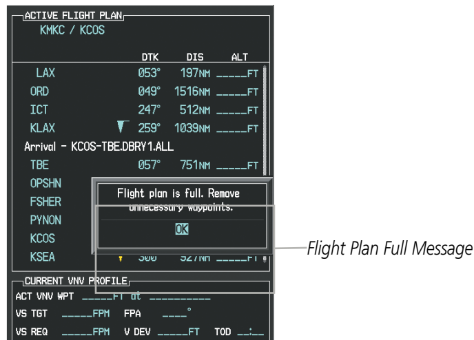
Figure 5-62 Active Flight Plan Page - FPL Full
