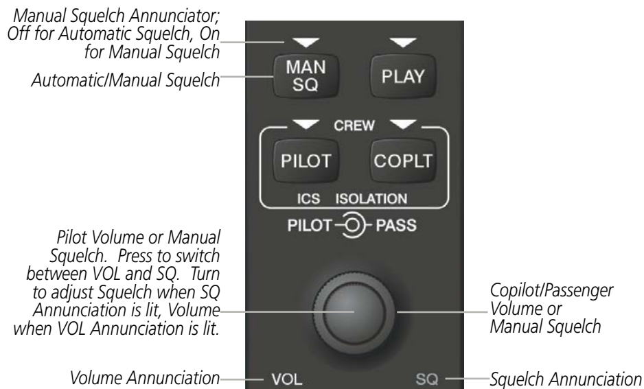
Figure 4-49 Volume/Squelch Control
