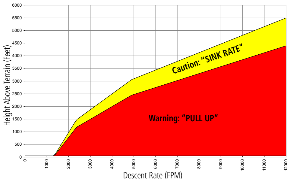
Figure 6-93 Excessive Descent Rate Alert Criteria
