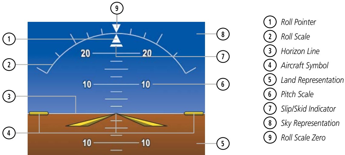
Figure 2-5 Attitude Indicator
