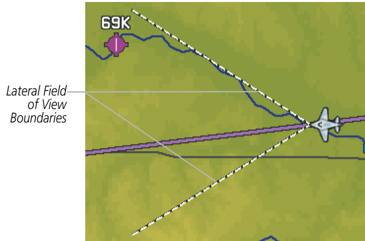
Figure 5-31 Navigation Map - Field of View
