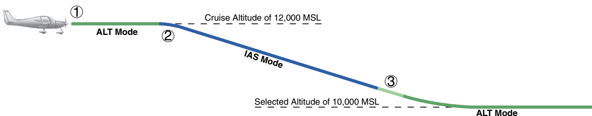
Figure 7-35 IAS Descent
