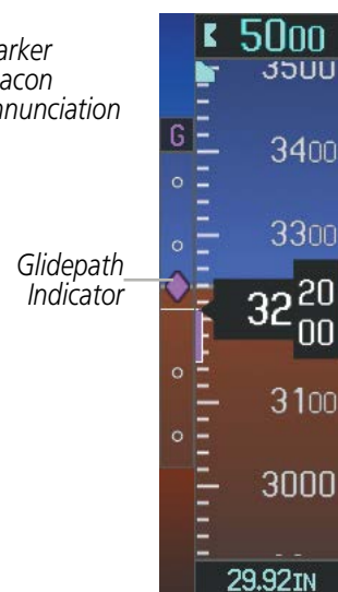
Figure 2-11 Glidepath Indicator
