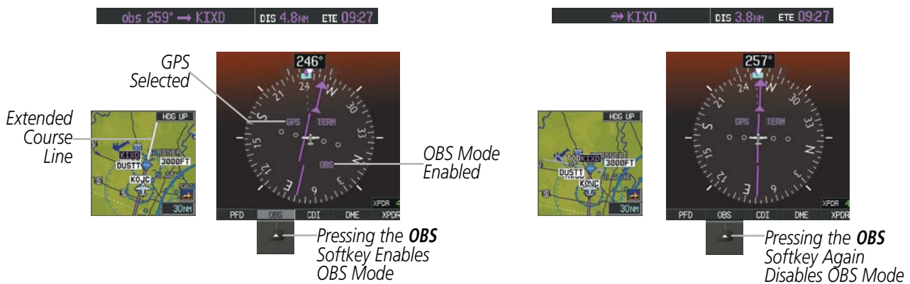
Figure 2-26 Omni-bearing Selector (OBS) Mode
