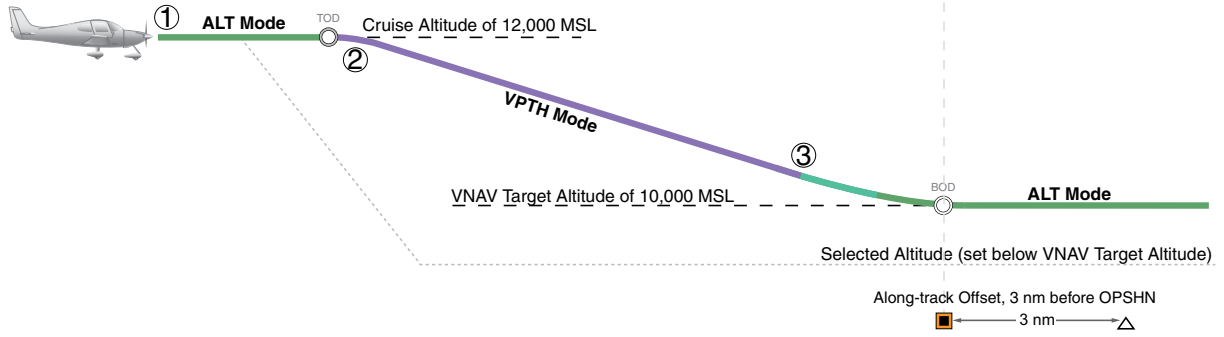
Figure 7-36 VPTH Descent
