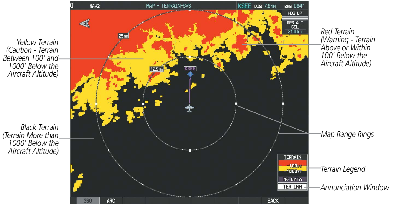
Figure 6-143 Terrain-SVS Page
