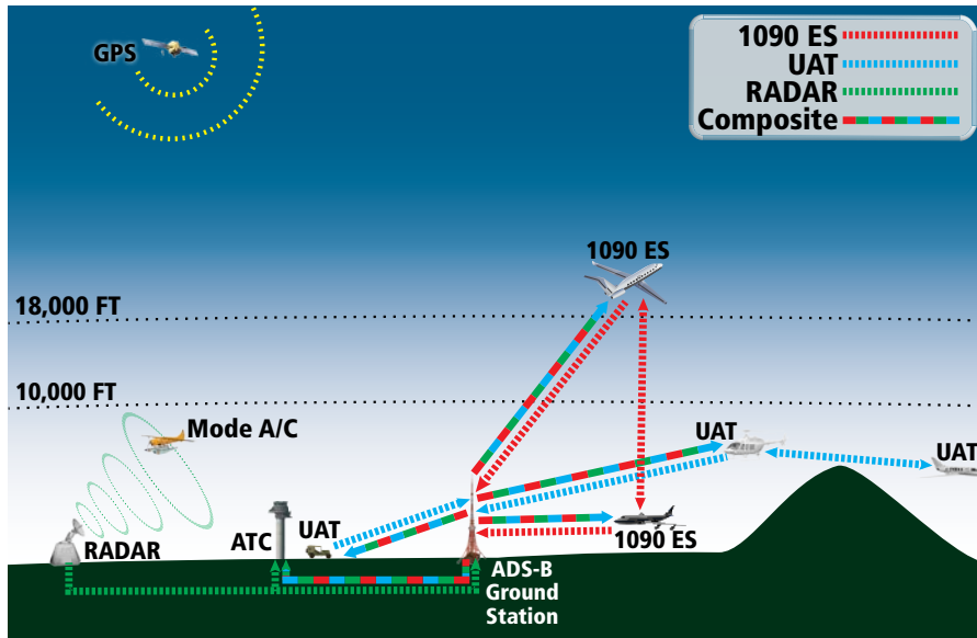
Figure 6-193 ADS-B System
