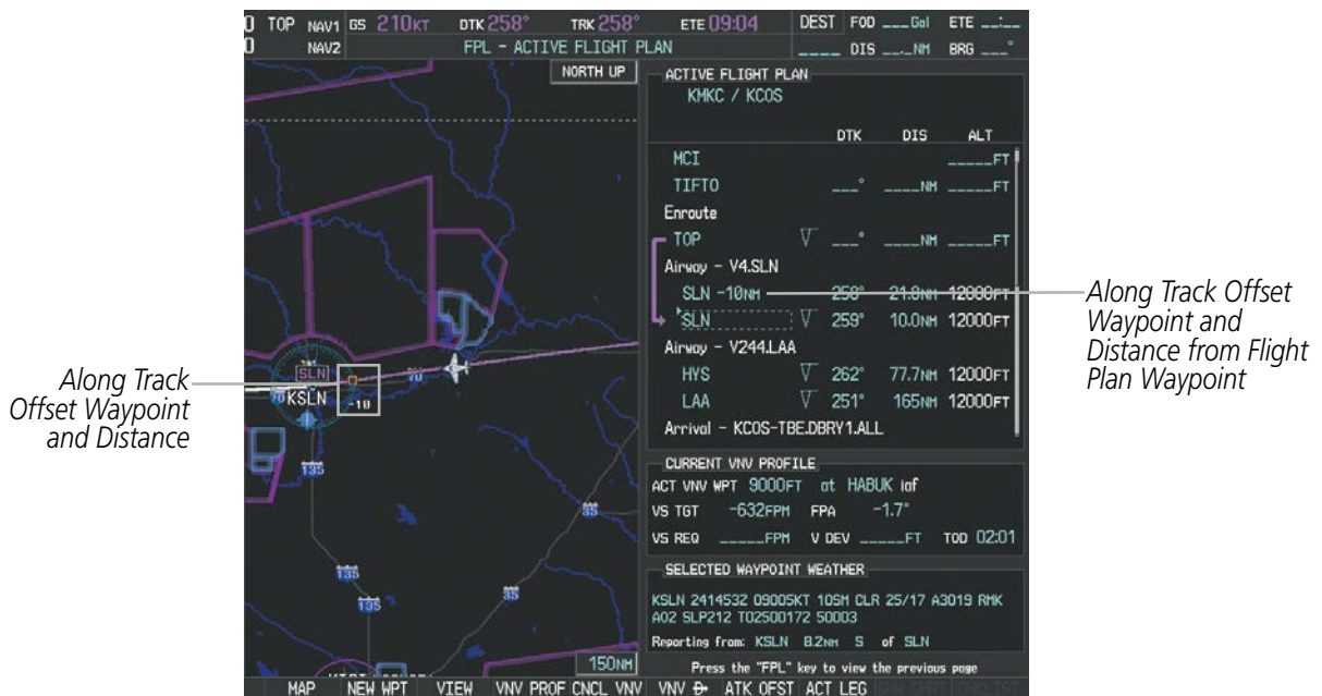
Figure 5-86 Along Track Offset
