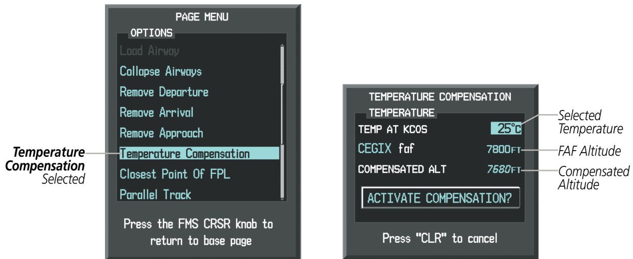
Figure 5-111 Temperature Compensation
