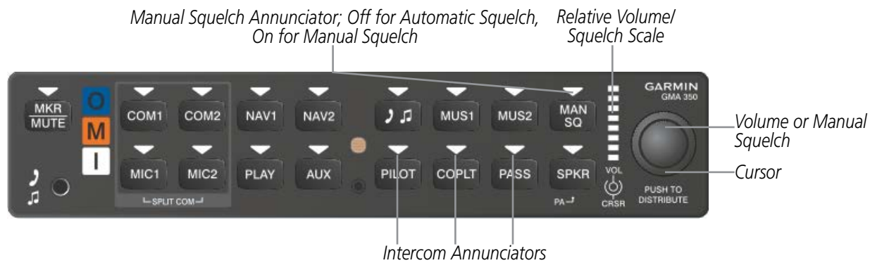
Figure 4-58 Audio Panel Controls
