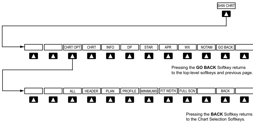
Figure 8-24 ChartView SHW CHRT, Chart Selection, and Chart Option Softkeys
