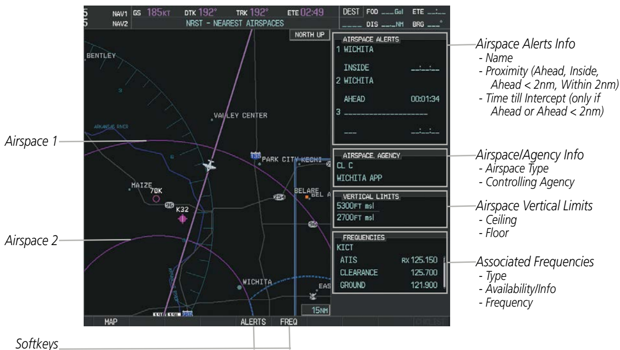
Figure 5-55 Nearest Airspaces Page
