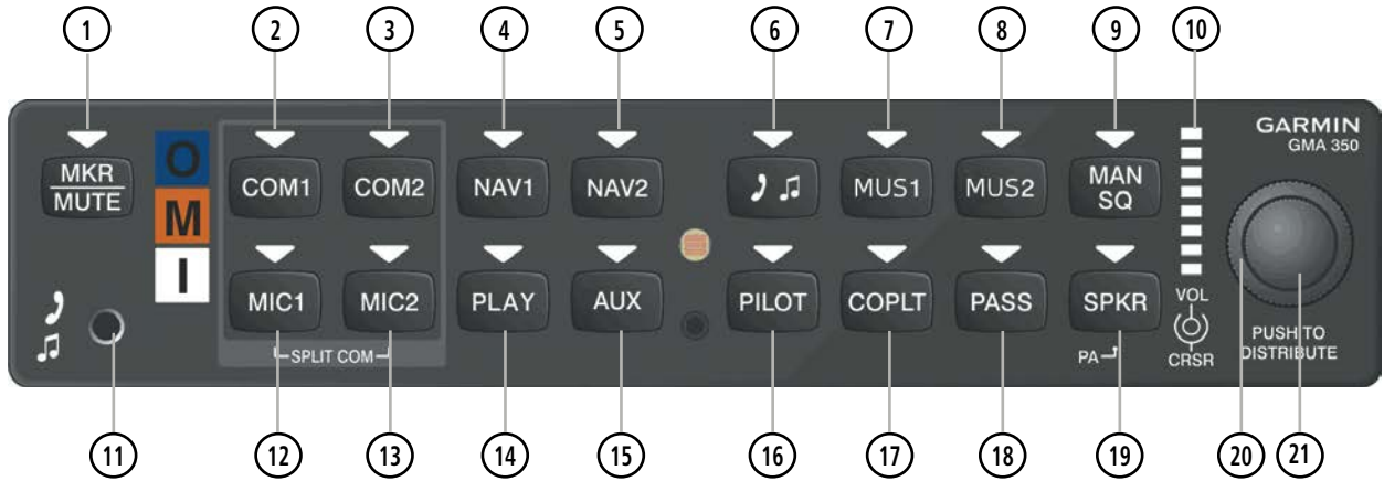
GMA 350 Controls
