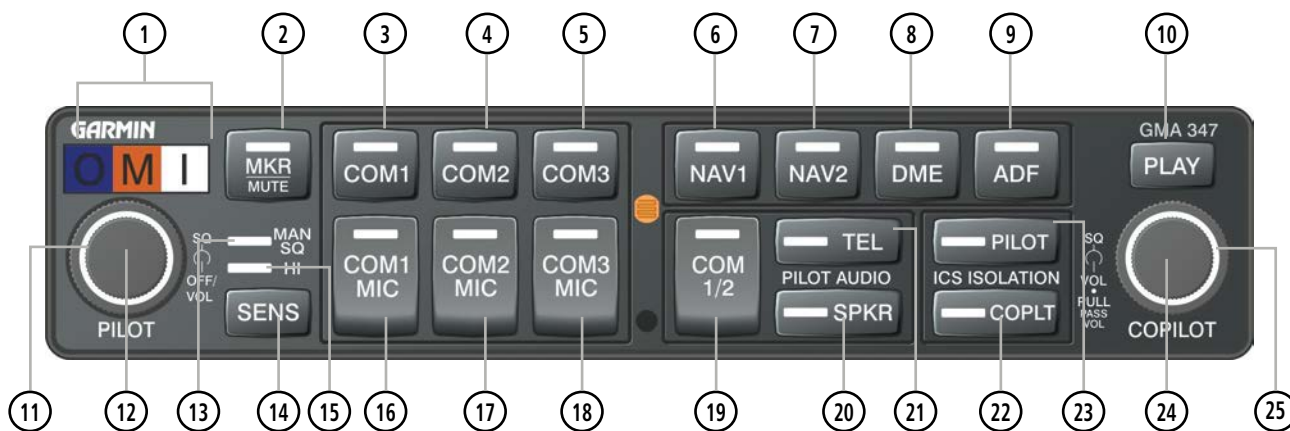
Figure 4-4 GMA 347 Audio Panel Controls
