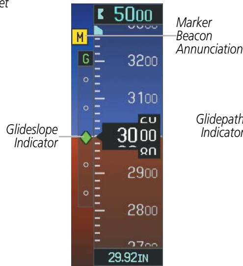
Figure 2-10 Glideslope Indicator
