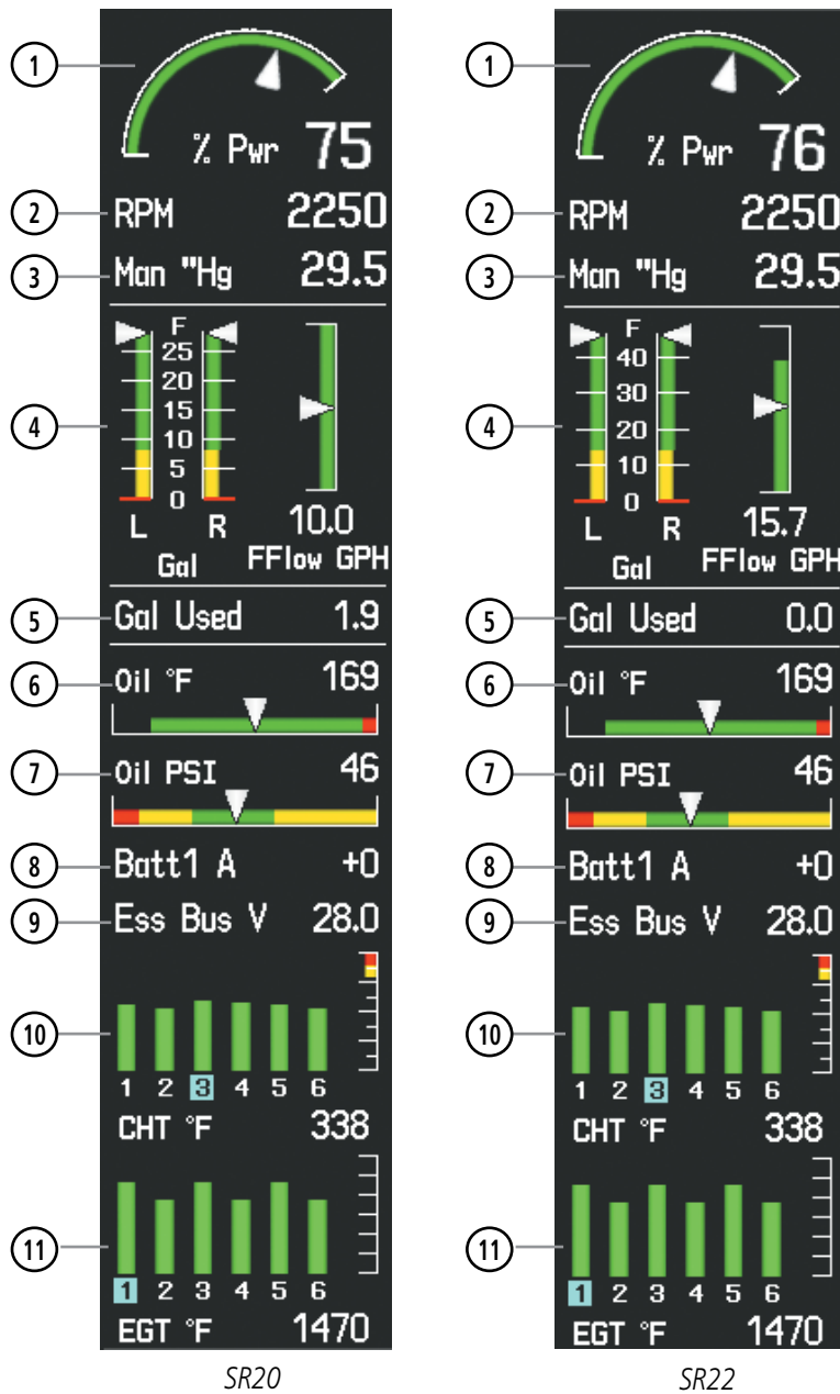
Figure 3-2 EIS Display (Naturally Aspirated)
