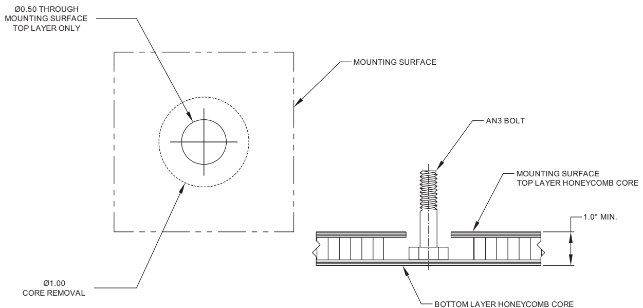
Figure 1-13 Mounting Bolt Preparation (Composite Aircraft)
