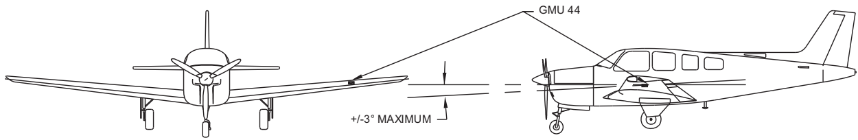
Figure 1-34 Level Mounting of GMU 44(B) Magnetometer
