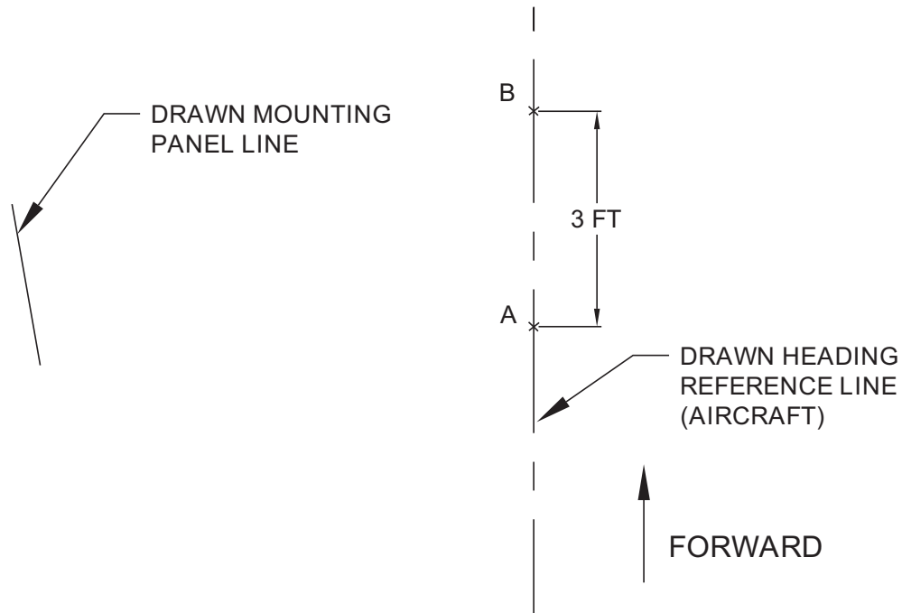
Figure 1-71 3-4-5 Triangle Method Step 1
