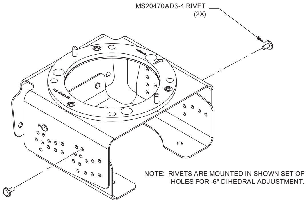
Figure 1-53 GMU 44 Universal Mount Incline Offset Procedure
