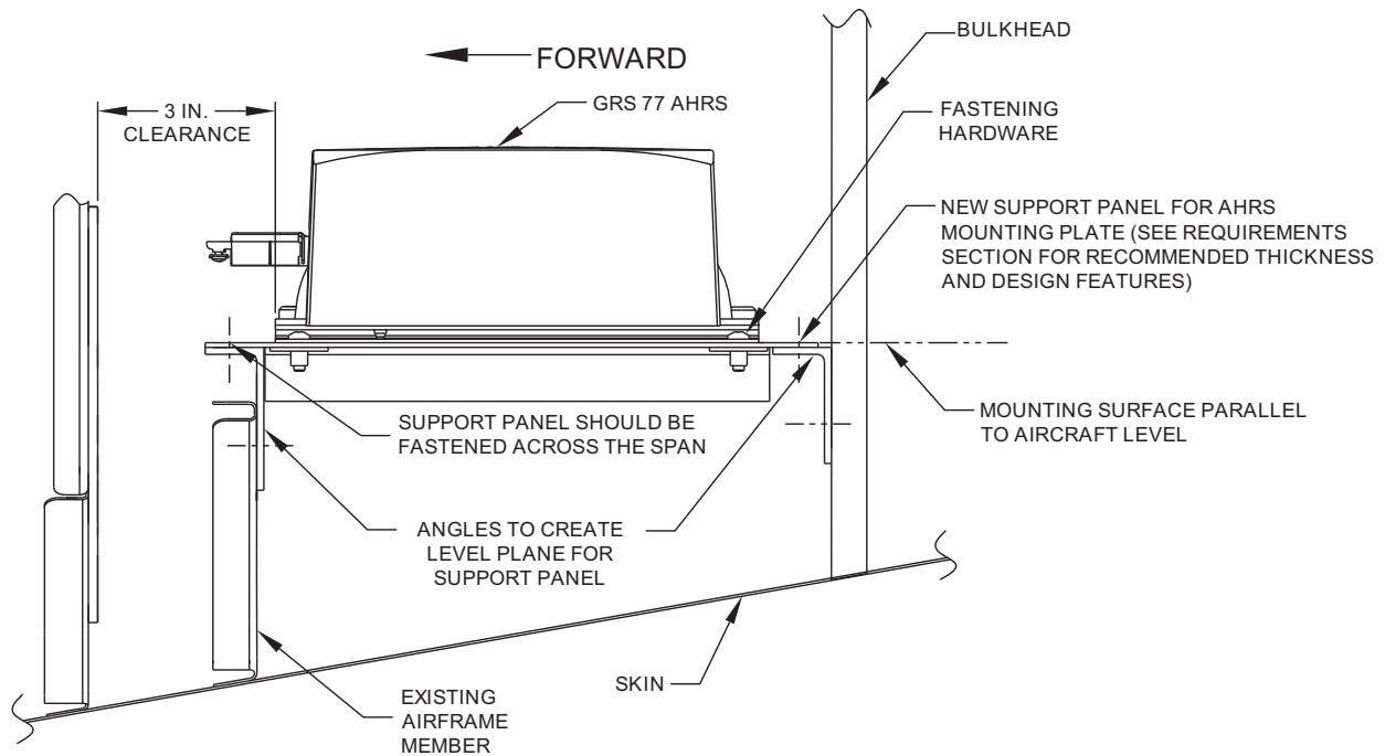
Figure 1-30 Installation of GRS 77 with Installed Support Plate
