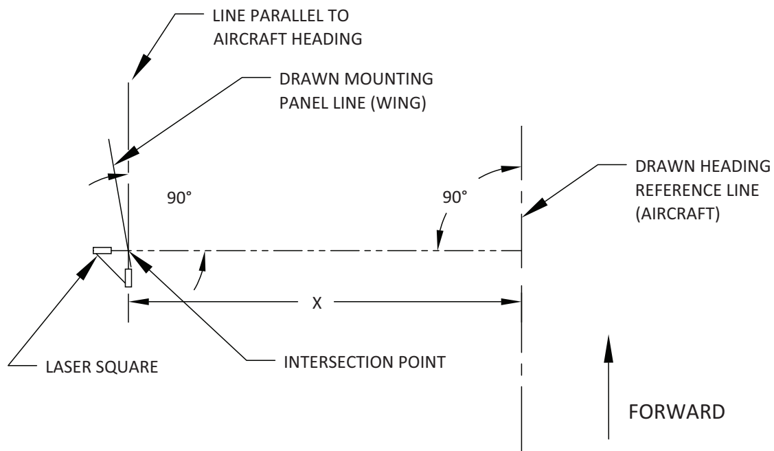
Figure 1-69 Transferring Center Line Step 2 (Laser Square Method)
