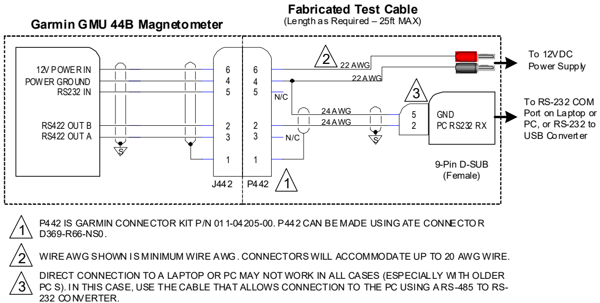
Figure 2-3 GMU 44B Magnetic Interference Survey Setup using R-485 to RS-232 Converter
