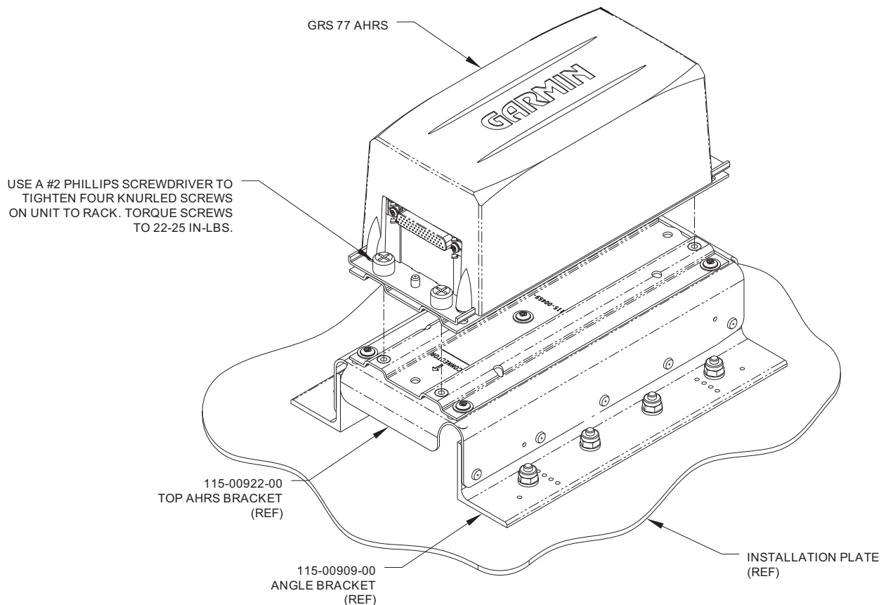
Figure 1-32 Final Installation Example
