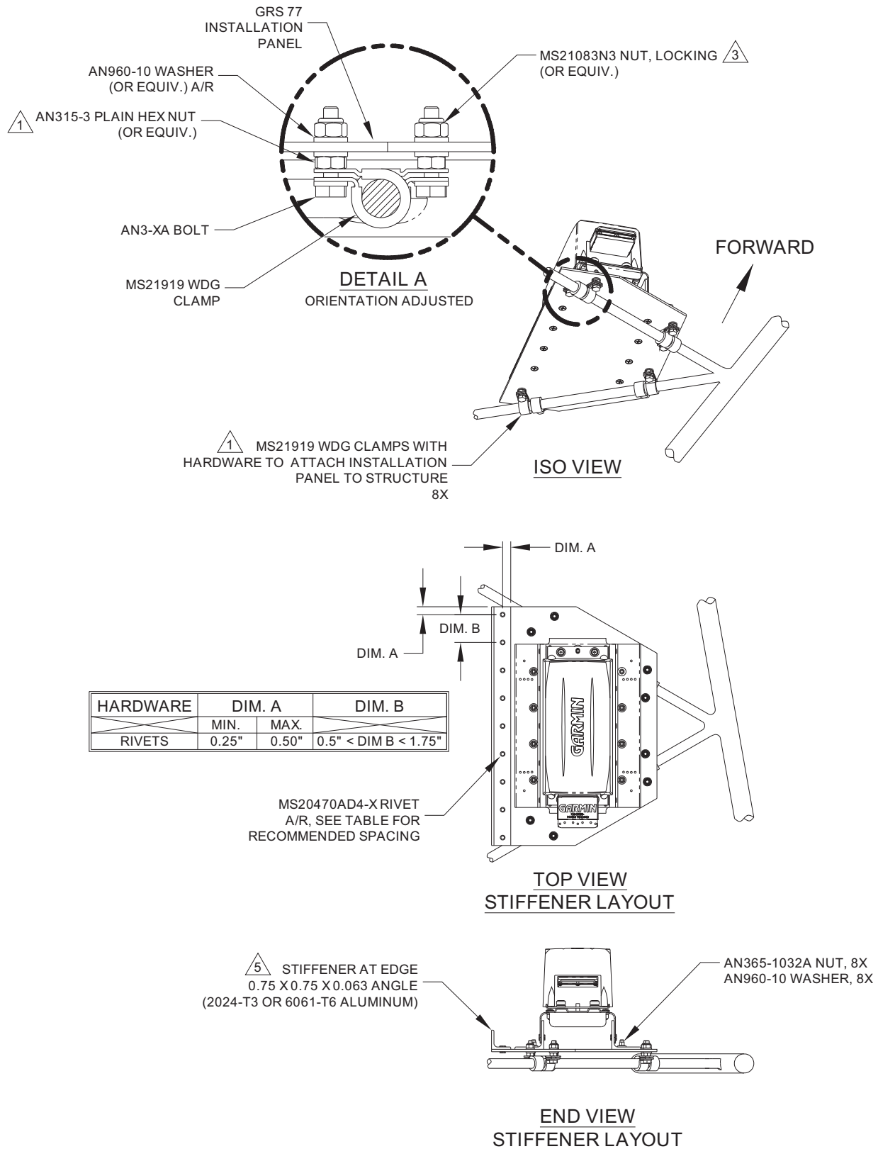
Figure 1-20 Installation of GRS 77 AHRS Universal Mount in Tube and Fabric Aircraft Using MS21919 Clamps
