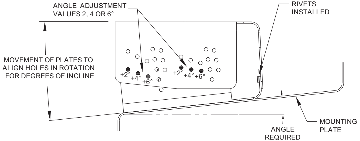
Figure 1-50 GMU 44 Universal Mount Hole Alignment, Rotational Method (Bottom Plate Mounted)
