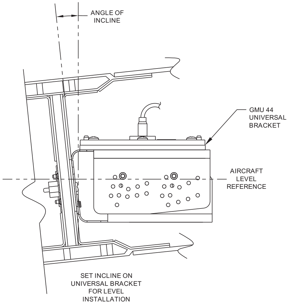
Figure 1-41 GMU 44 Universal Mount Level Installation Axis 2
