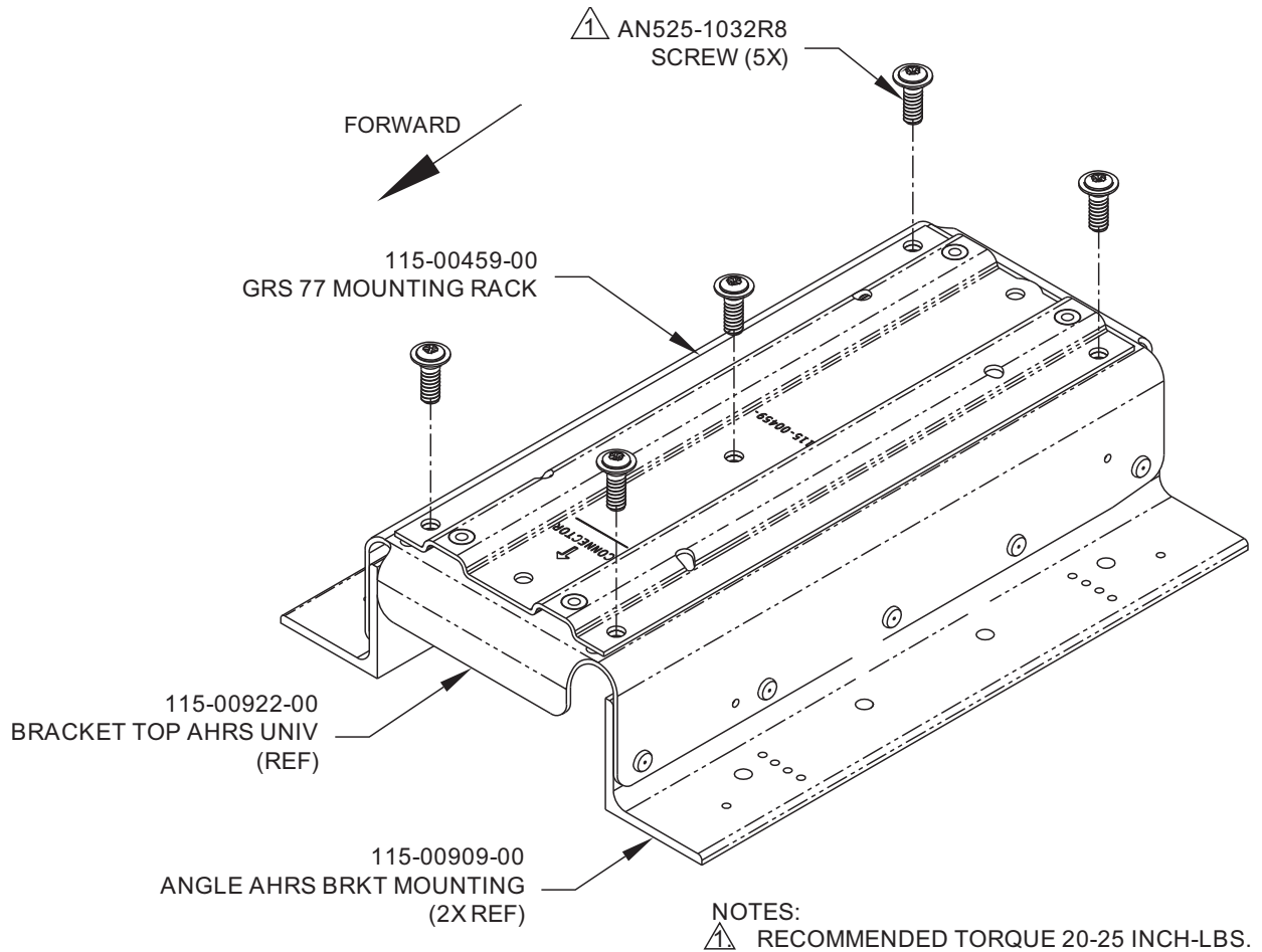
Figure 1-8 Assembling GRS 77 Mounting Rack to GRS 77 Universal Mount
