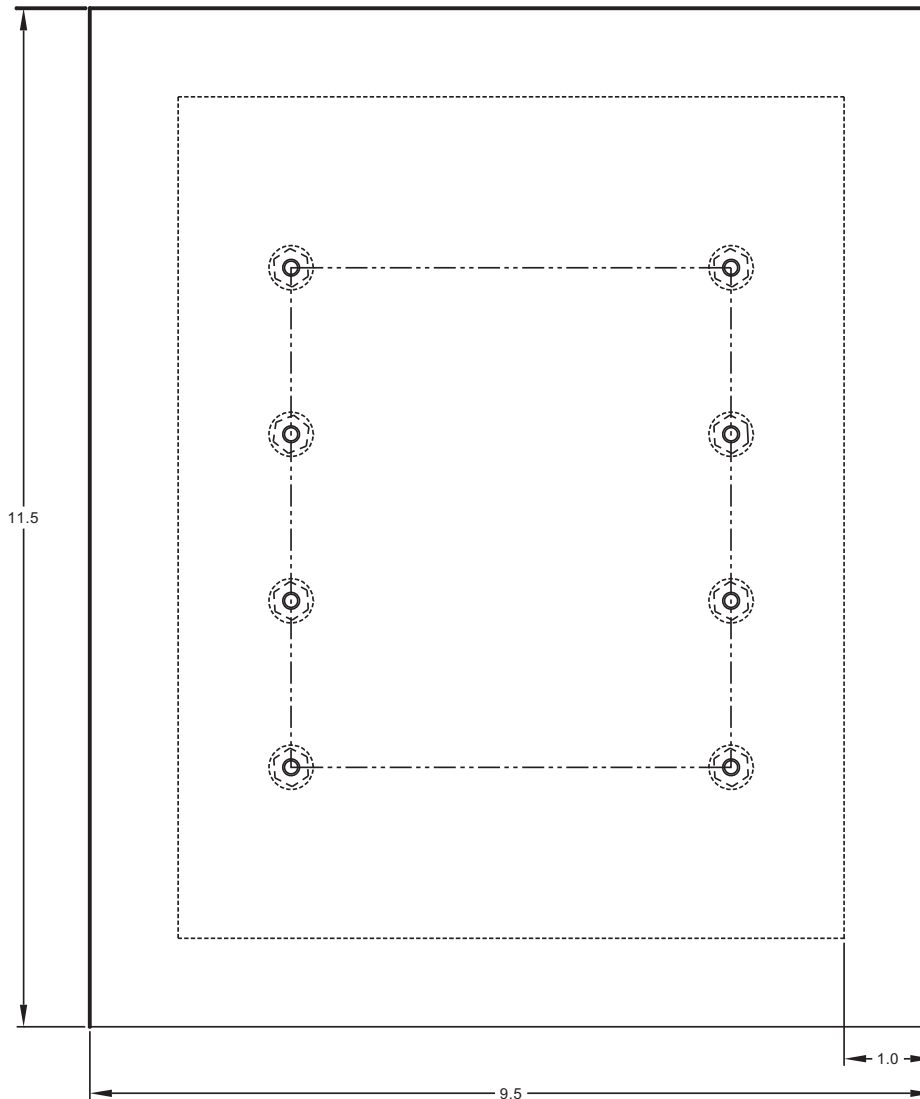
Figure 1-16 Second Cloth Installation for Mounting Bolts (Composite Aircraft)
