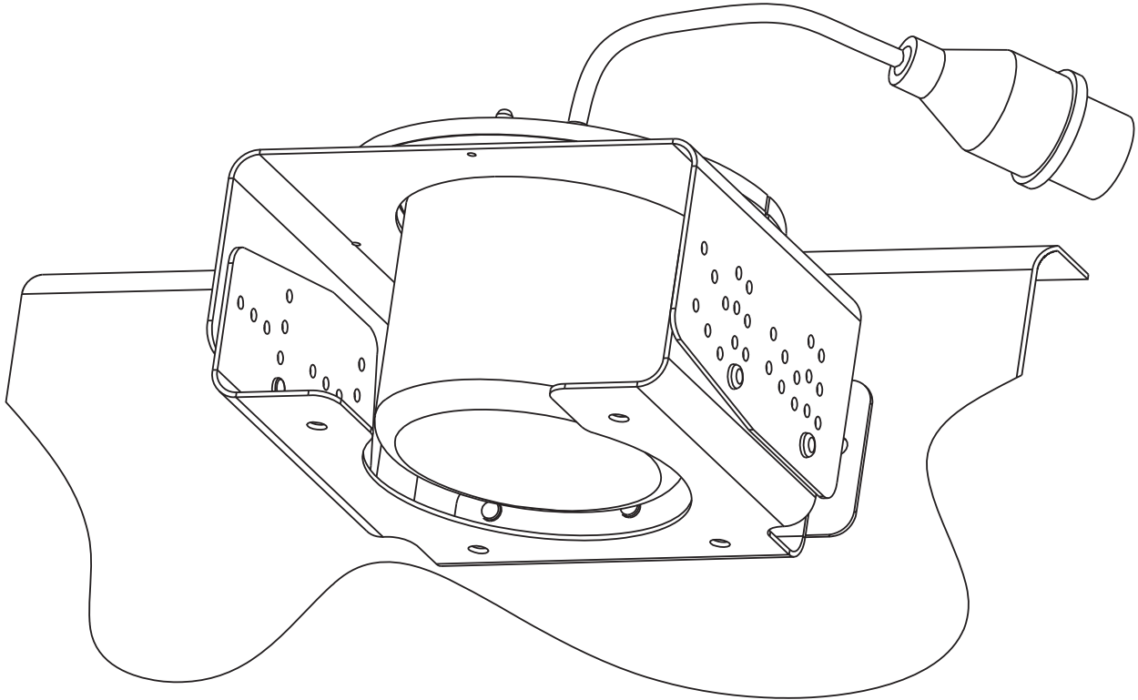
Figure 1-36 GMU 44 Universal Mount, Side Plate Mounted
