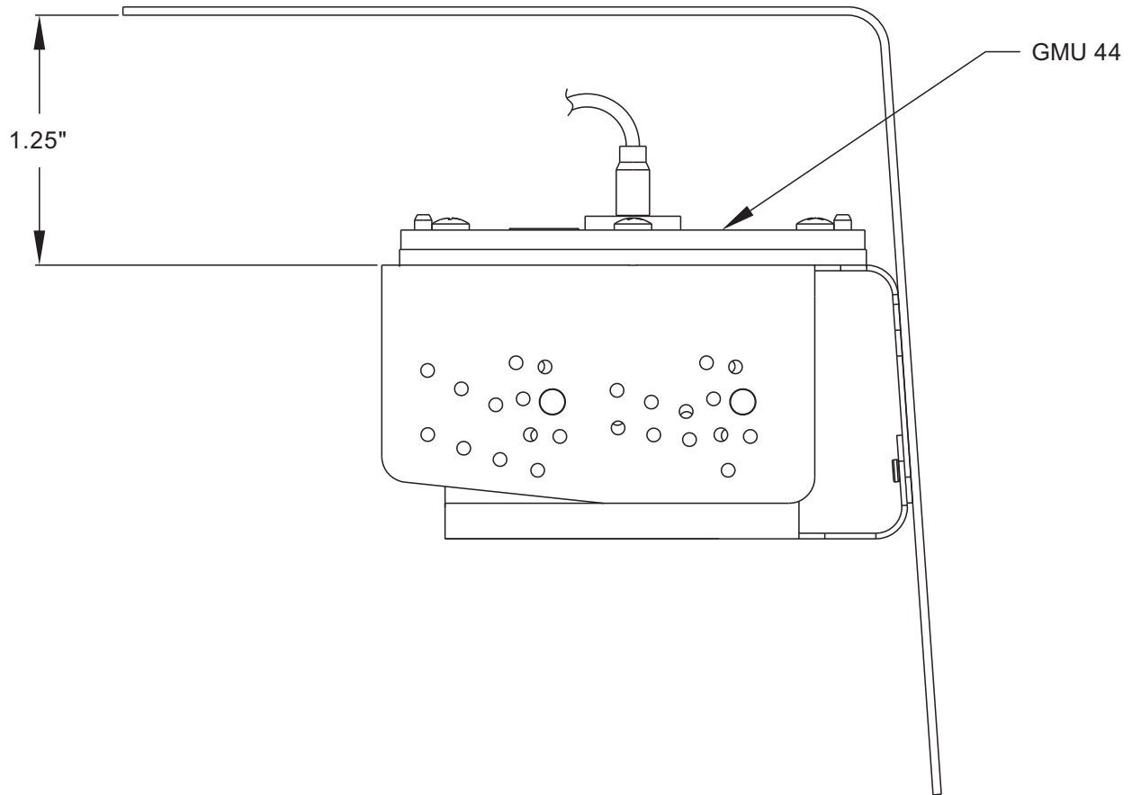
Figure 1-57 GMU 44(B) Installation Clearance
