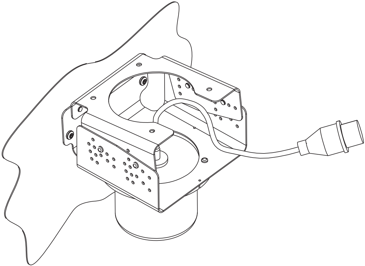
Figure 1-38 GMU 44 Universal Mount, Side Plate - Suspended
