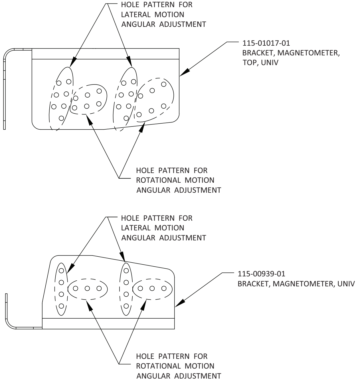
Figure 1-47 GMU 44 Universal Mount Top and Bottom Hole-Patterns
