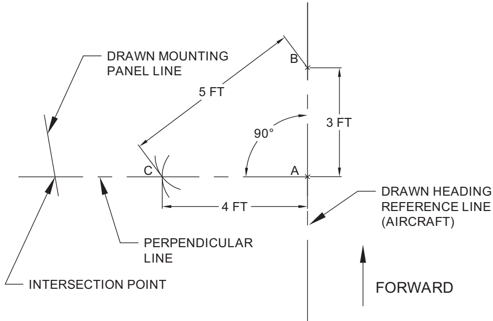
Figure 1-73 3-4-5 Triangle Method Step 3
