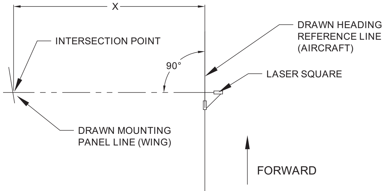
Figure 1-68 Transferring Center Line Step 1 (Laser Square Method)
