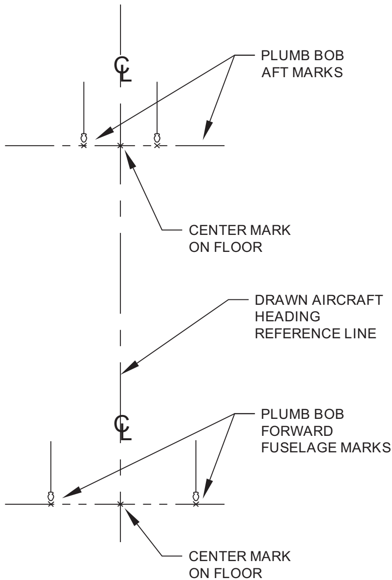
Figure 1-67 Center Line (Plumb Bob Method)
