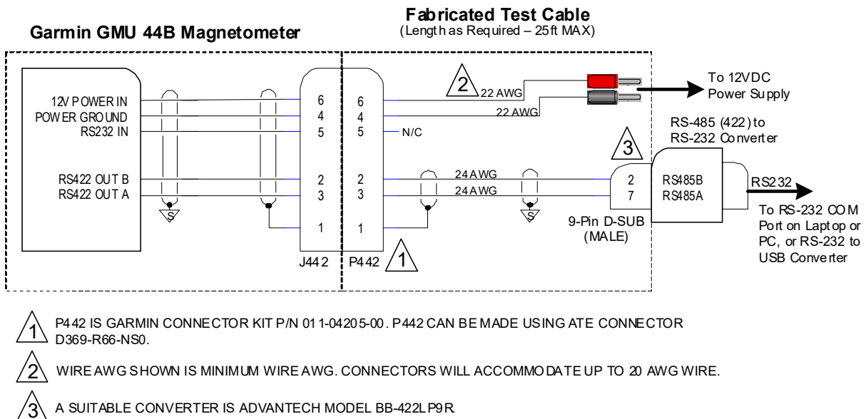
Figure 2-4 GMU 44B Magnetic Interference Survey Setup using R-485 to RS-232 Converter
