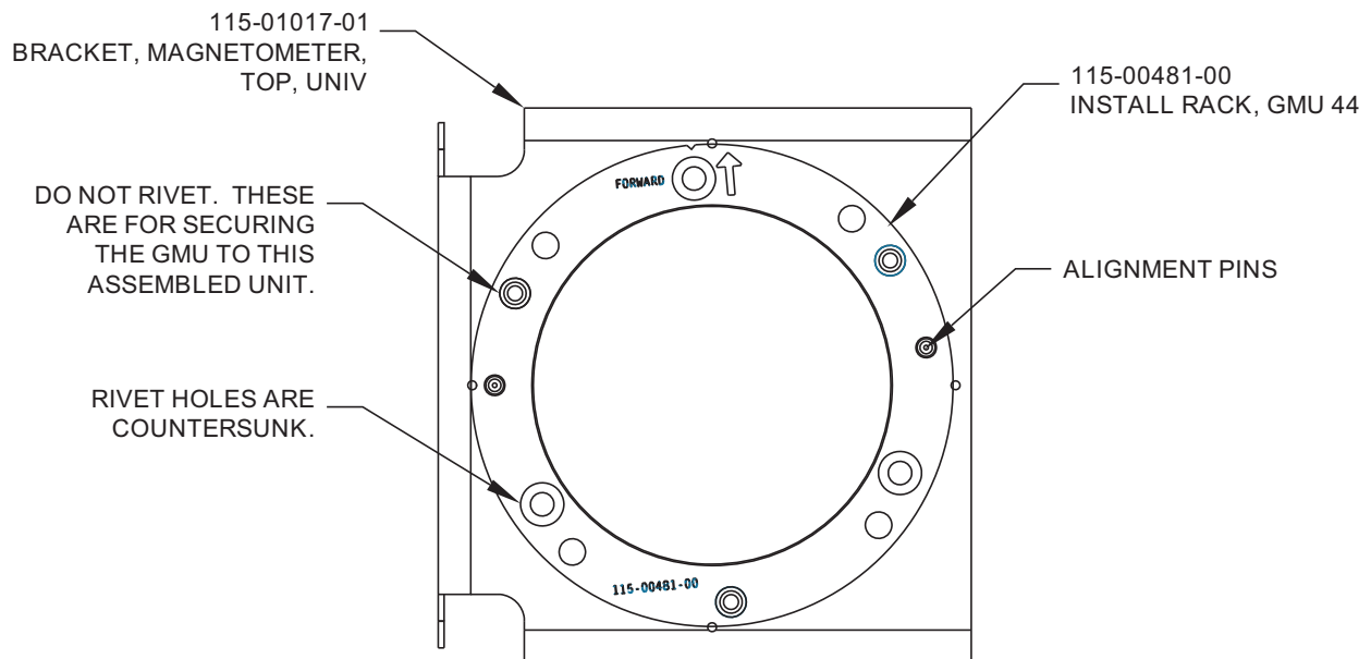
Figure 1-44 Installation Rack Rivet Through Holes
