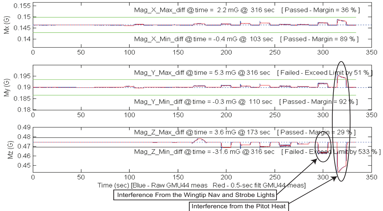
Figure 2-5 Interference From The Wingtip Nav And Strobe Lights Interference From The Pitot Heat
