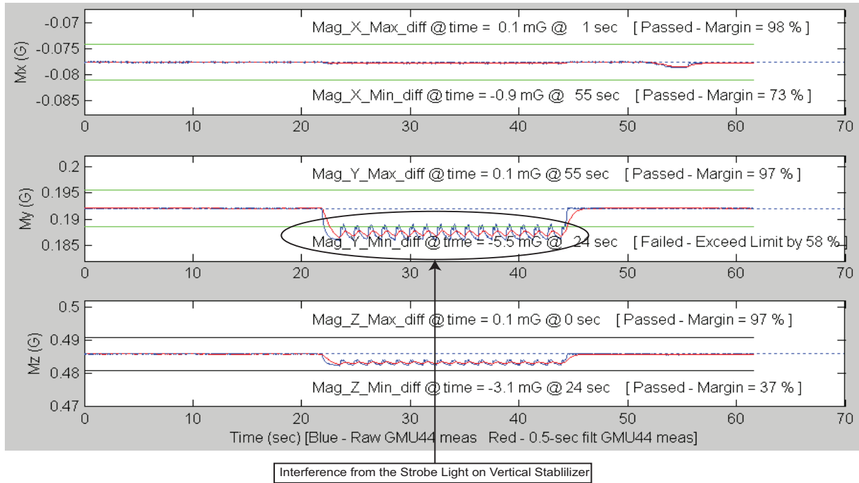
Figure 2-6 Interference From The Strobe Light On Vertical Stabilizer
