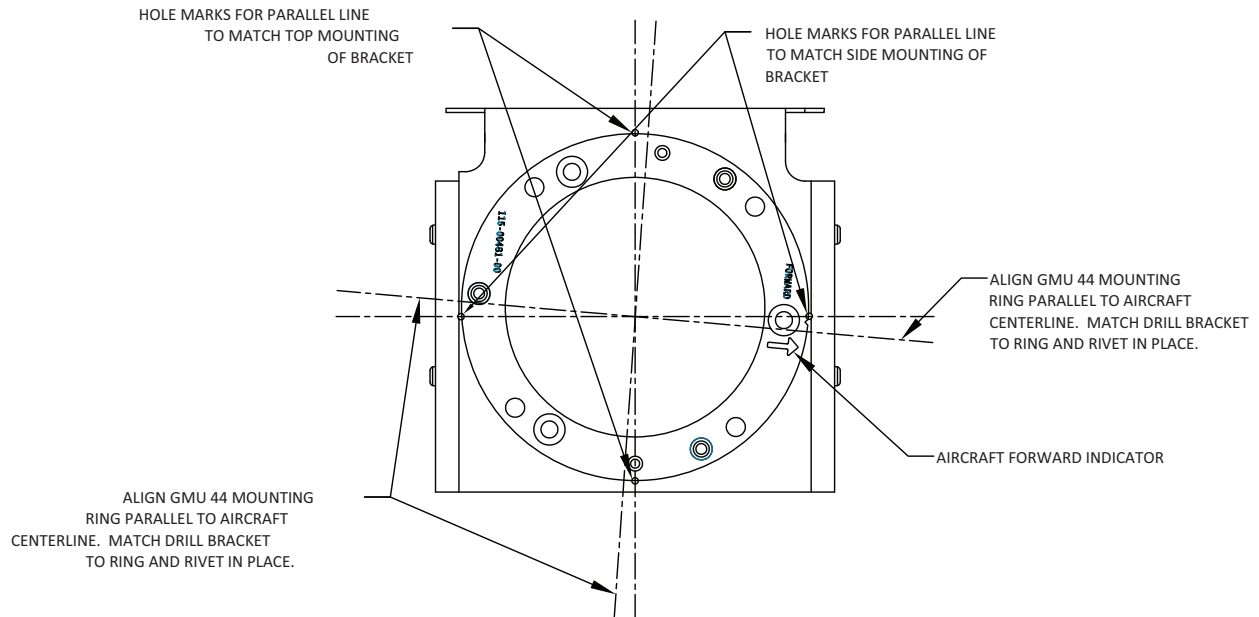
Figure 1-43 Top Plate Alignment to Aircraft Heading
