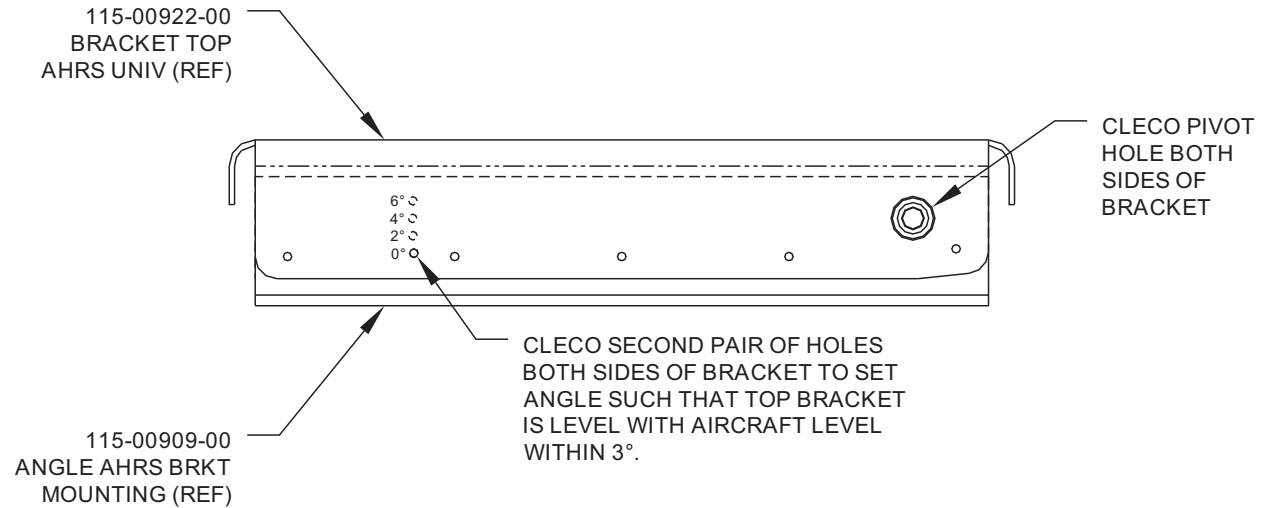
Figure 1-5 GRS 77 Universal Mount Assembly
