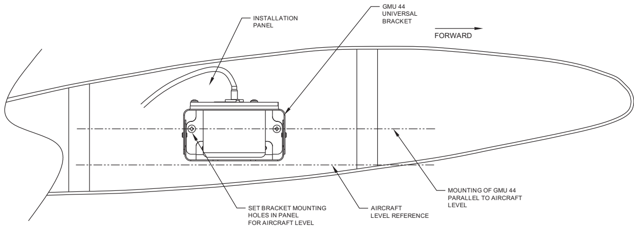
Figure 1-40 GMU 44 Universal Mount Level Installation Axis 1
