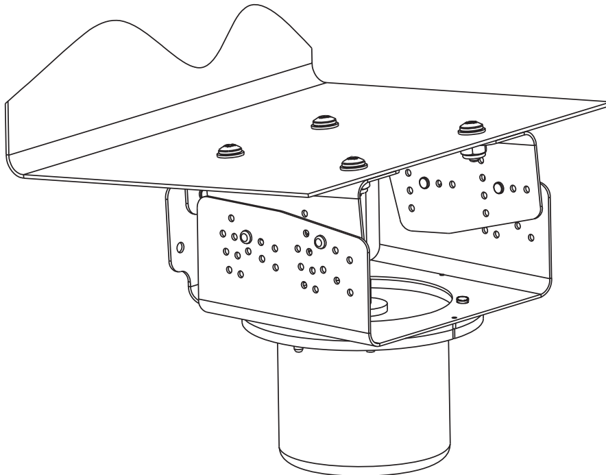
Figure 1-39 GMU 44 Universal Mount, Bottom Plate Mounted - Suspended
