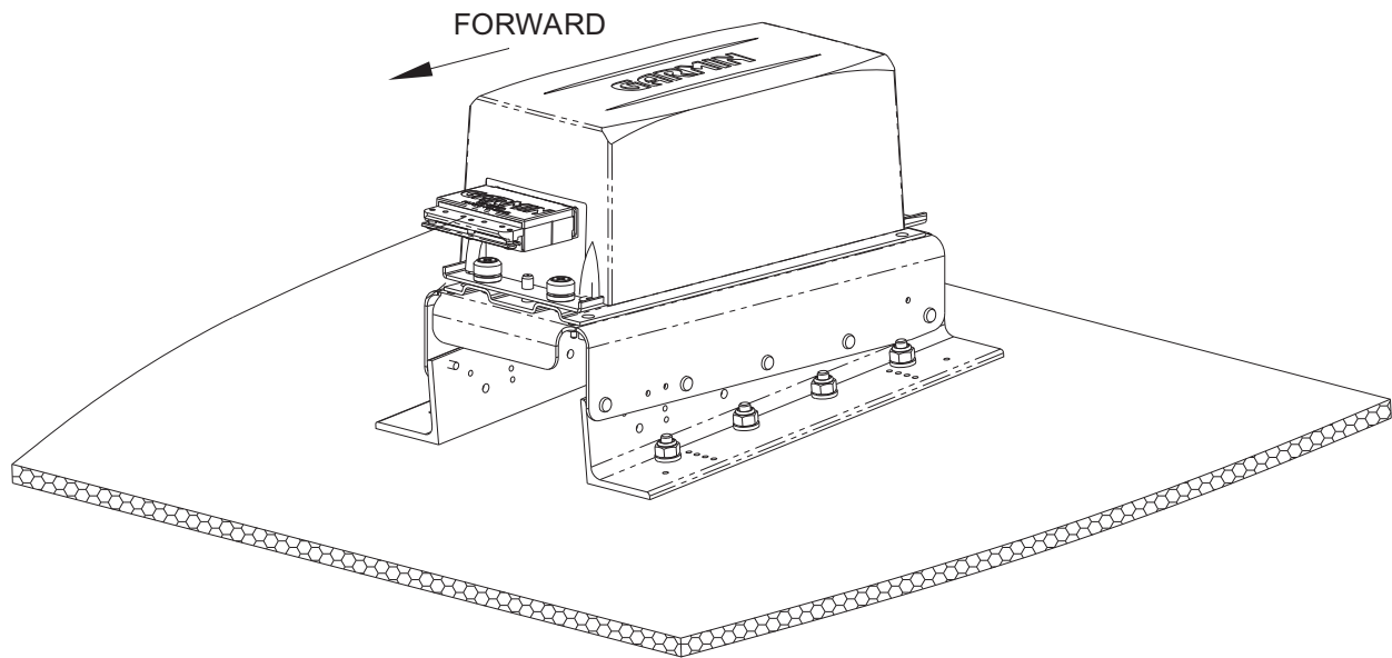
Figure 1-11 Universal Mount (Composite Aircraft)
