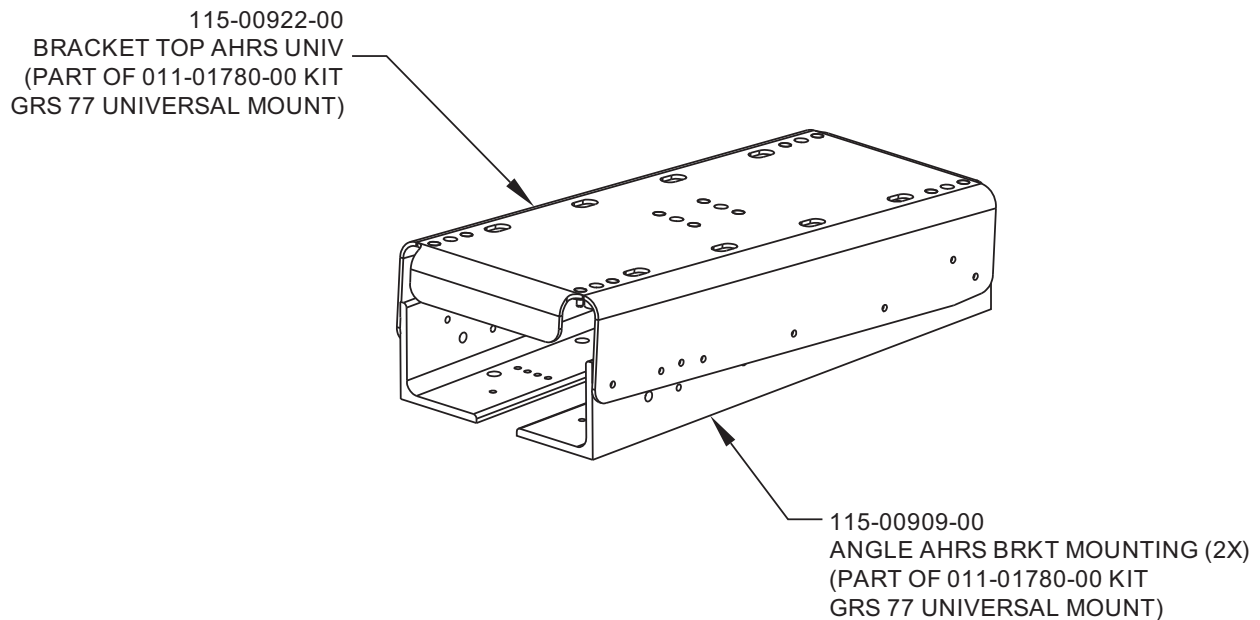
Figure 1-3 GRS 77 Universal Mount (Inward Facing Angle Brackets)
