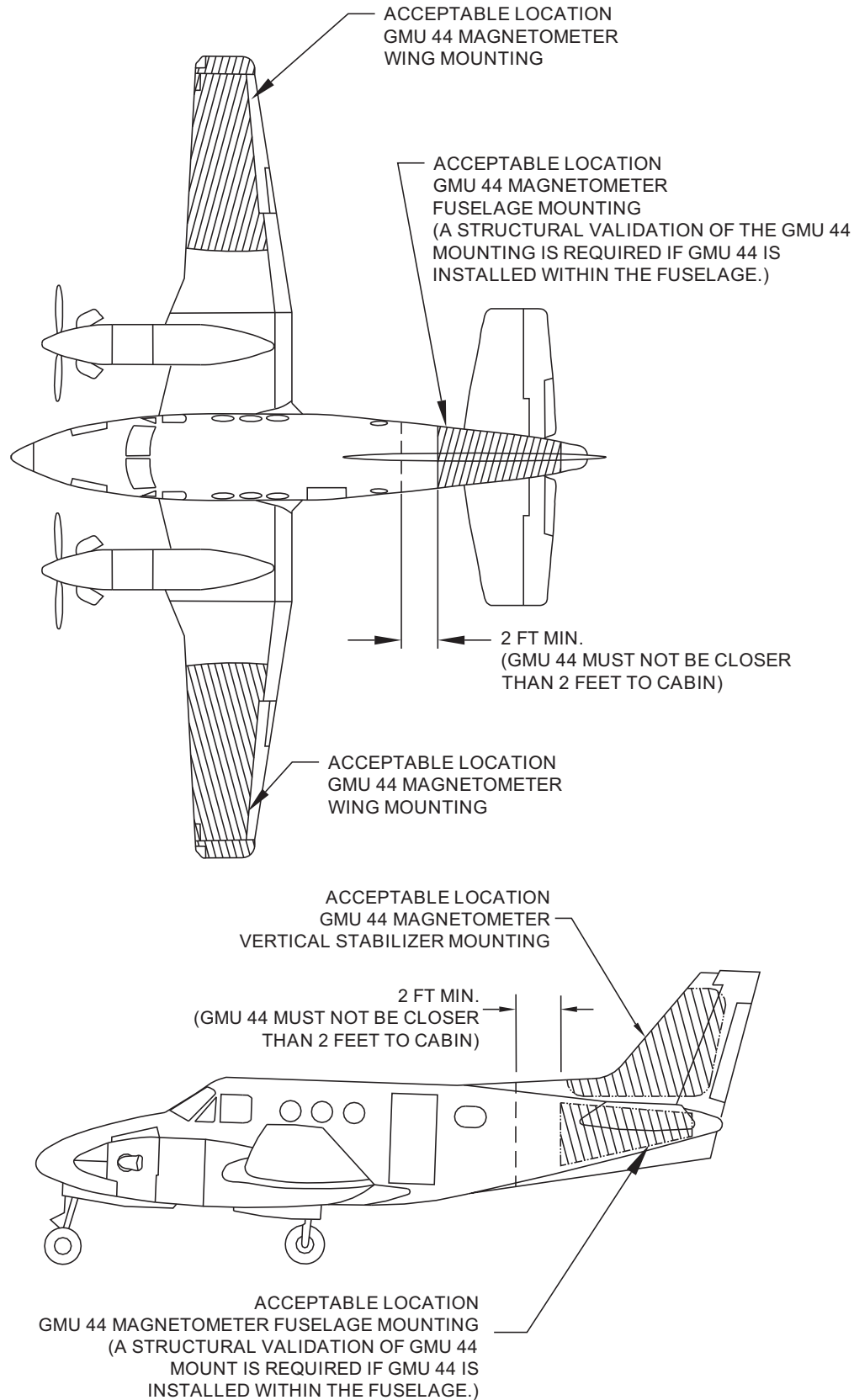
Figure 1-33 GMU 44(B) Mounting Locations
