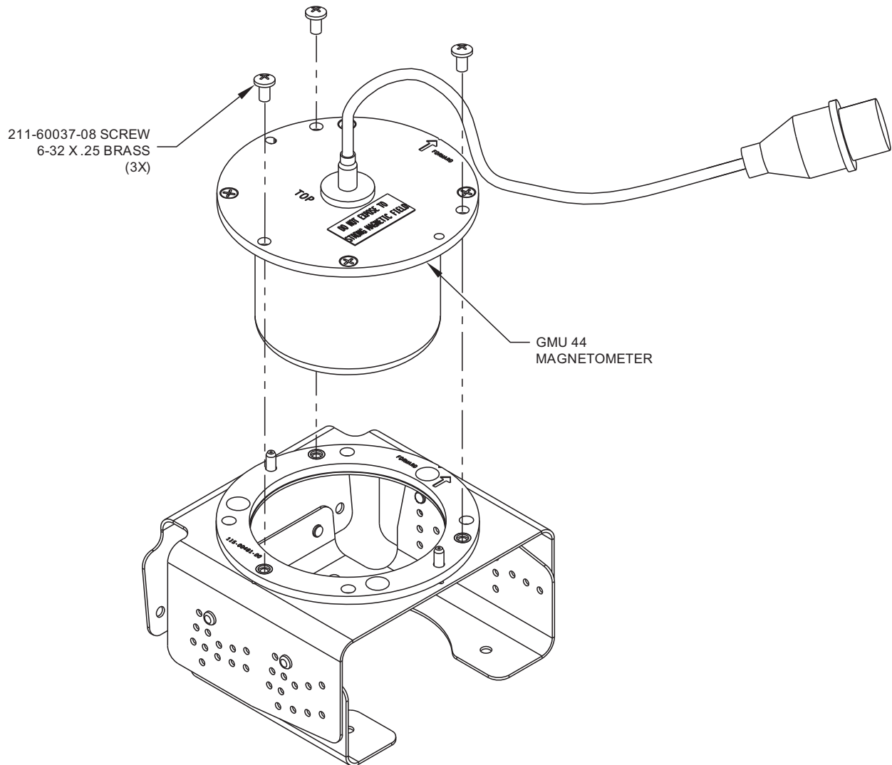
Figure 1-56 Installation of the GMU 44(B) into the GMU 44 Universal Mount
