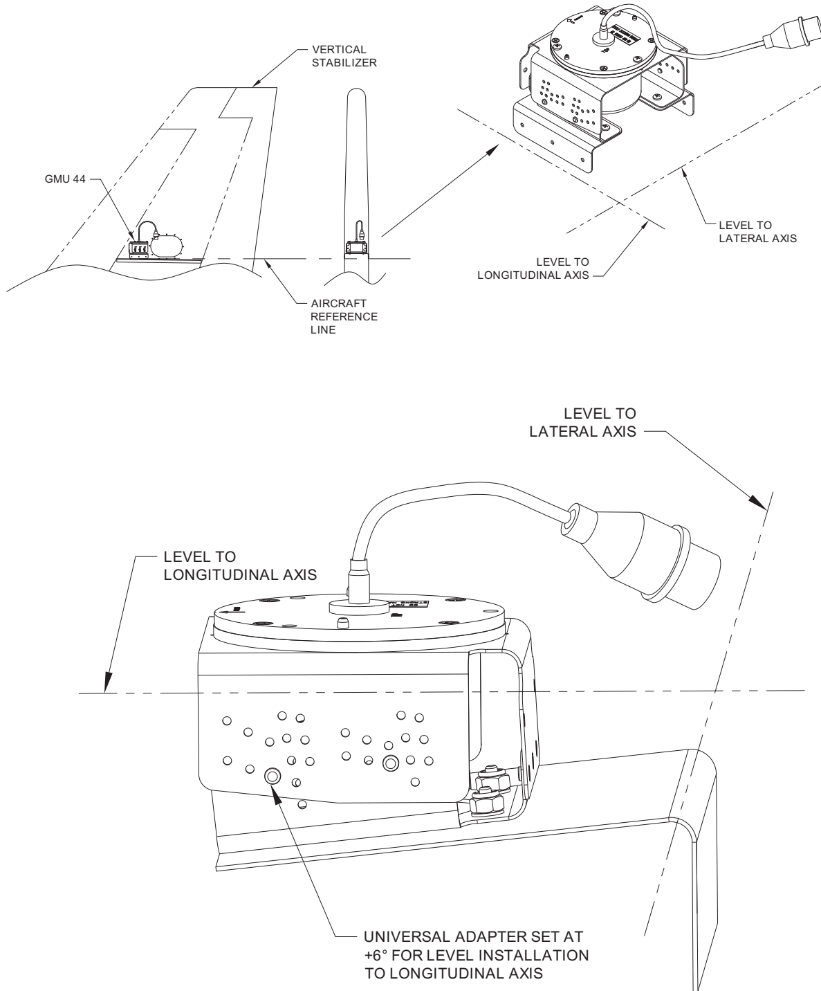
Figure 1-42 GMU 44 Universal Mount Level Installation Using Support Equipment
