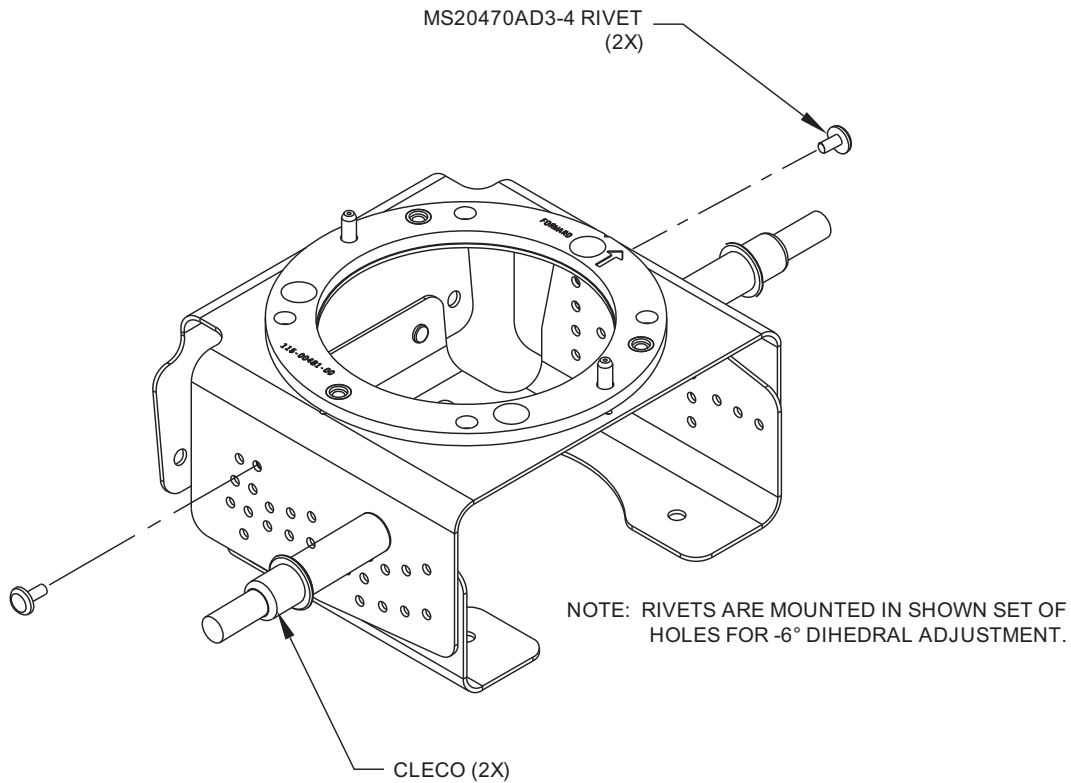
Figure 1-52 GMU 44 Universal Mount Incline Offset Procedure
