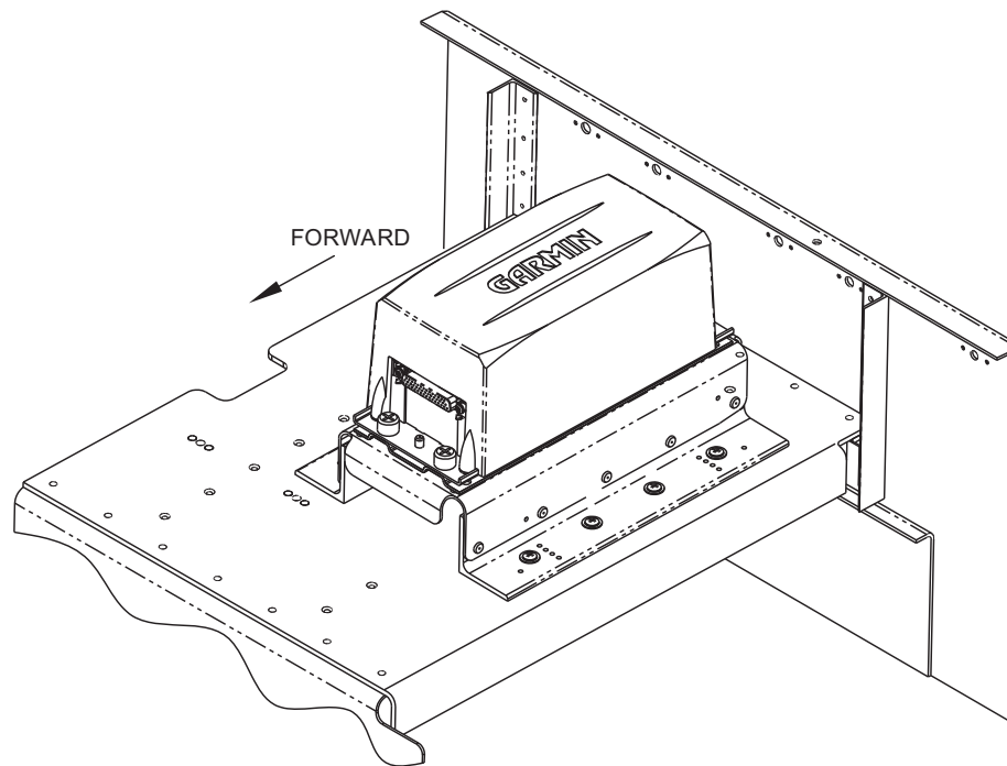
Figure 1-9 GRS 77 Universal Mount (Typical)
