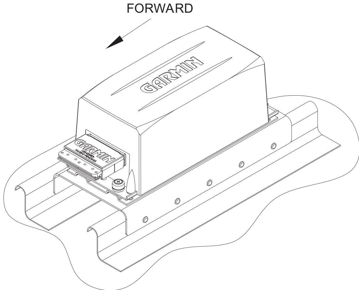
Figure 1-24 Mounting Bracket Attachment to Stringers or Longerons
