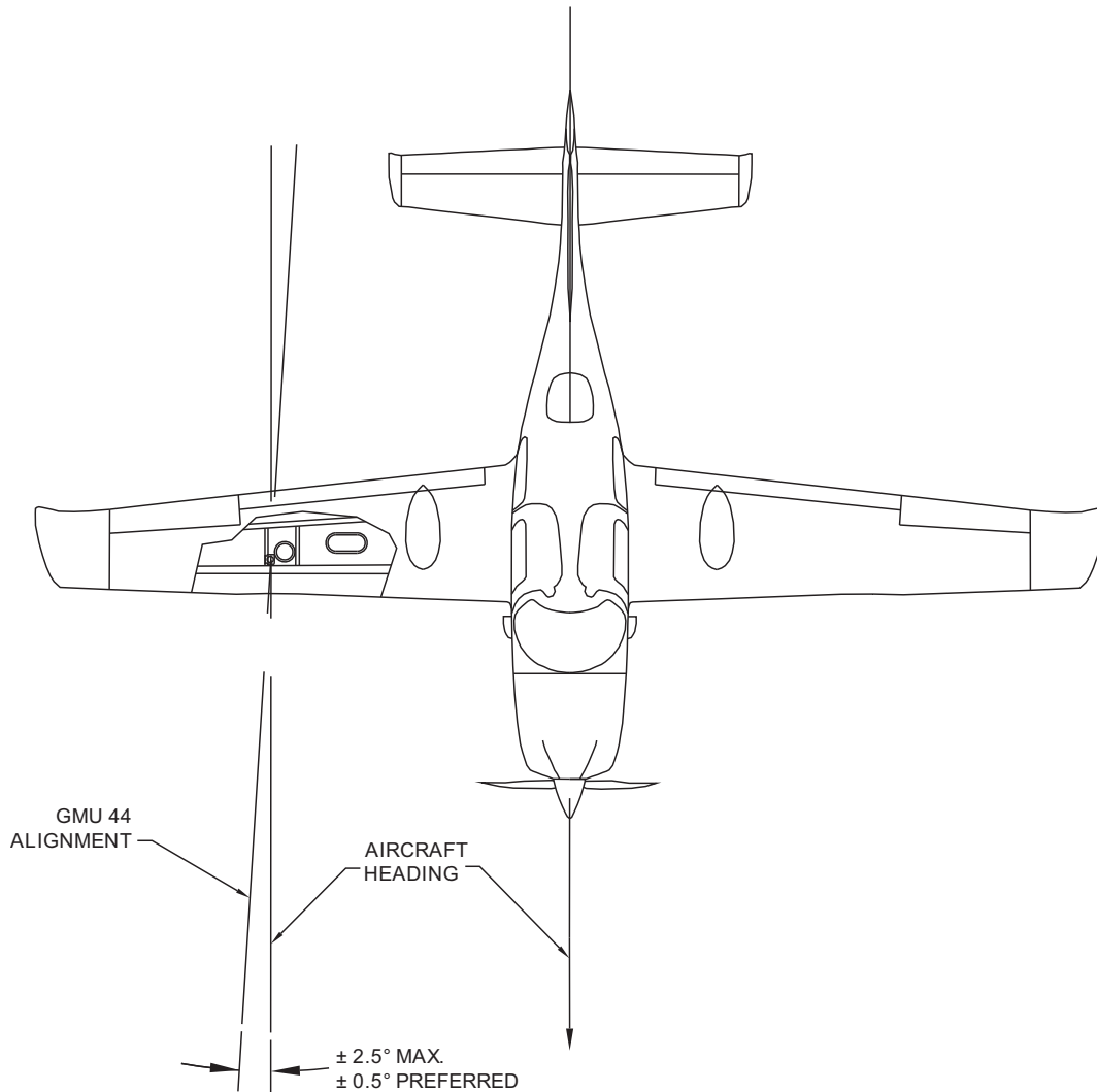
Figure 1-35 Heading Offset Limit GMU 44(B) Magnetometer
