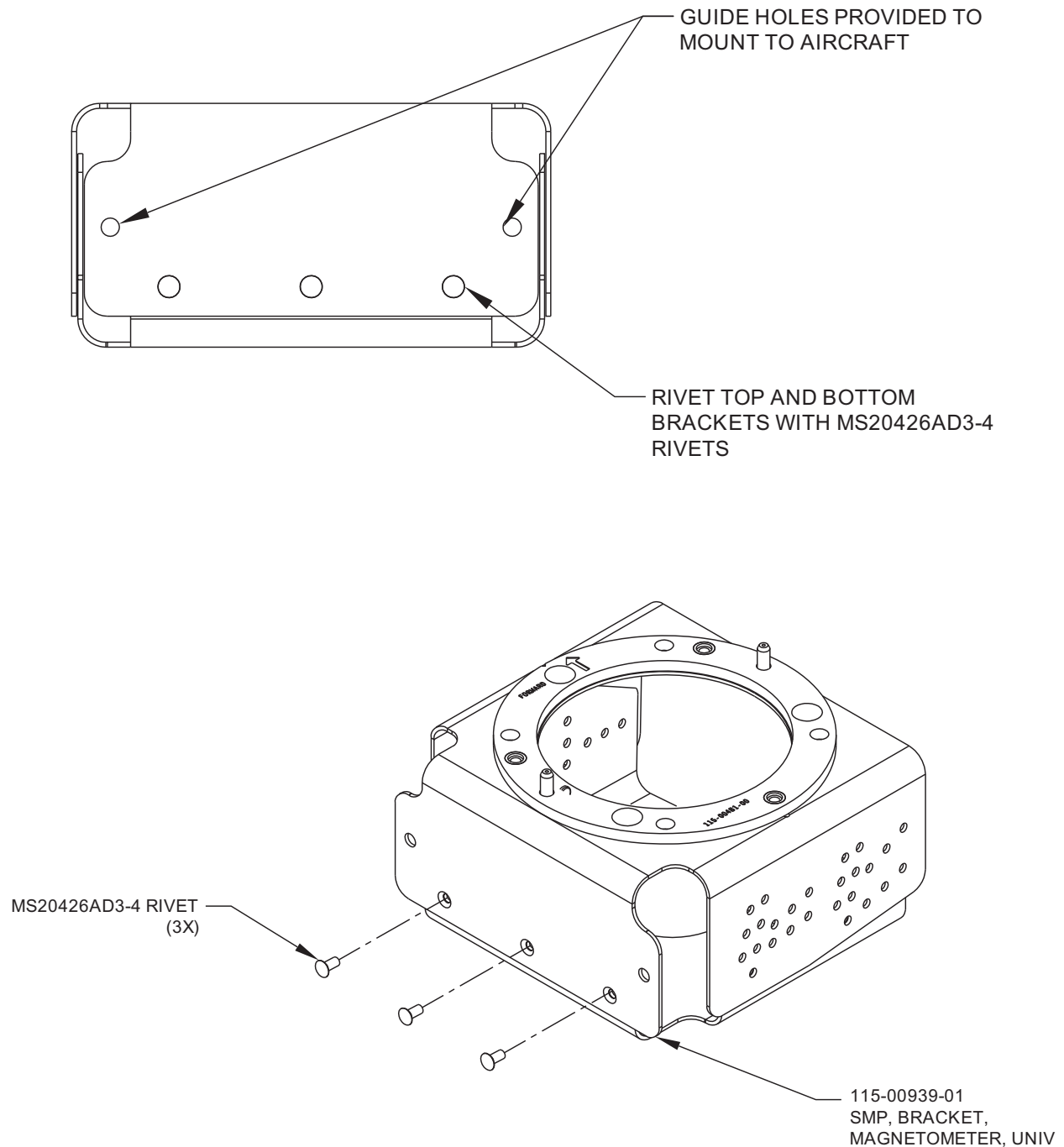
Figure 1-46 GMU 44 Universal Mount Top and Bottom Bracket Assembly
