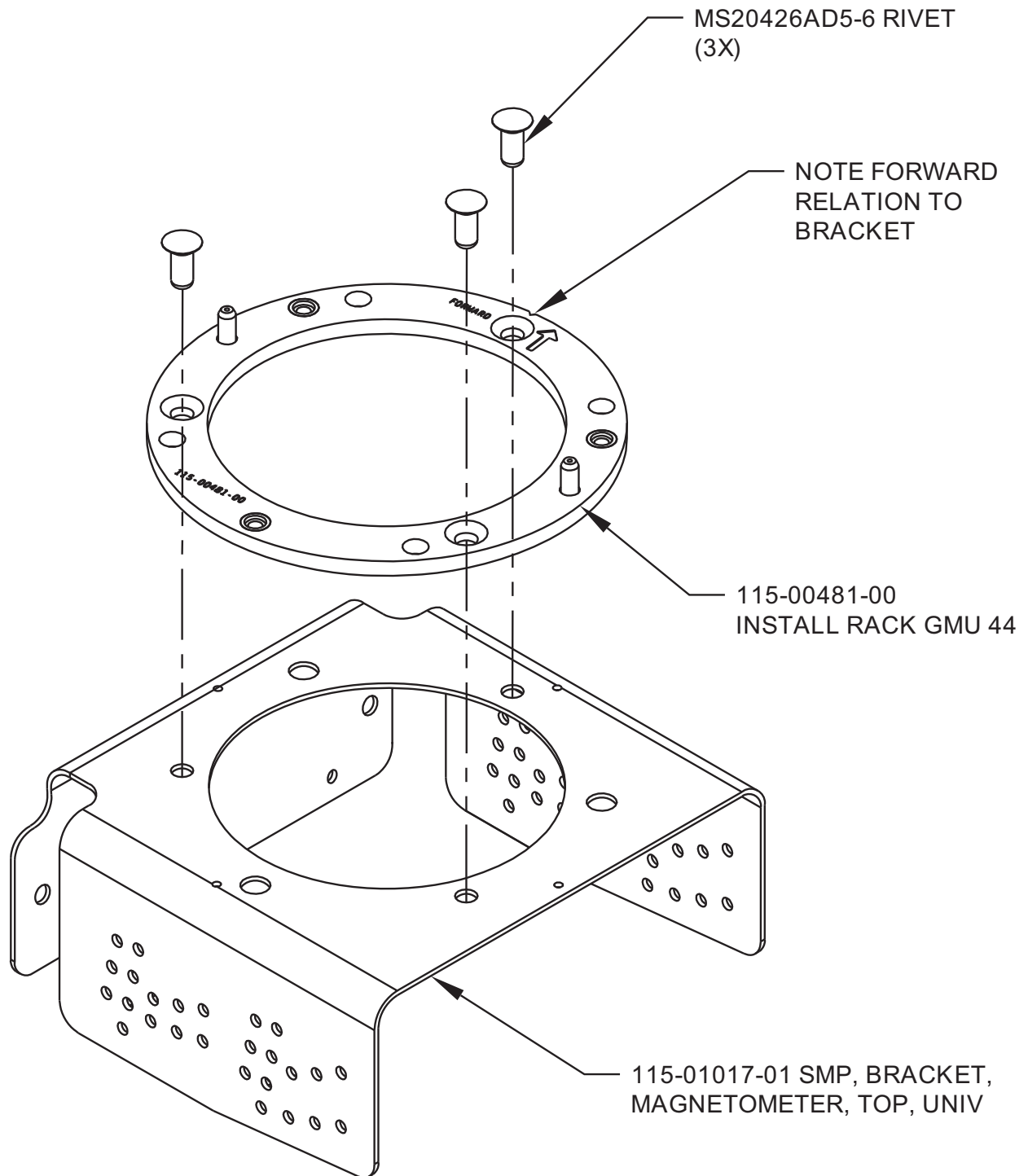
Figure 1-45 Installation Rack to Top Bracket Installation
