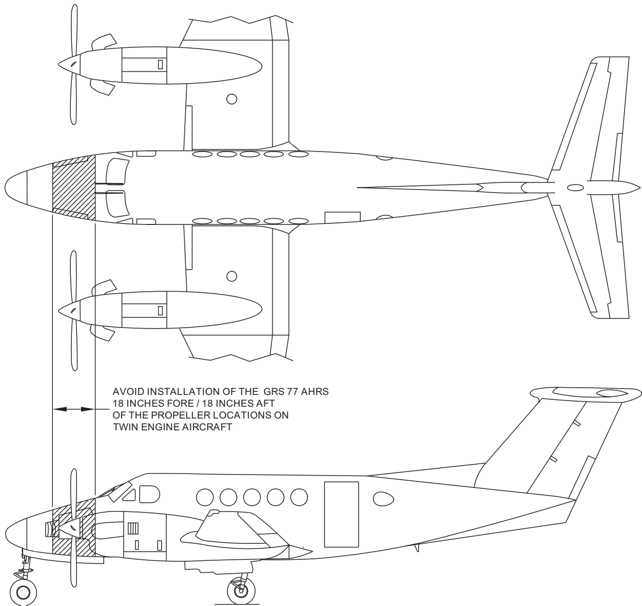
Figure 1-2 Acceptable Locations for the AHRS
