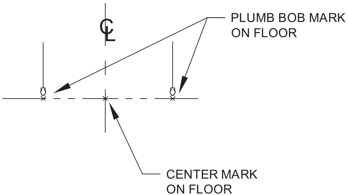
Figure 1-65 Center Mark for the Forward Fuselage (Plumb Bob Method)
