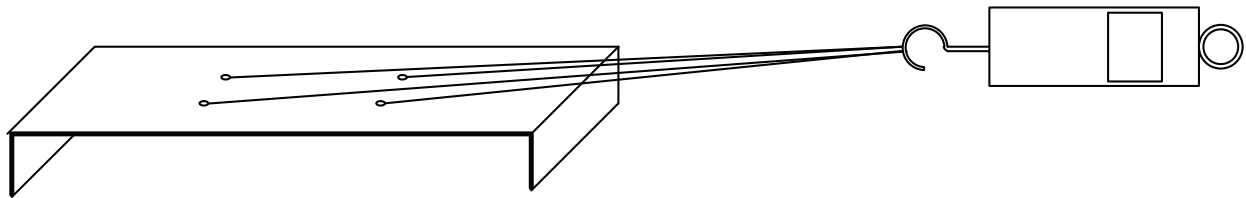
Figure 1-76 Forward Static Load Test
