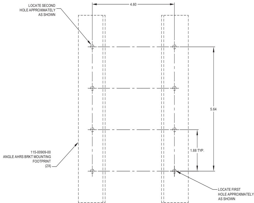
Figure 1-12 Mounting Location (Composite Aircraft)
