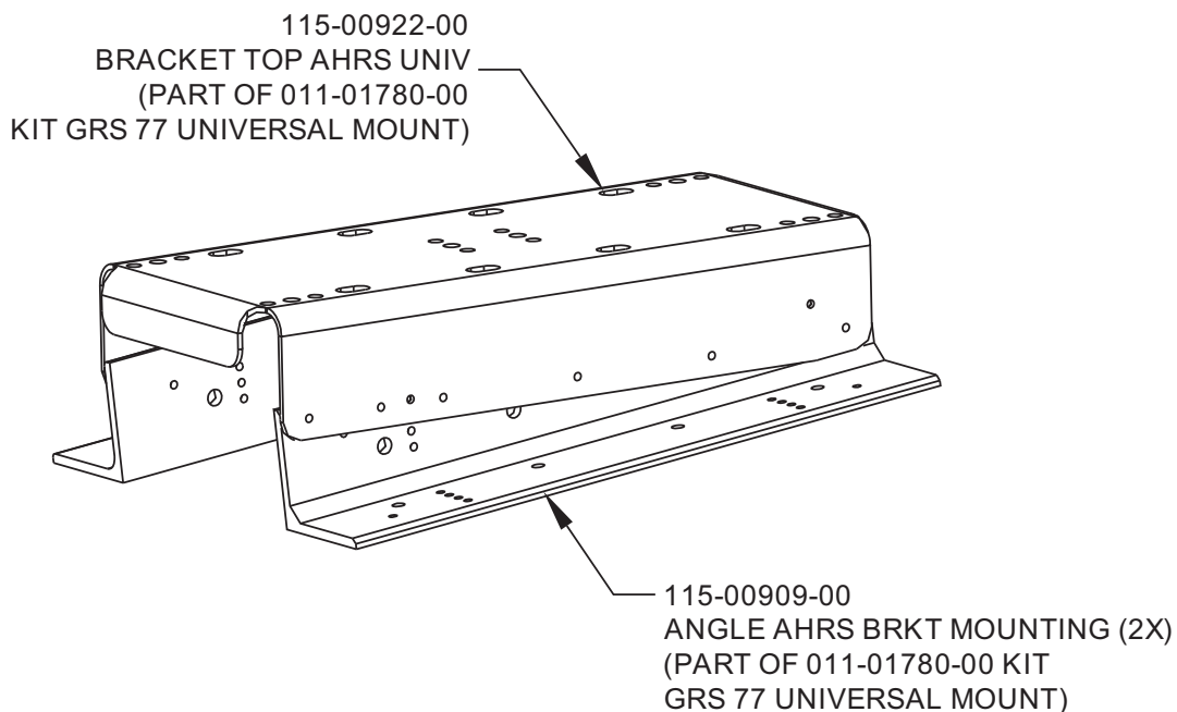
Figure 1-4 GRS 77 Universal Mount (Outward Facing Angle Brackets)
