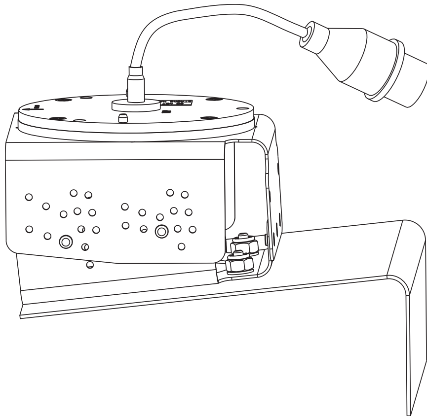
Figure 1-37 GMU 44 Universal Mount, Bottom Plate Mounted
