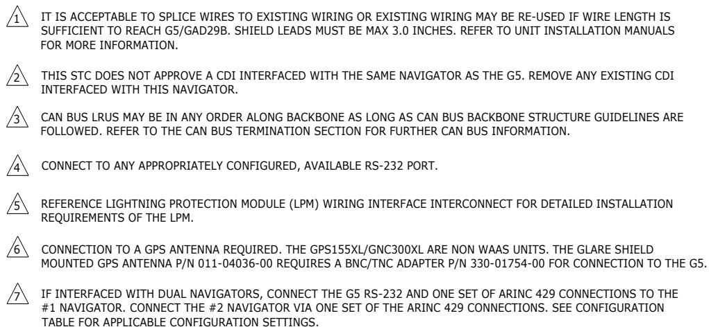
Figure 5-17 G5 (HSI) with GPS Navigator
