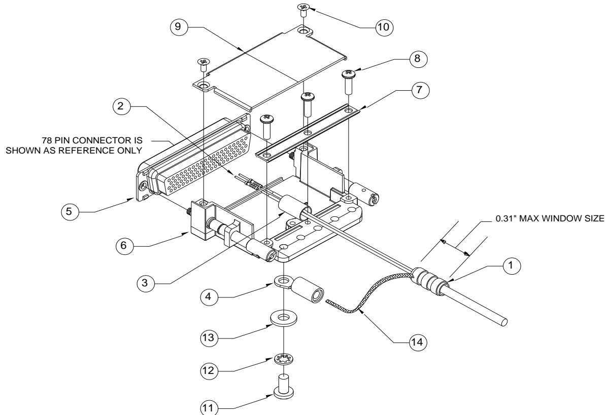
Figure 4-49 GAD29(B)(D), GAD13, GMU11 Wiring Harness Connector Assembly
