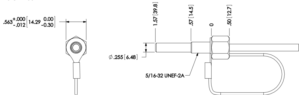
Figure 6-22 GTP 59 Outline Drawing
