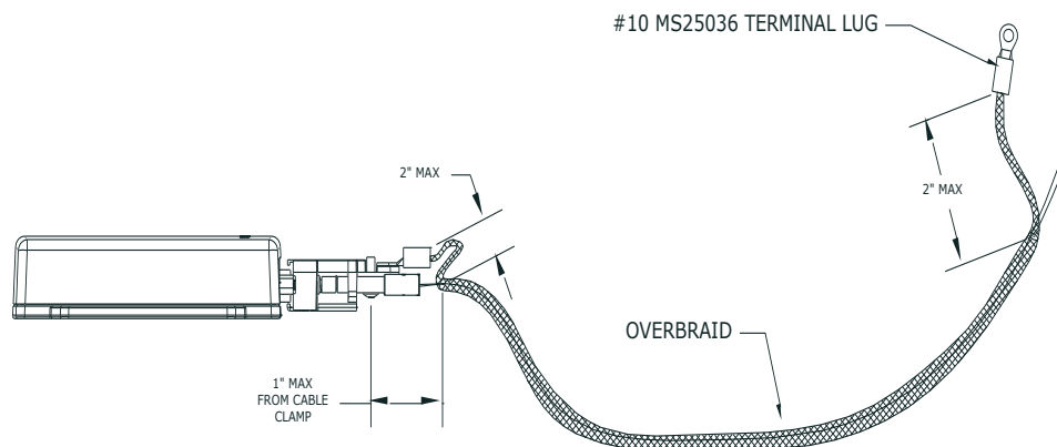
Figure 6-26 GMU 11 Overbraid Installation
