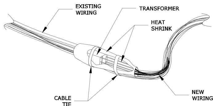
Figure 3-6 GAD 29B/29D Inline Transformer Mounting Instructions
