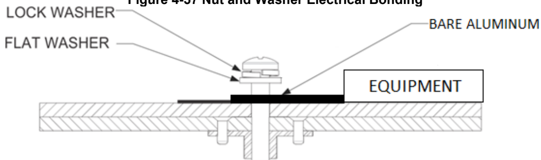
Figure 4-58 Nut Plate Electrical Bonding
