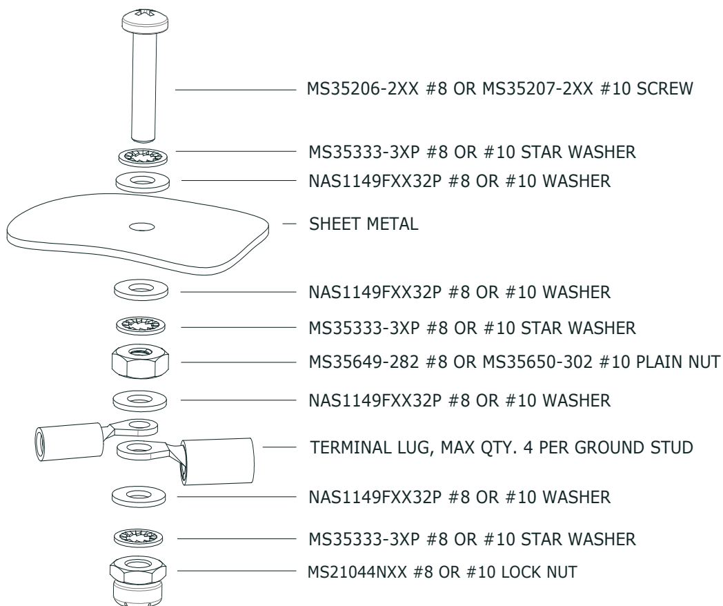
Figure 4-64 - Pan Head Screw Ground Stud Buildup
