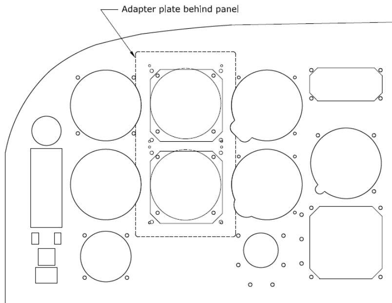
Figure 4-28 Adapter Plate Located on Far Side of Instrument Panel Use reference holes from adapter plate to align adapter plate behind panel.
