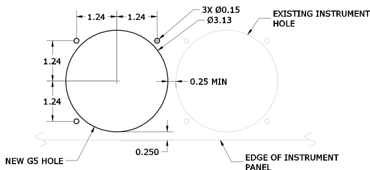
Figure 4-13 G5 Instrument Hole Dimensions
