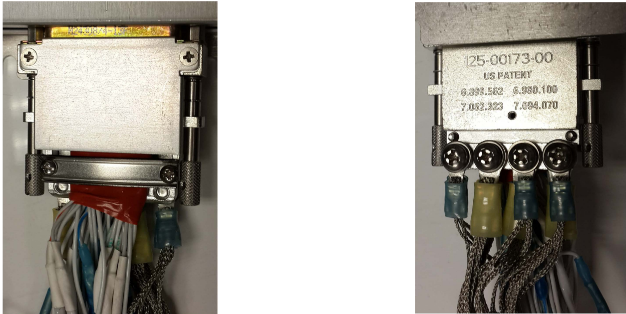
Figure 3-13 GMA 245R Audio Shield Termination (top and bottom)
