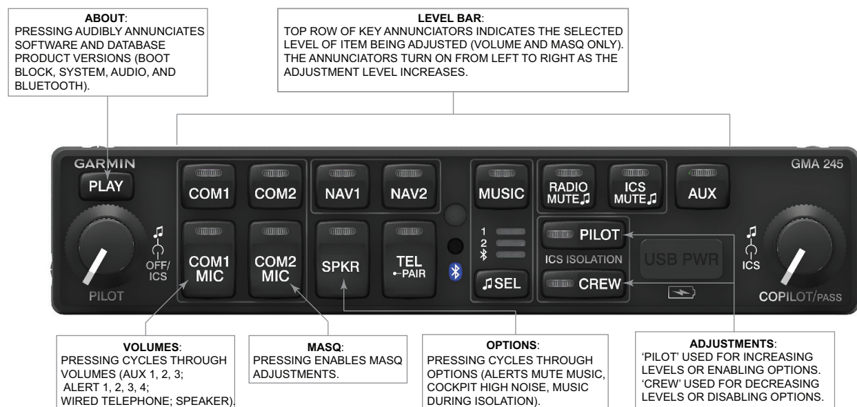
Figure 2-4 Front Panel Configuration
