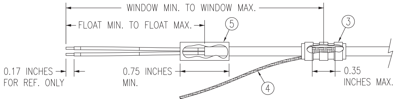
Figure 3-3 Method A.1 for Shield Termination
