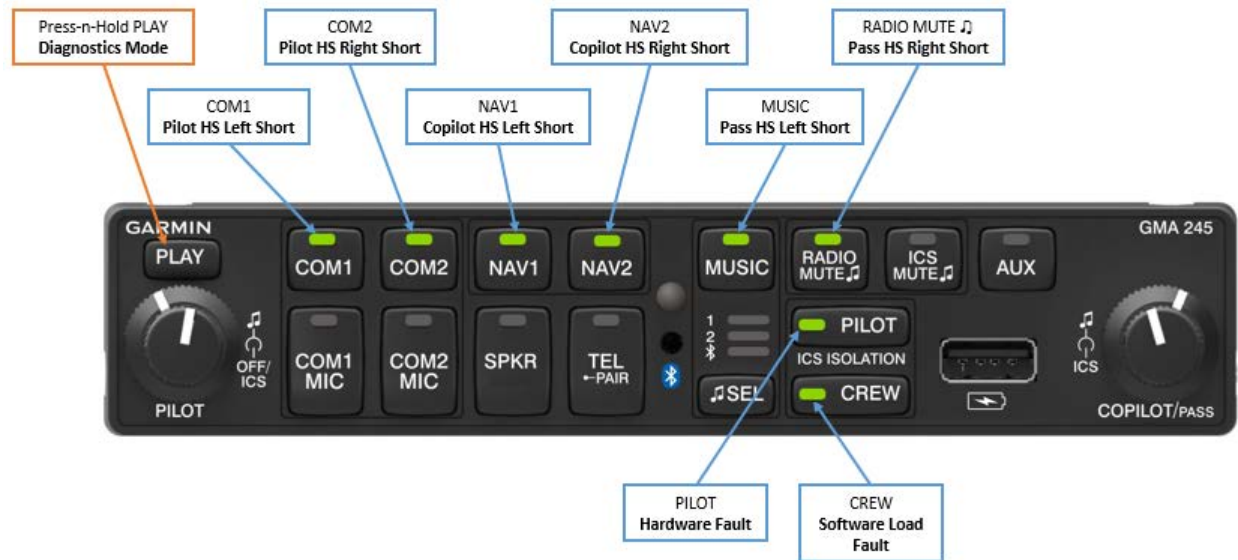
Figure 3-14 Diagnostics Mode
