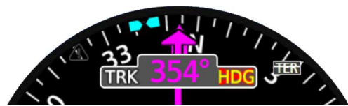
Figure 5- Top of the HSI when HDG failed (with GPS)
