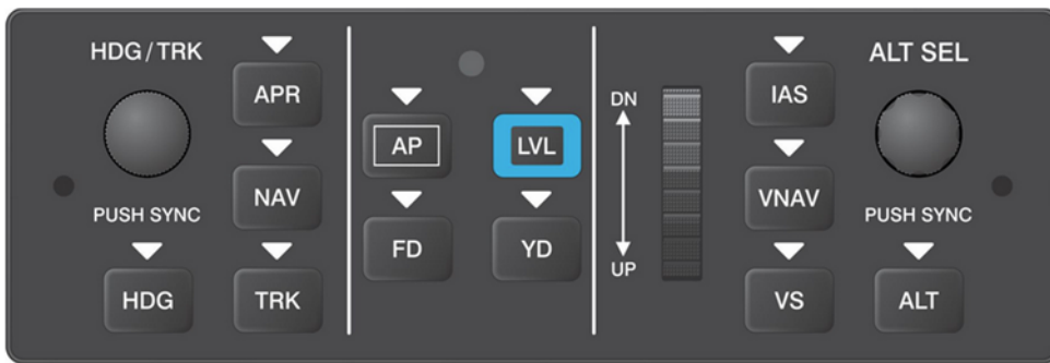
Figure 7-3: GMC 507 Control Unit (Reference Only)
