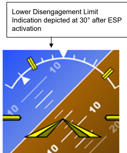
Figure 7-2: Engagement Limit Indications Upon ESP Activation
