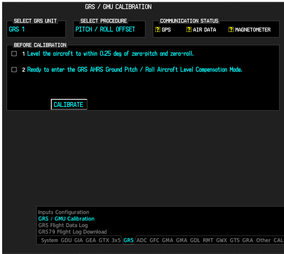
Figure 7-4, GRS/GMU Calibration, Pitch/Roll Offset
