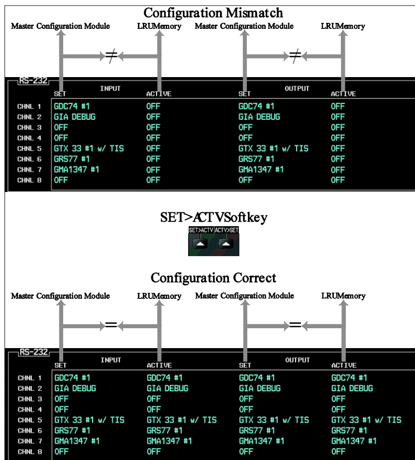
Figure 3-1, SET>ACTV Diagram
