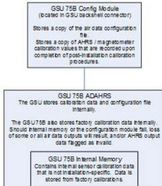
Figure 3-5, GSU Configuration Settings Storage (if GSU installed)
