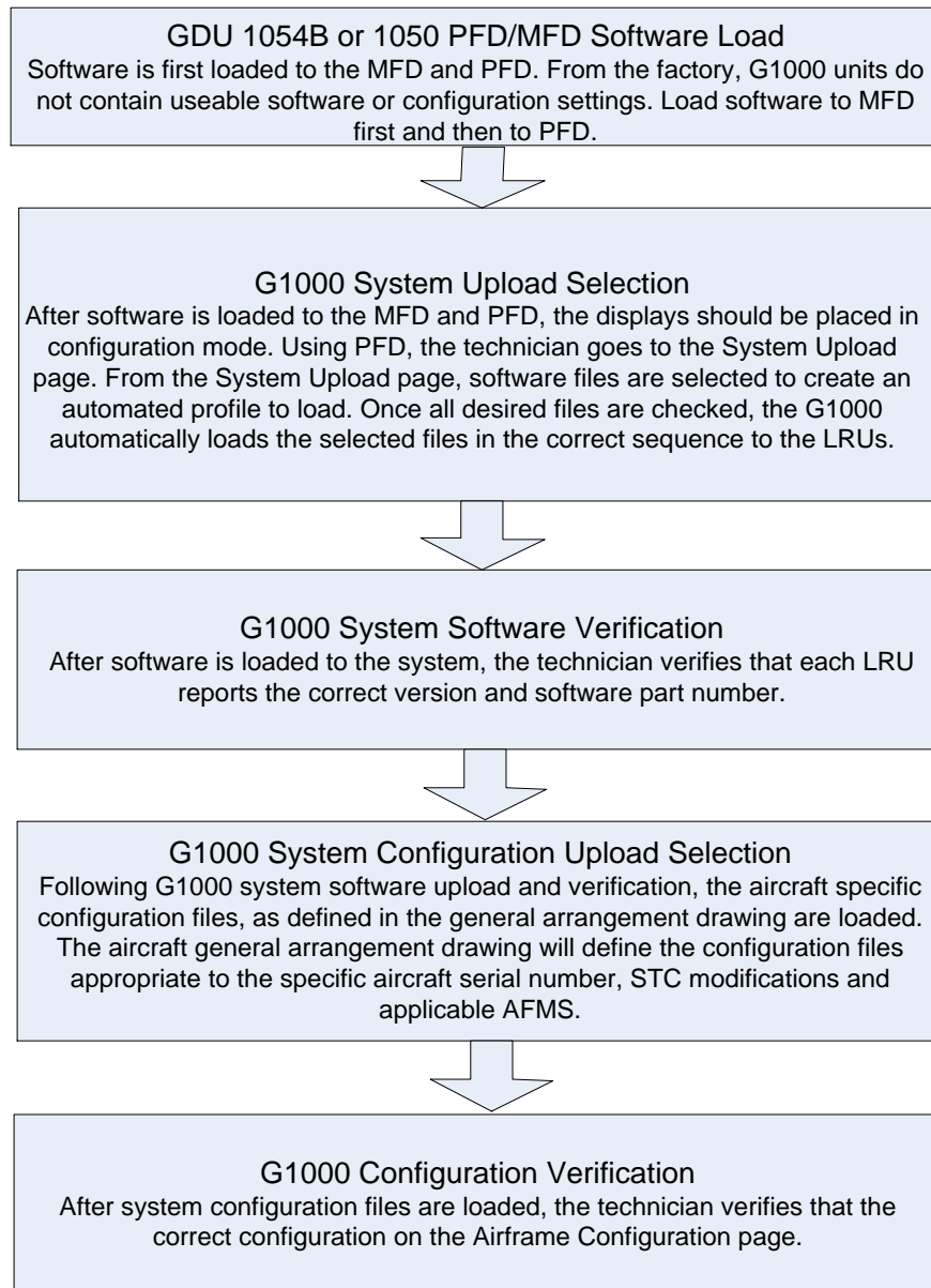
Figure 3-7, Software/Configuration Overview
