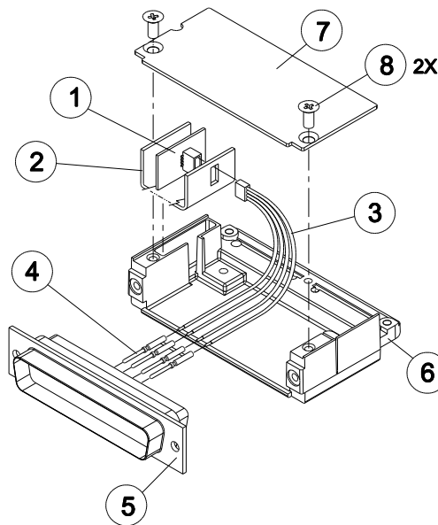
Figure 6-1, Configuration Module Installation
