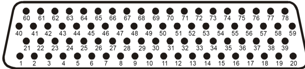
Figure 5-10, GSU 75 Connector View from Front (P751)
