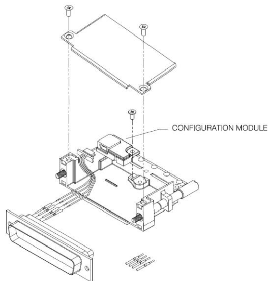
Figure 6-3, GSU 75 Configuration Module Installation
