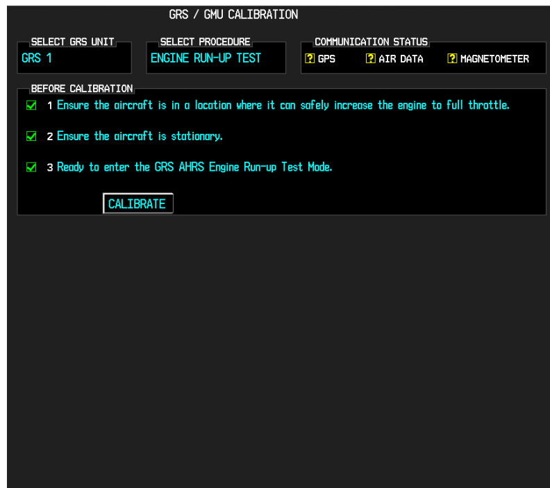
Figure 7-5, GRS/GMU Calibration, Engine Run-Up
