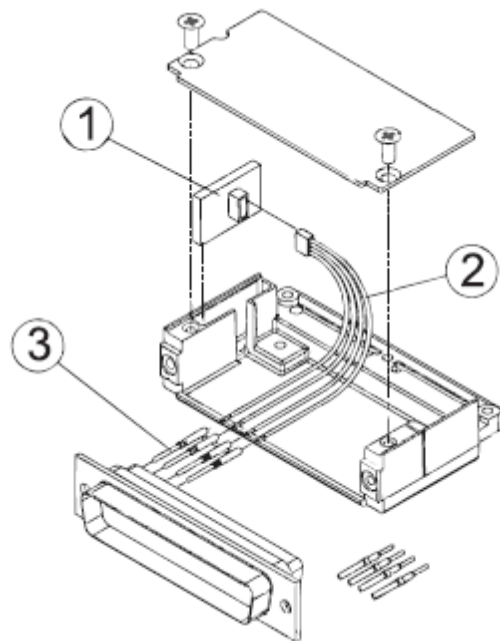
Figure 6-2, Configuration Module Installation
