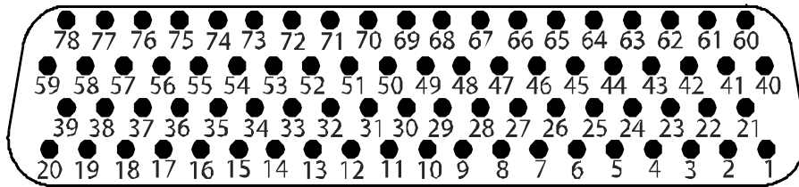
Figure 5-9, GDL 69A SXM Backplate Connector (P69A1)
