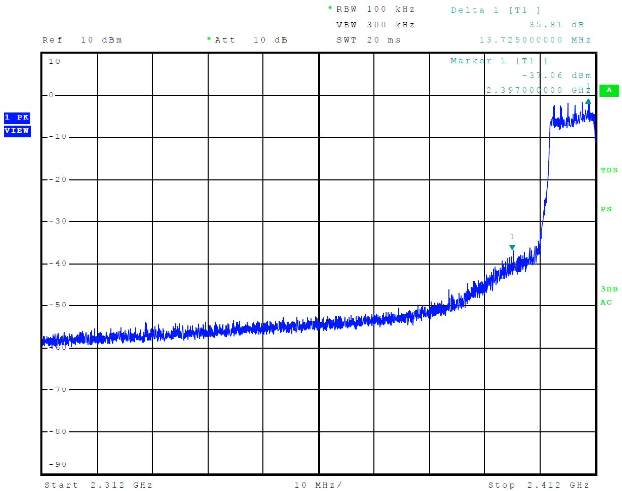
Figure 15 Plot of Transmitter Emissions Low Band Edge Mode 4 802.11g
