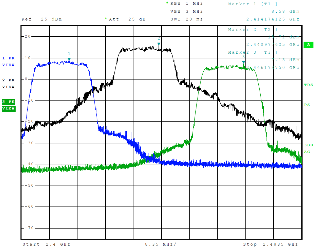
Figure 10 Plot of Transmitter Operation in 2412-2462 MHz Mode 4 802.11g
