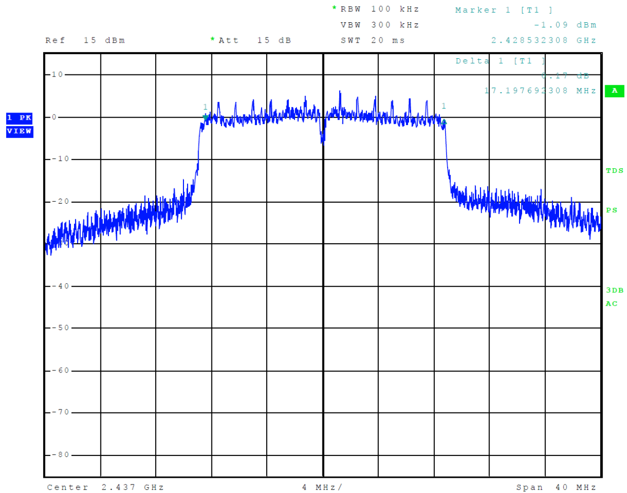
Figure 30 Plot of 6-dB Occupied Bandwidth Mode 5 802.11n
