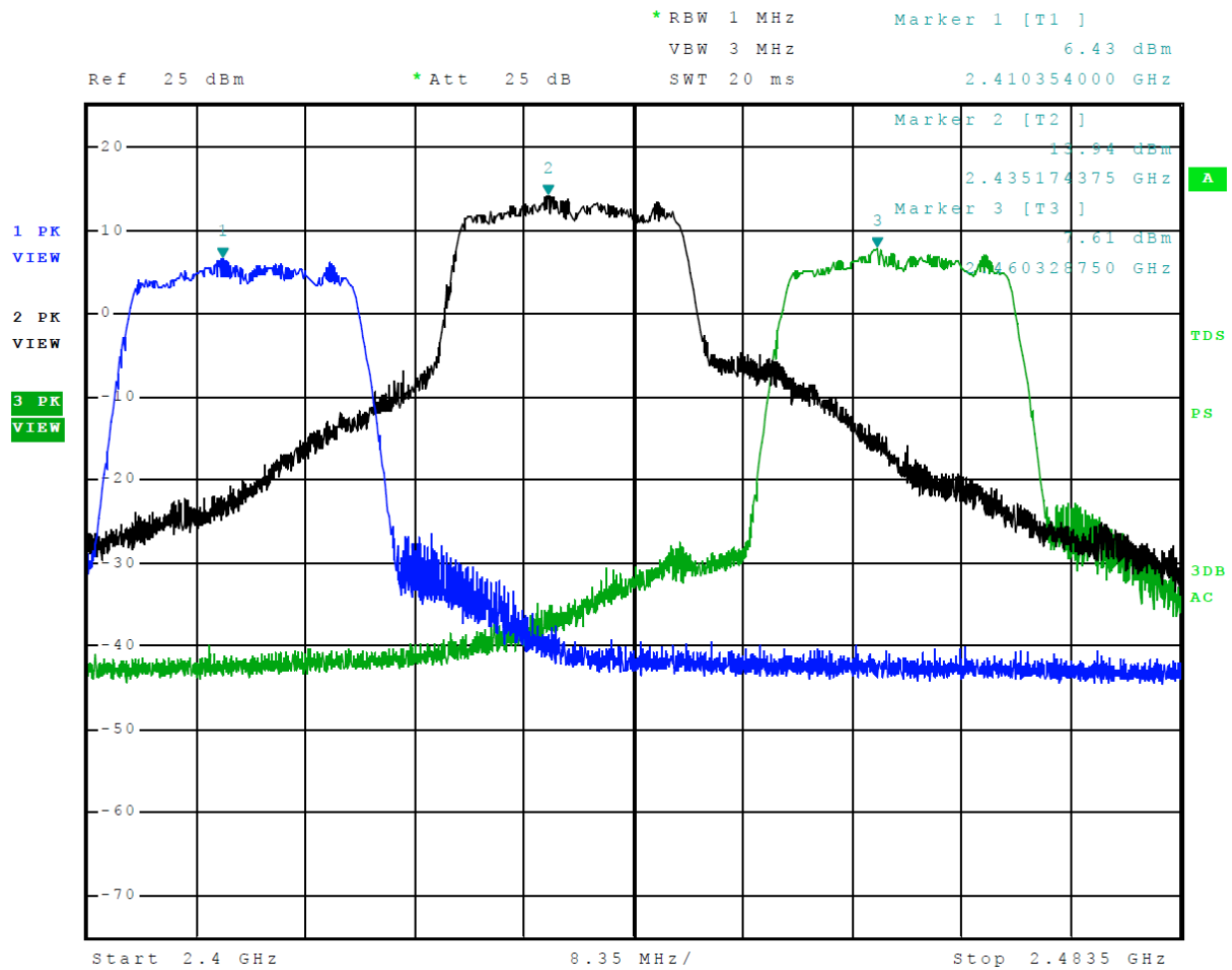
Figure 11 Plot of Transmitter Operation in 2412-2462 MHz Mode 5 802.11n
