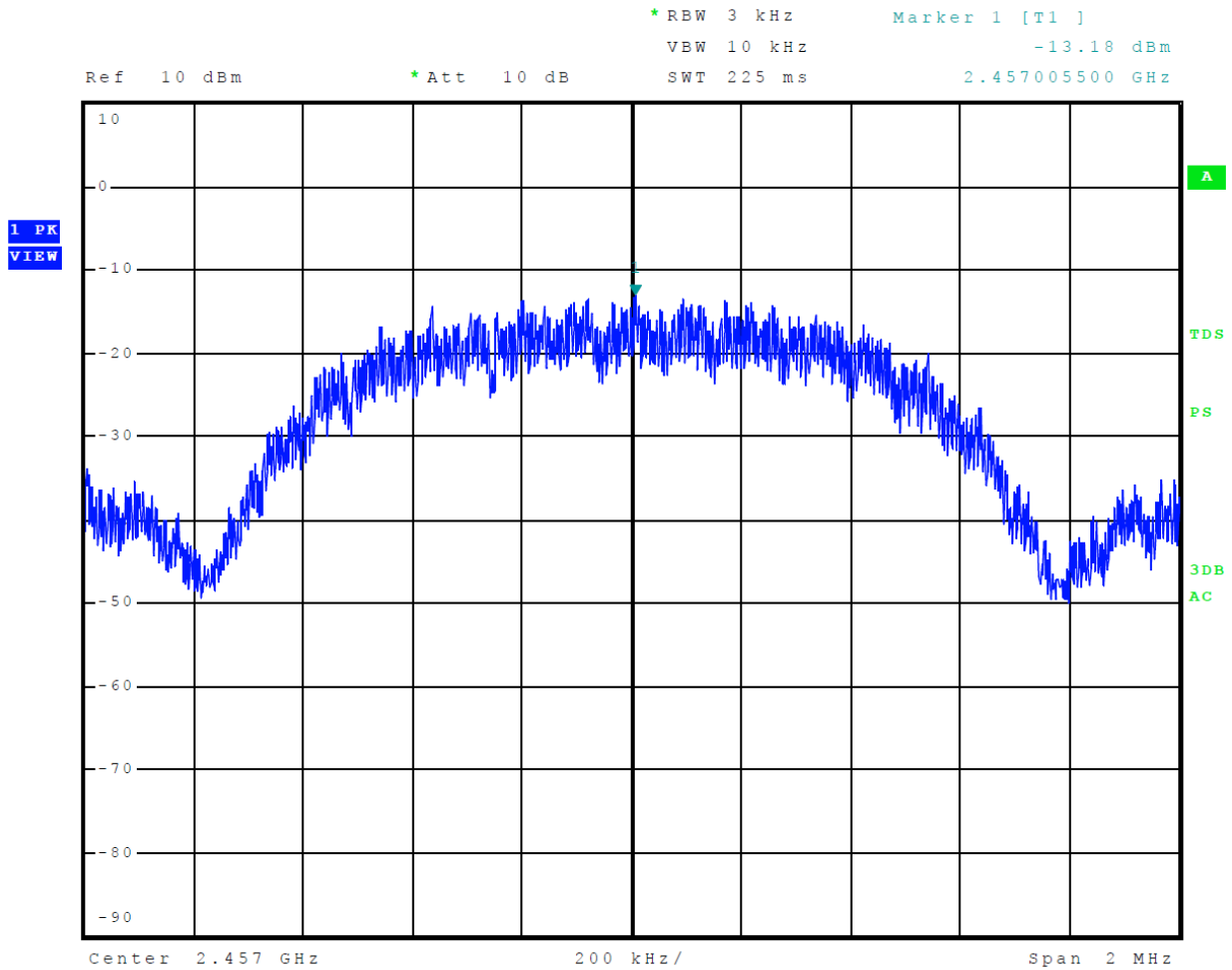
Figure 32 Plot of Transmitter Power Spectral Density Mode 1 ANT
