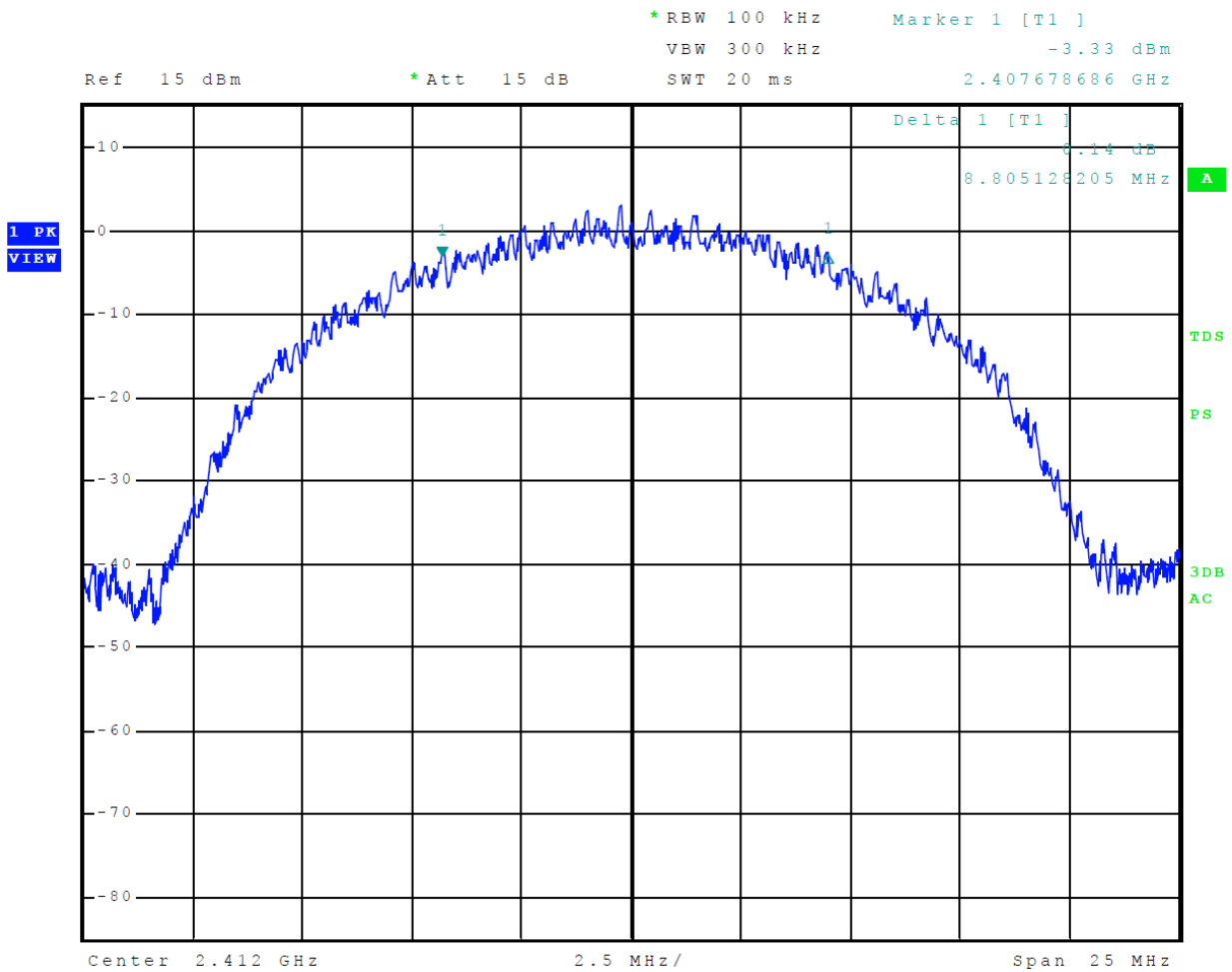
Figure 26 Plot of 6-dB Occupied Bandwidth Mode 3 802.11b
