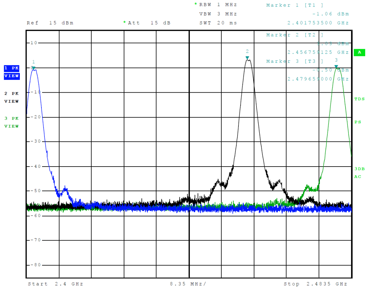
Figure 7 Plot of Transmitter Emissions Operation in 2402-2480 MHz Mode 1 ANT
