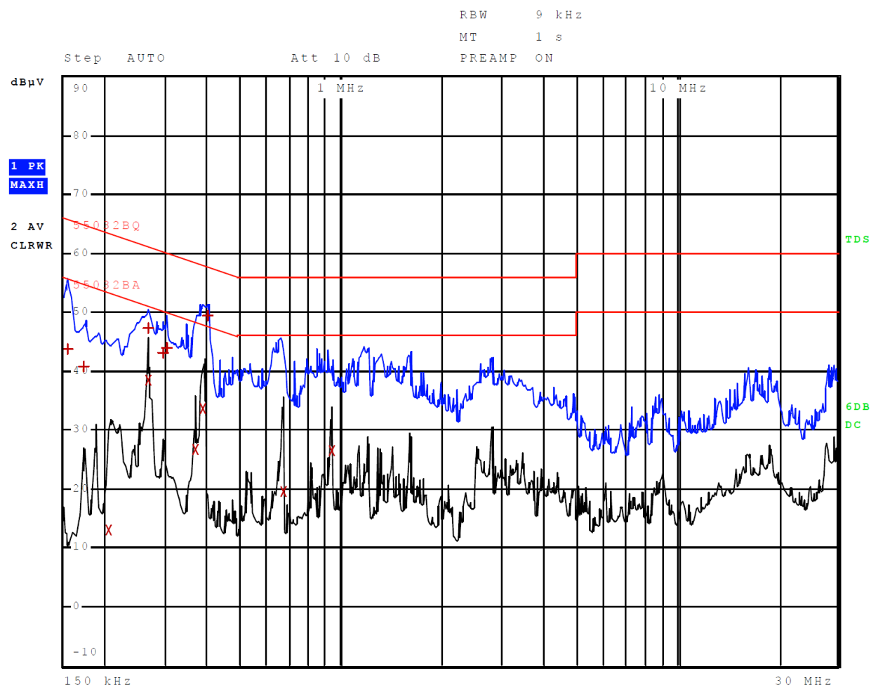
Figure 6 AC Line Conducted emissions of EUT line 2 (EUT – Computer)
