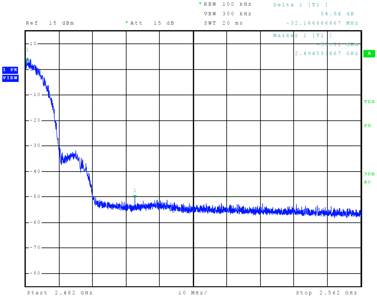
Figure 19 Plot of Transmitter Emissions High Band Edge Mode 3 802.11b
