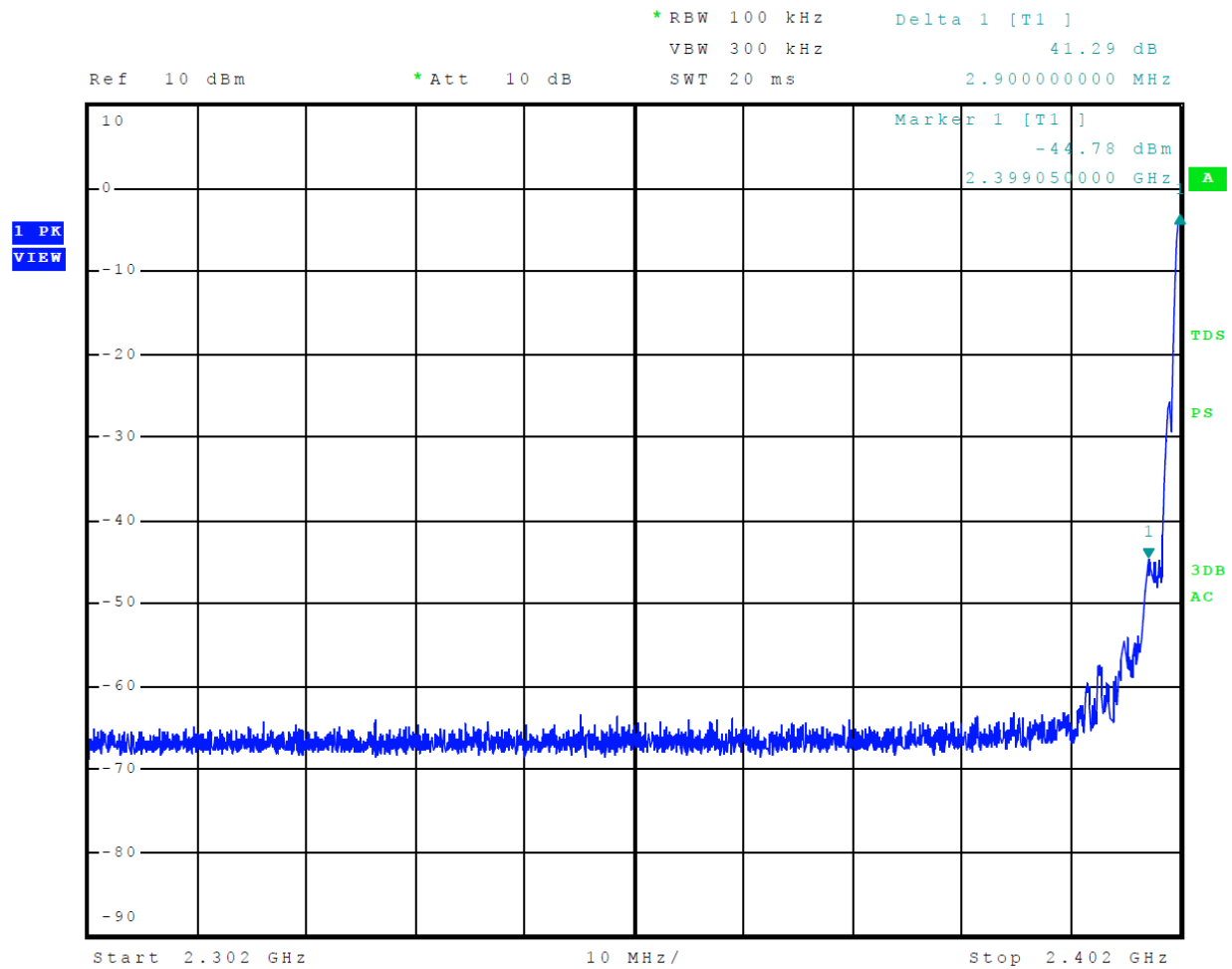
Figure 13 Plot of Transmitter Emissions Low Band Edge Mode 2 BLE
