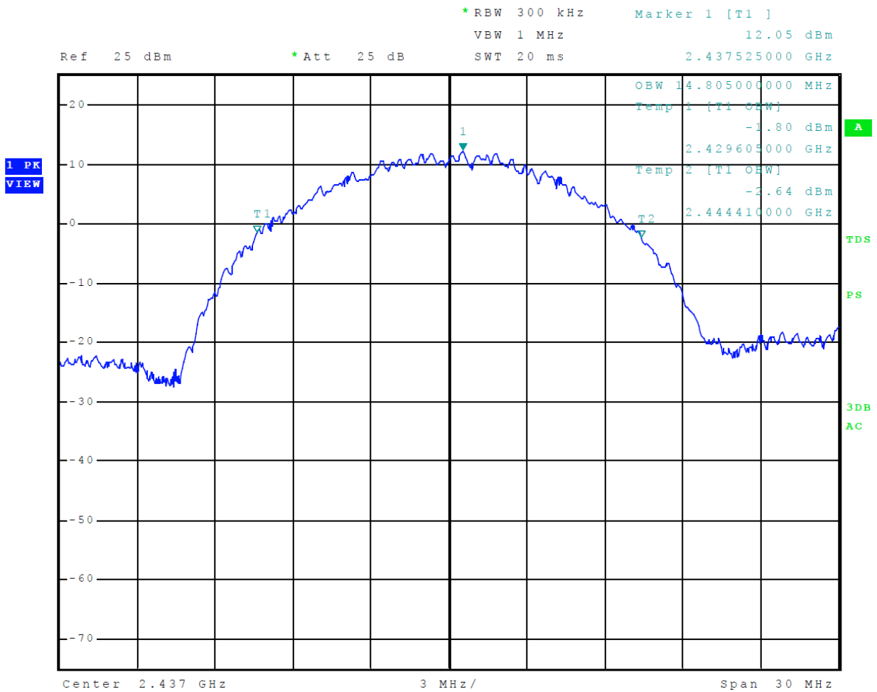
Figure 27 Plot of 99% Occupied Bandwidth Mode 3 802.11b
