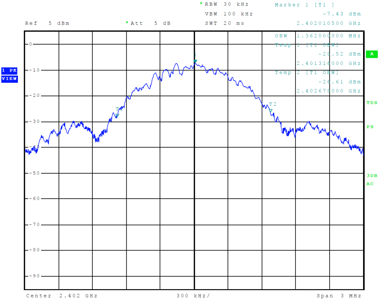
Figure 25 Plot of 99% Occupied Bandwidth Mode 2 BLE
