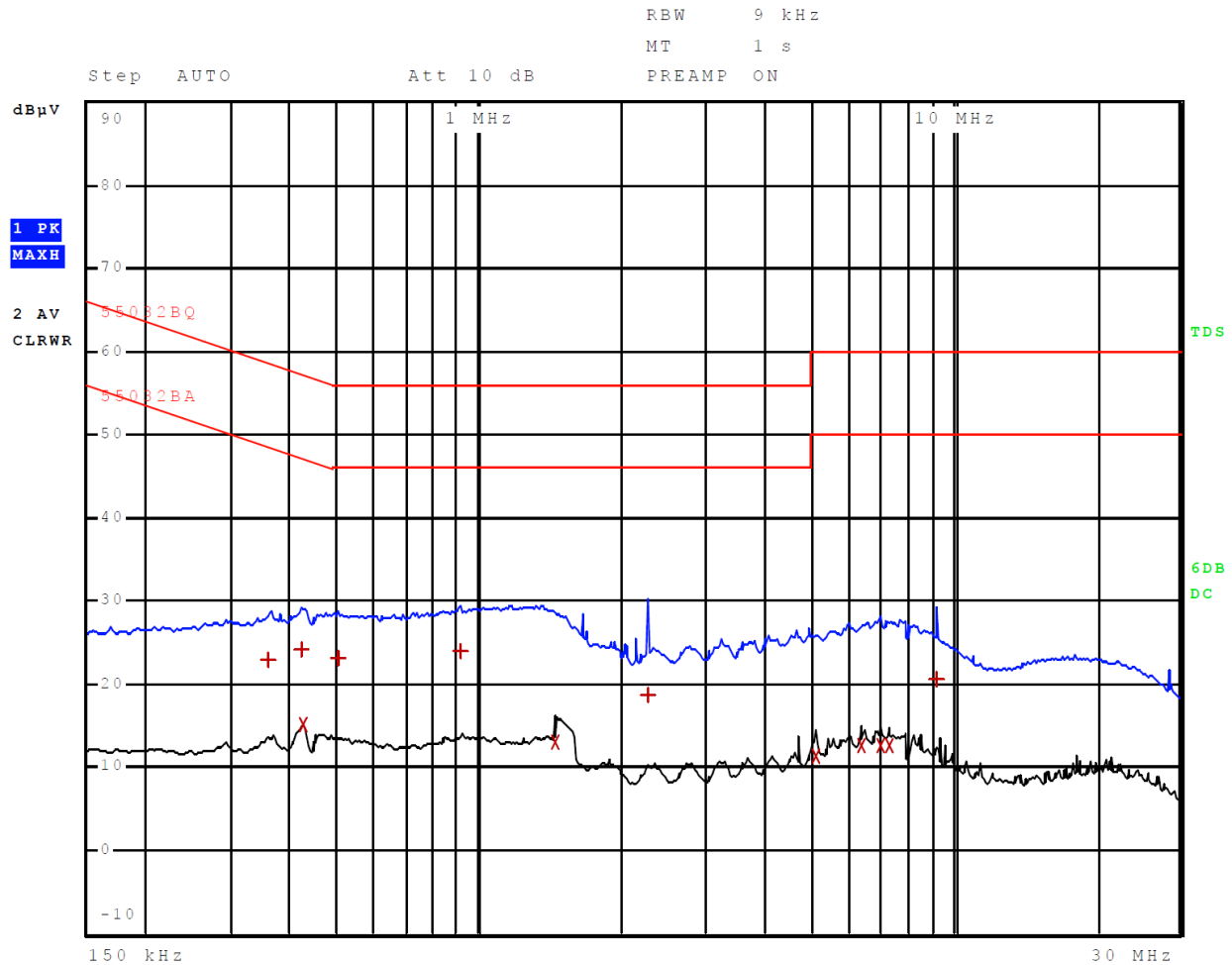
Figure 4 AC Line Conducted emissions of EUT line 2 (EUT – USB-C AC Adapter)
