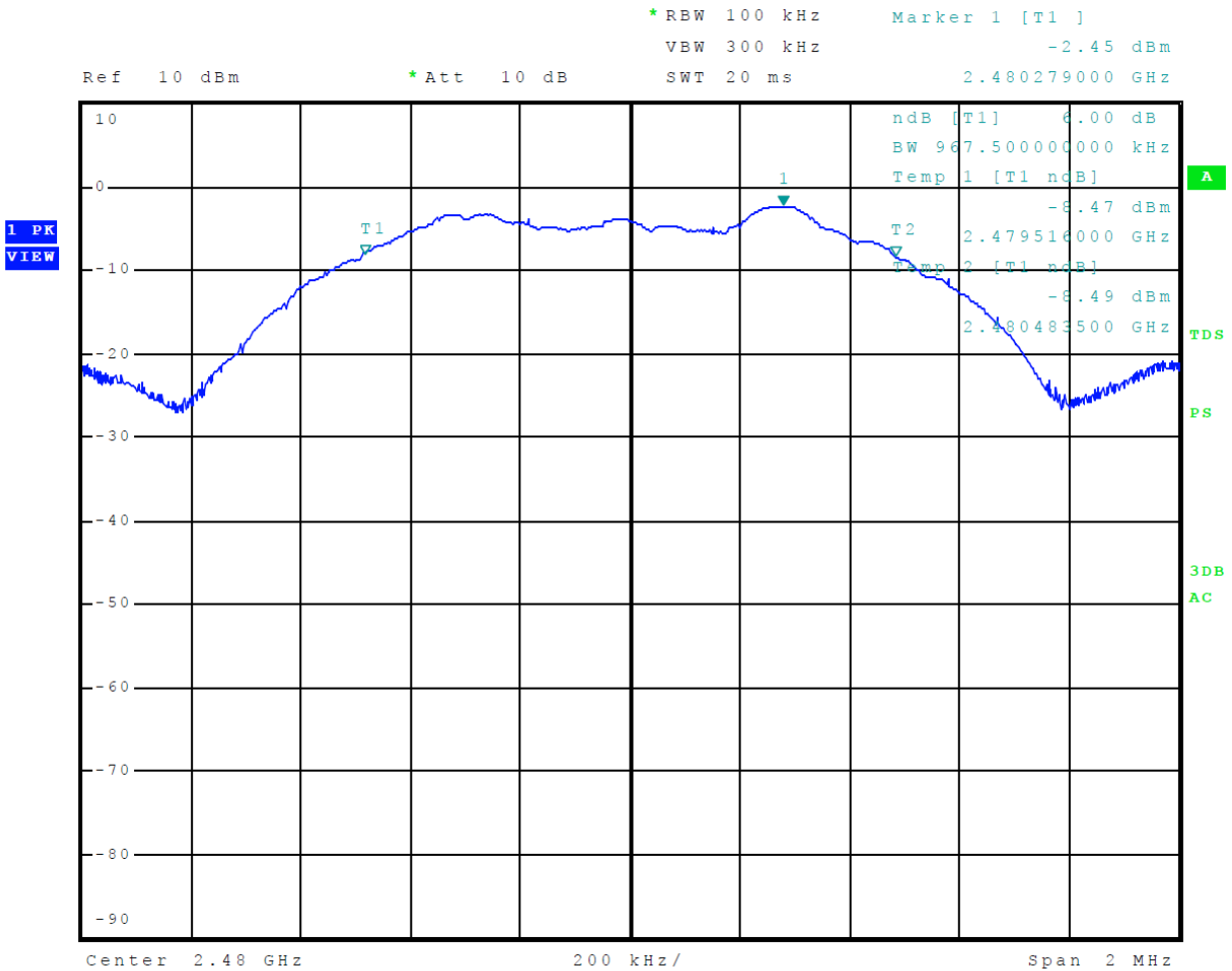
Figure 22 Plot of 6-dB Occupied Bandwidth Mode 1 ANT
