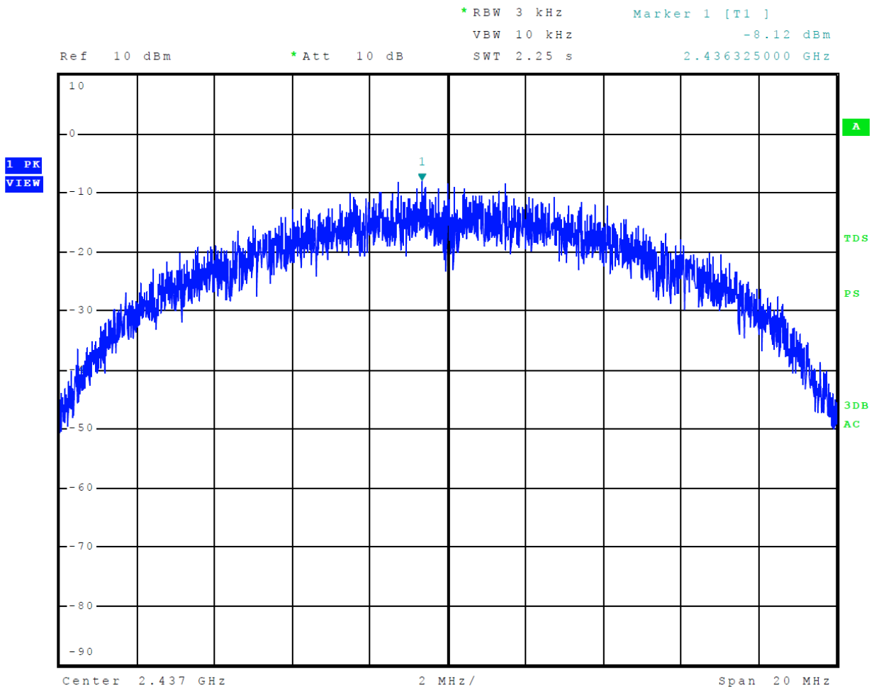
Figure 34 Plot of Transmitter Power Spectral Density Mode 3 802.11b
