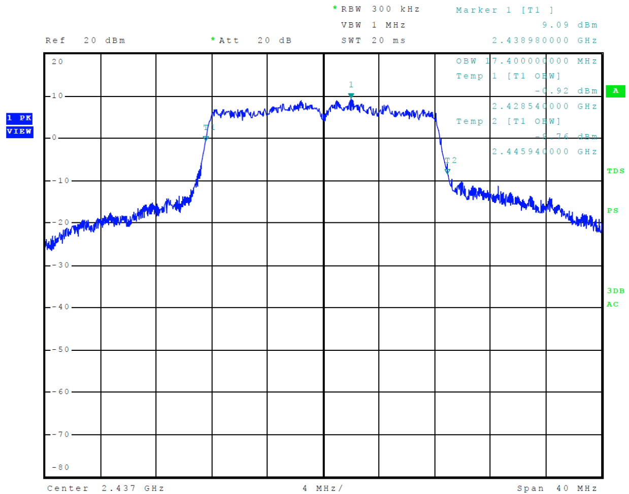
Figure 29 Plot of 99% Occupied Bandwidth Mode 4 802.11g
