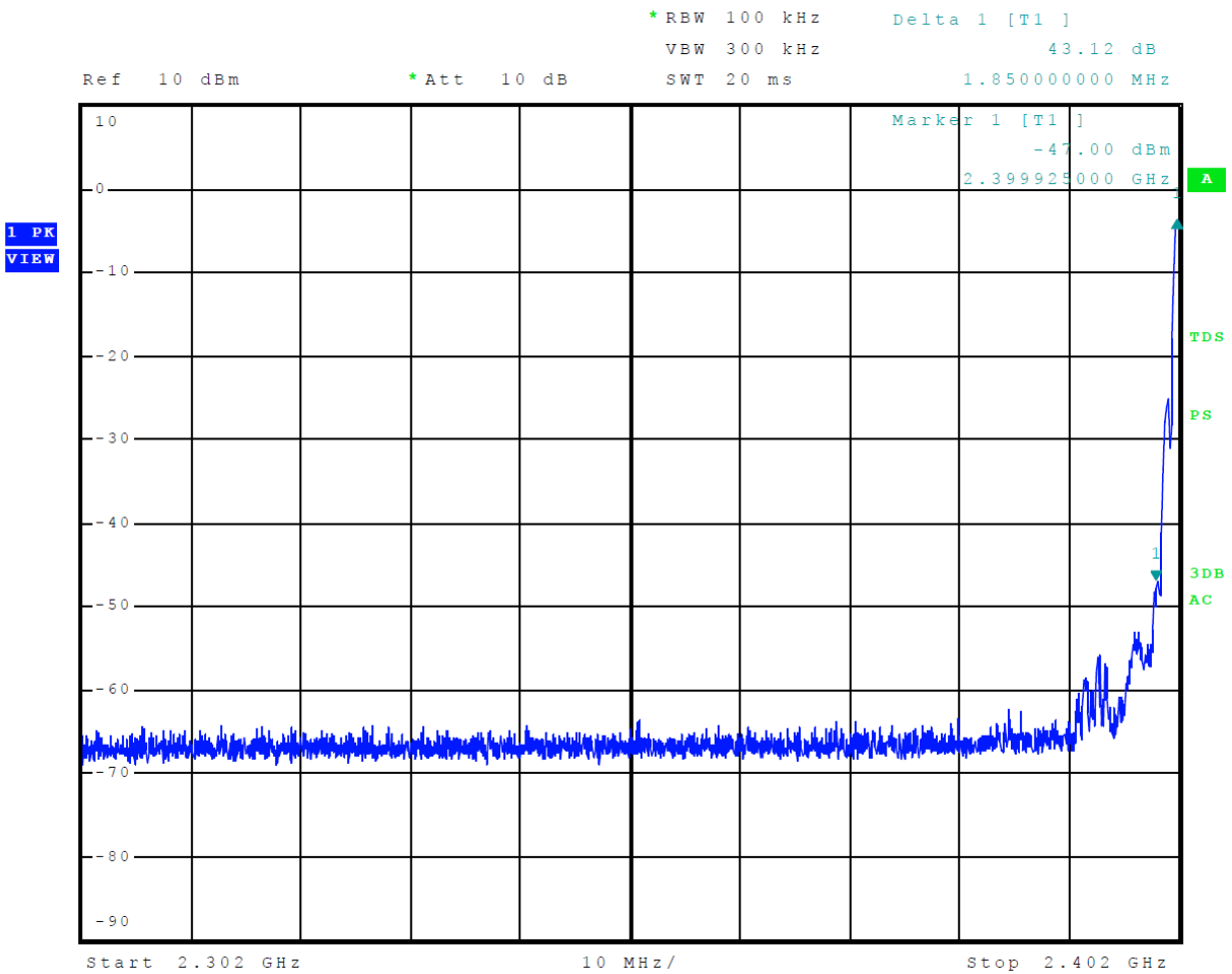
Figure 12 Plot of Transmitter Emissions Low Band Edge Mode 1 ANT
