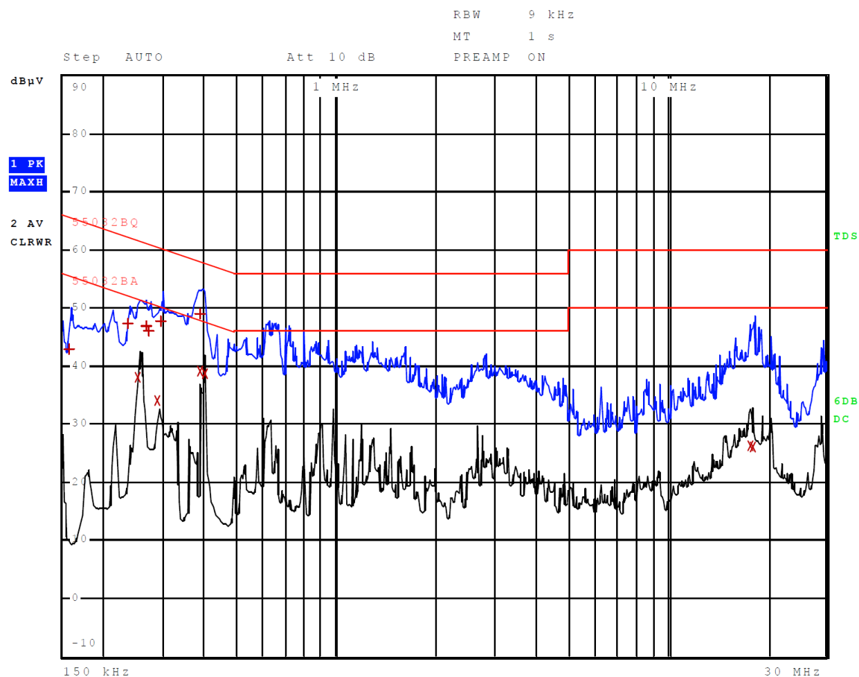
Figure 5 AC Line Conducted emissions of EUT line 1 (EUT – Computer)
