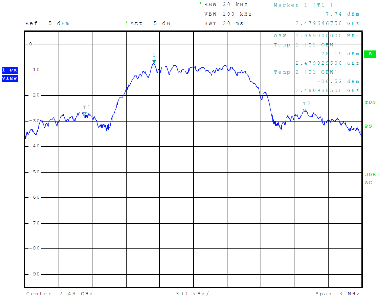
Figure 23 Plot of 99% Occupied Bandwidth Mode 1 ANT
