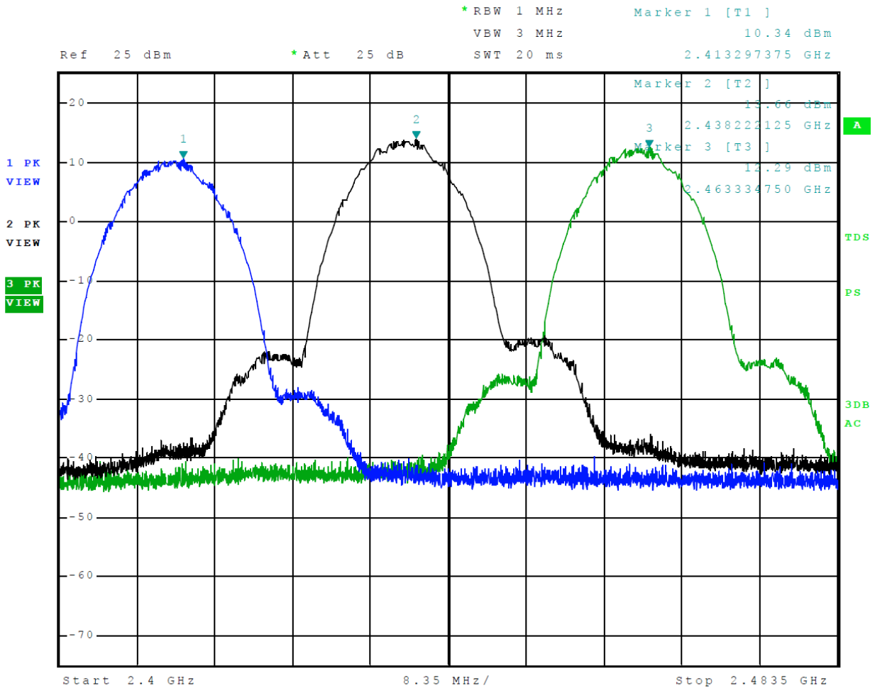
Figure 9 Plot of Transmitter Operation in 2412-2462 MHz Mode 3 802.11b
