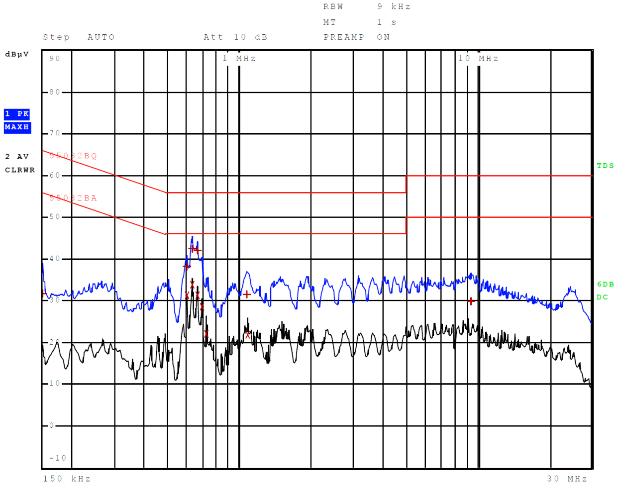
Figure 1 AC Line Conducted emissions of EUT line 1 (EUT – USB-A AC Adapter)
