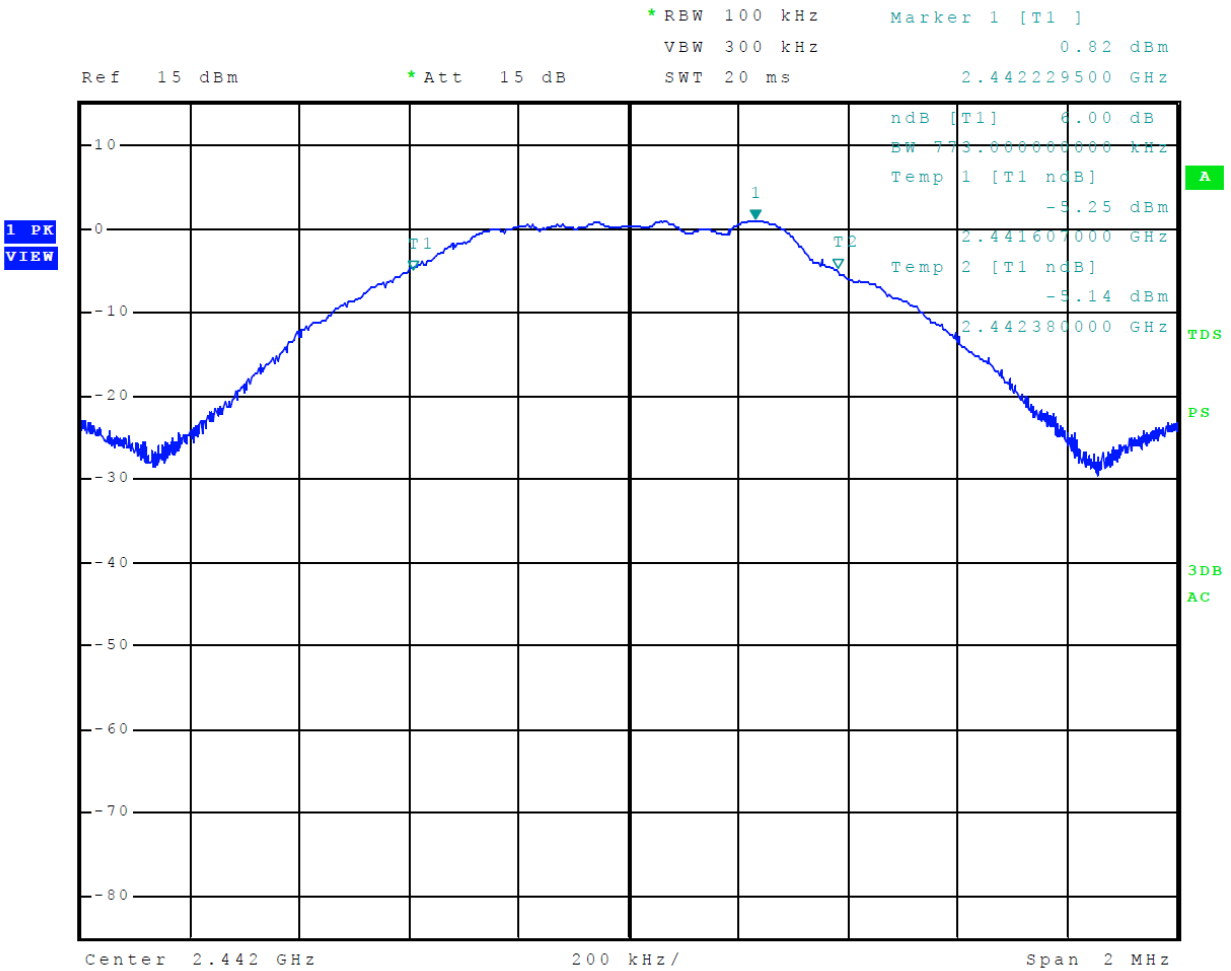
Figure 24 Plot of 6-dB Occupied Bandwidth Mode 2 BLE
