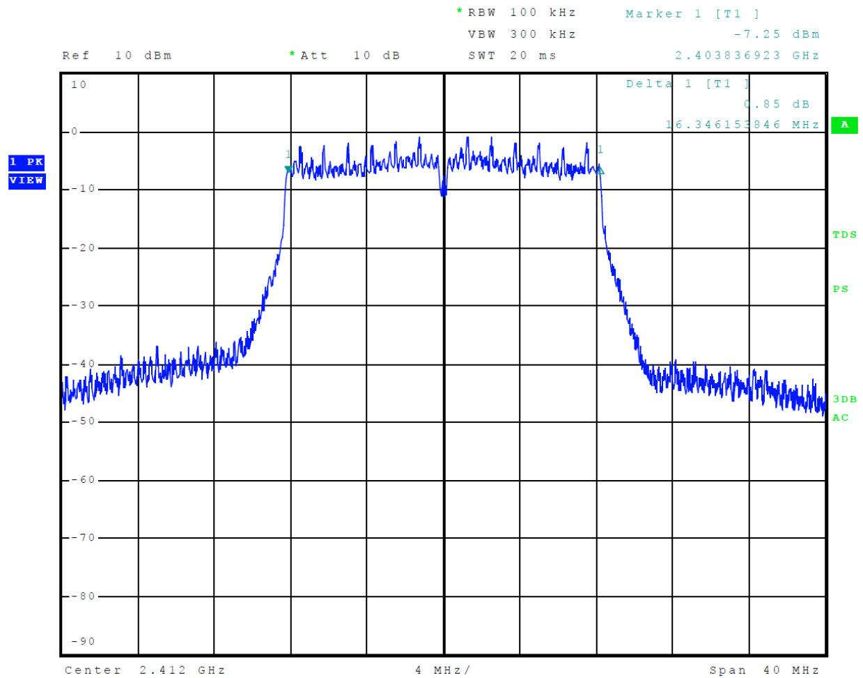
Figure 28 Plot of 6-dB Occupied Bandwidth Mode 4 802.11g
