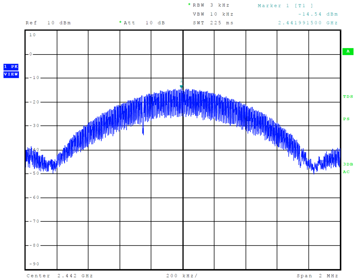
Figure 33 Plot of Transmitter Power Spectral Density Mode 2 BLE
