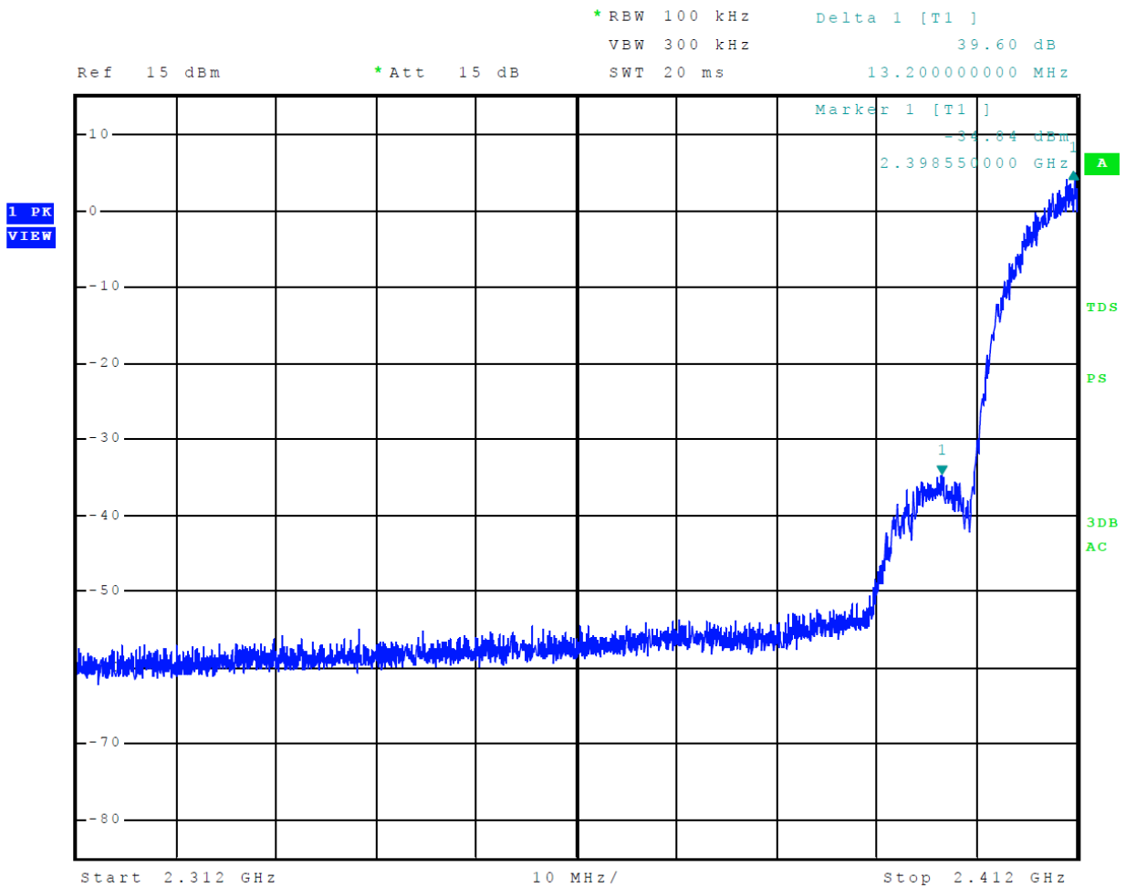
Figure 14 Plot of Transmitter Emissions Low Band Edge Mode 3 802.11b
