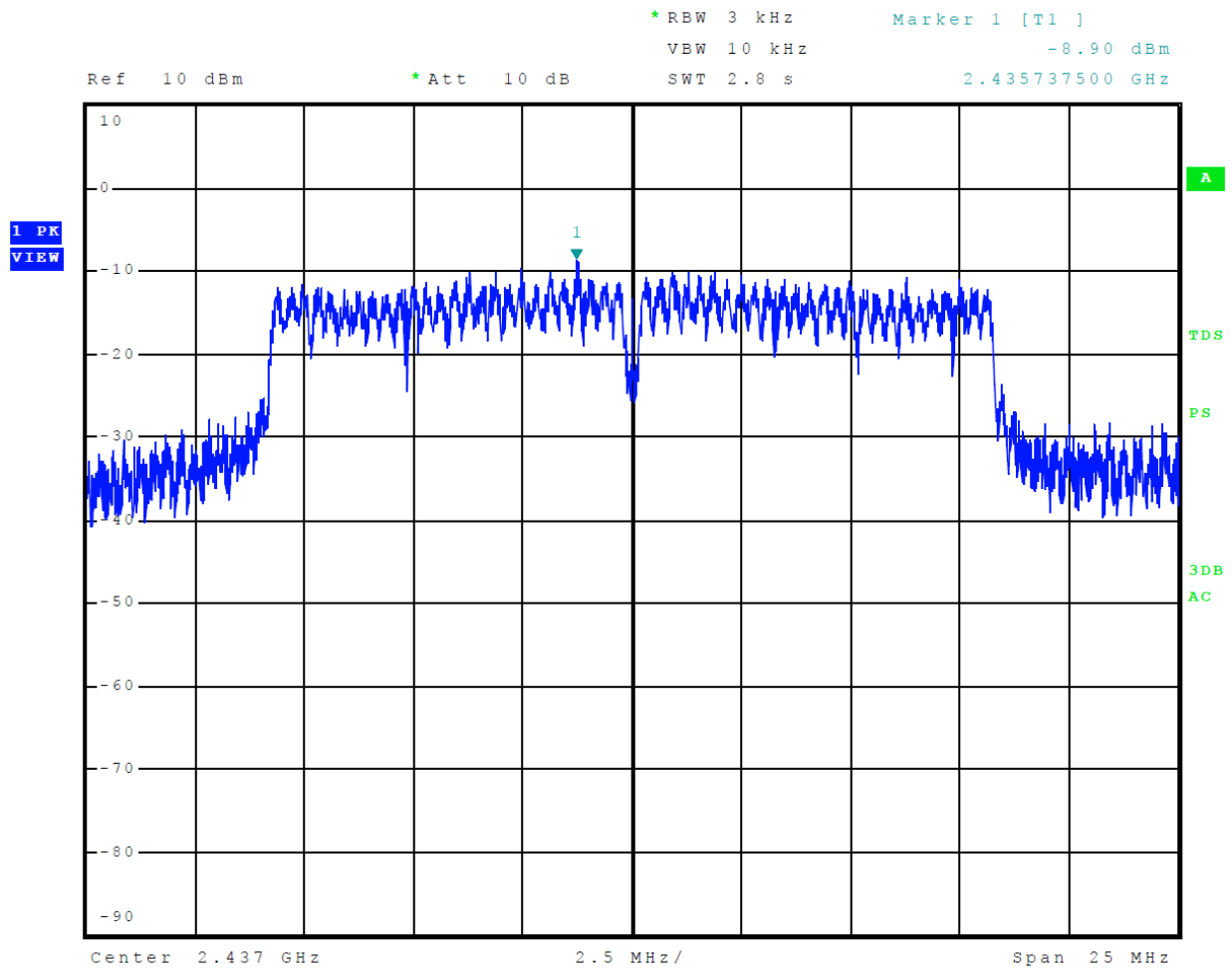
Figure 35 Plot of Transmitter Power Spectral Density Mode 4 802.11g
