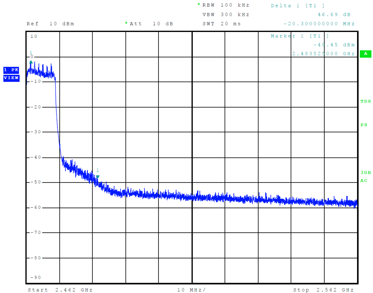
Figure 21 Plot of Transmitter Emissions High Band Edge Mode 5 802.11n
