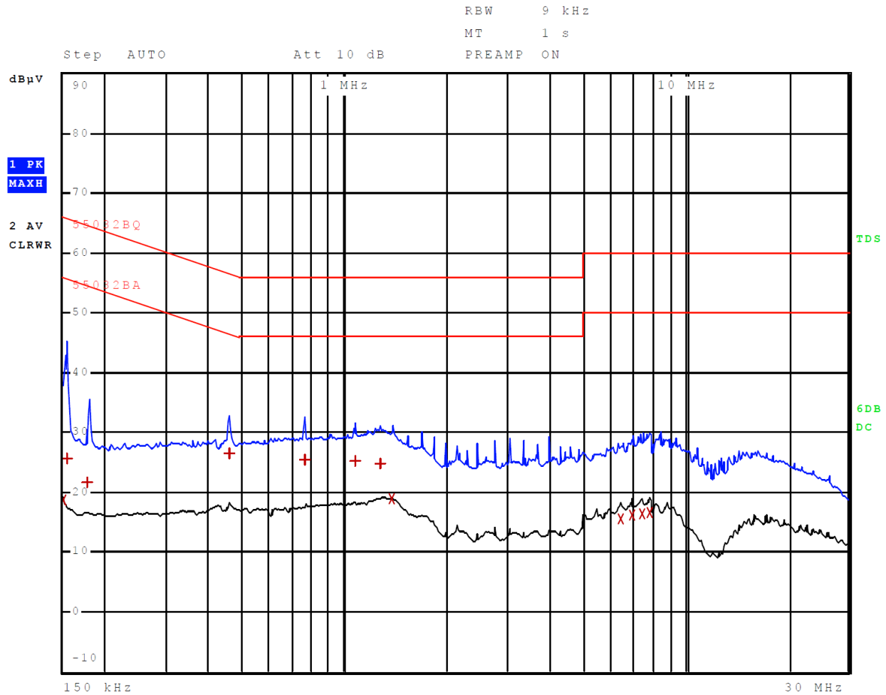
Figure 3 AC Line Conducted emissions of EUT line 1 (EUT – USB-C AC Adapter)
