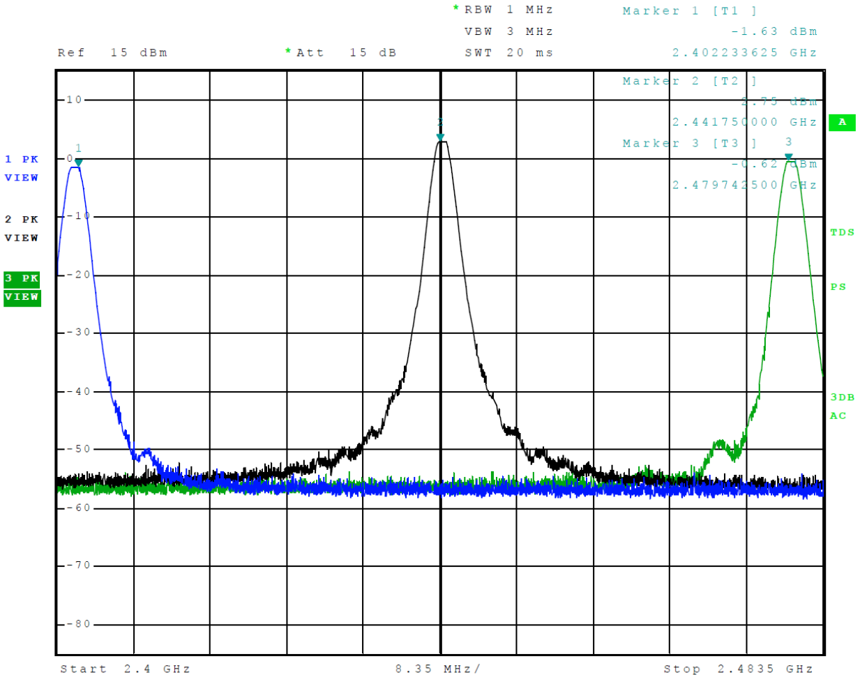
Figure 8 Plot of Transmitter Emissions Operation in 2402-2480 MHz Mode 2 BLE
