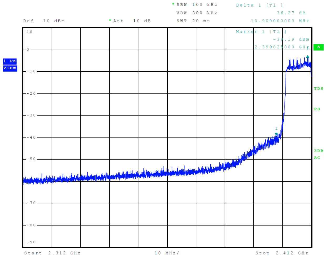
Figure 16 Plot of Transmitter Emissions Low Band Edge Mode 5 802.11n
