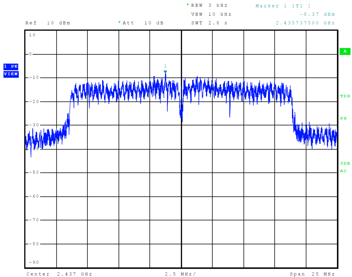
Figure 36 Plot of Transmitter Power Spectral Density Mode 5 802.11n
