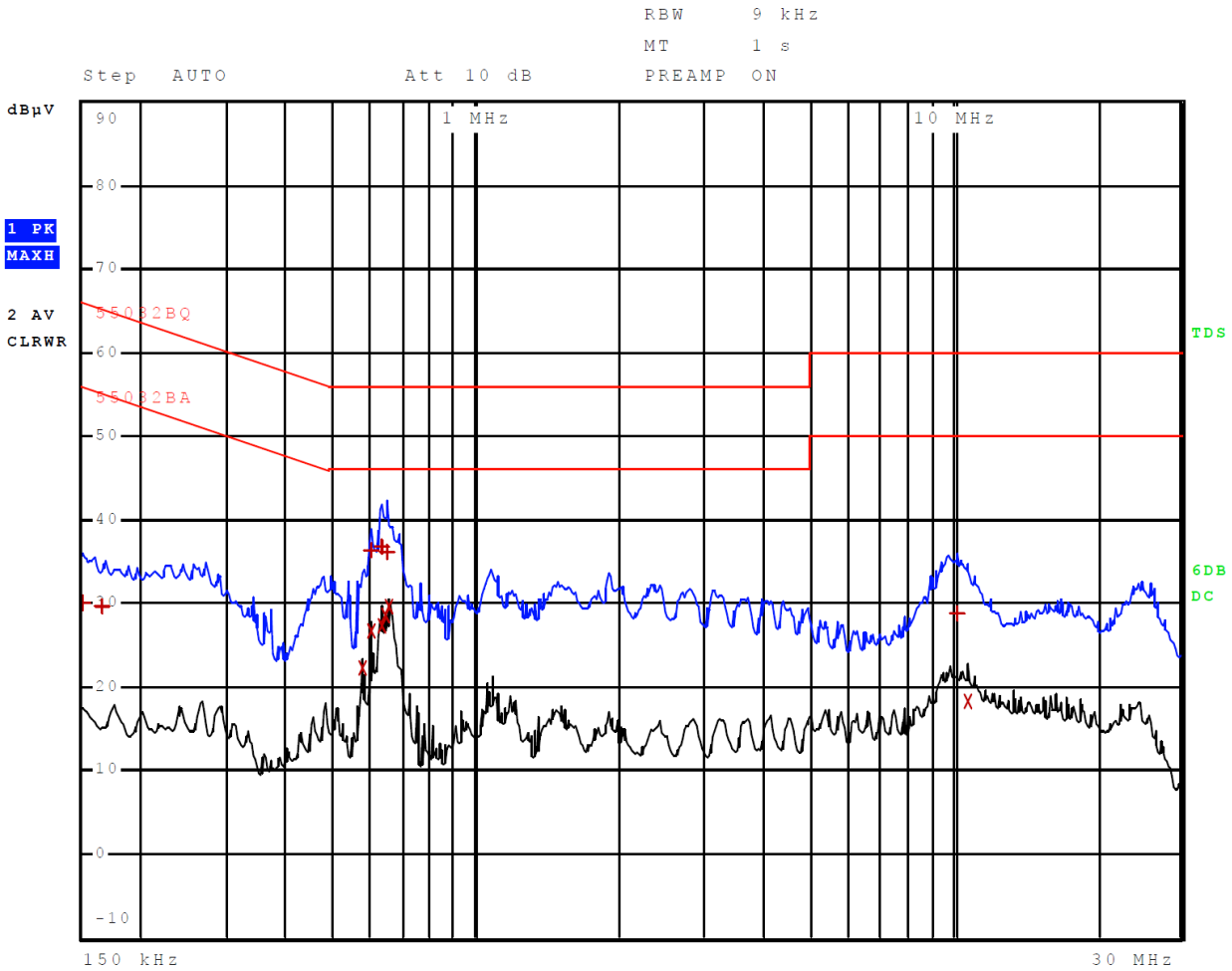
Figure 2 AC Line Conducted emissions of EUT line 2 (EUT – USB-A AC Adapter)
