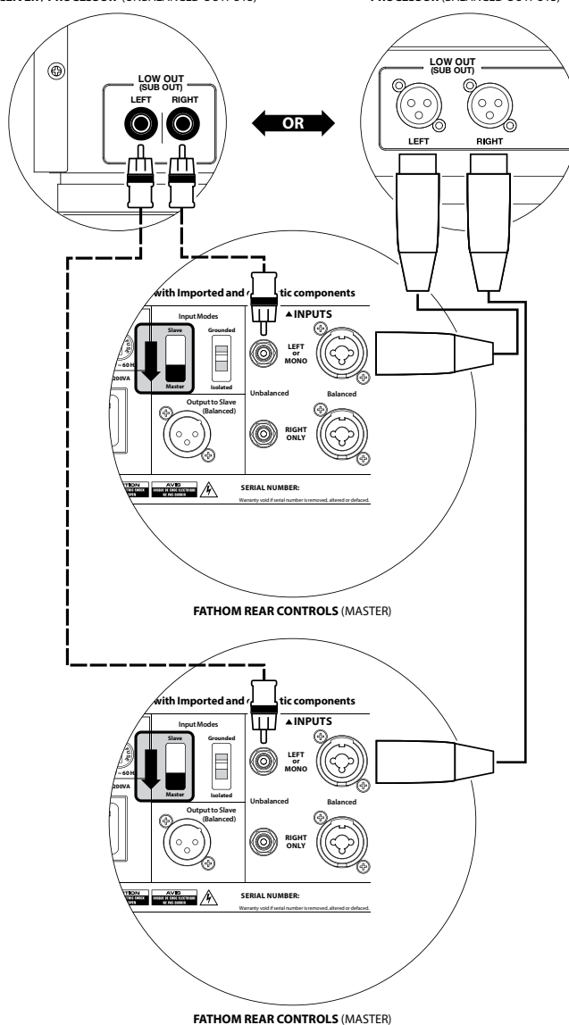
RECEIVER / PROCESSOR (UNBALANCED OUTPUTS)
