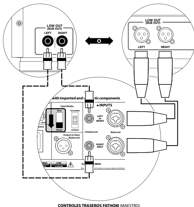
CONTROLES TRASEROS FATHOM (MAESTRO)
