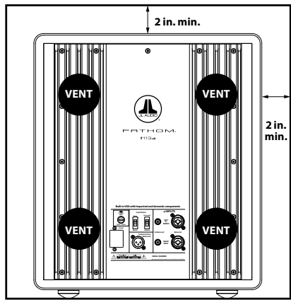
Rear-view of cabinet install (f110, f112, f113):
