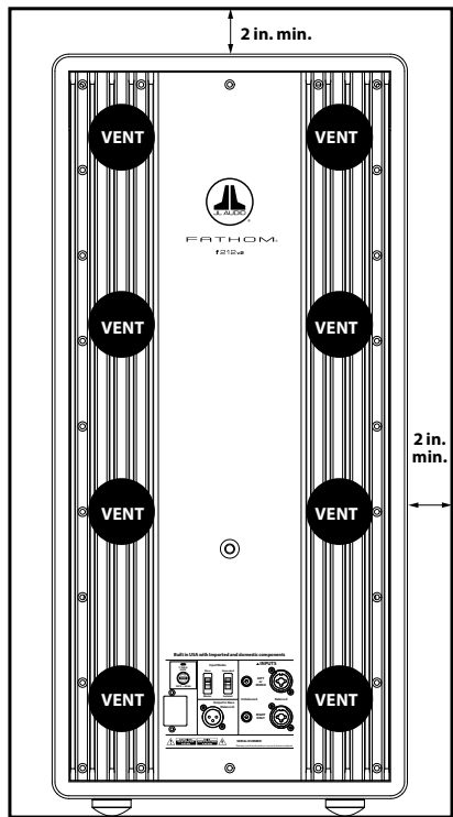
Rear-view of cabinet install (f212):
