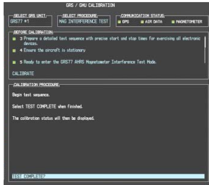
Figure 5-4. Magnetometer Interference Test
