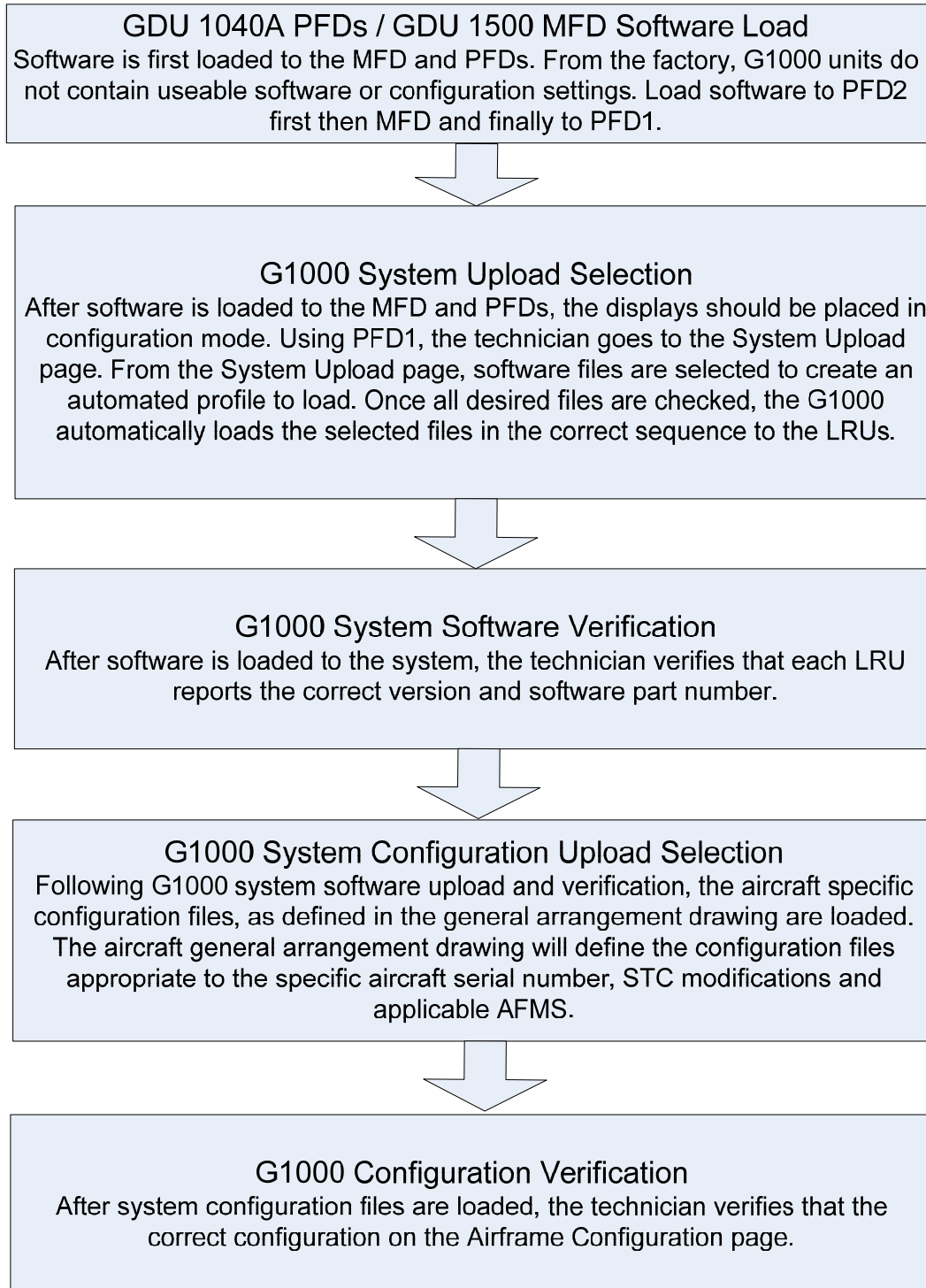
Figure 2-1. Software/Configuration Overview
