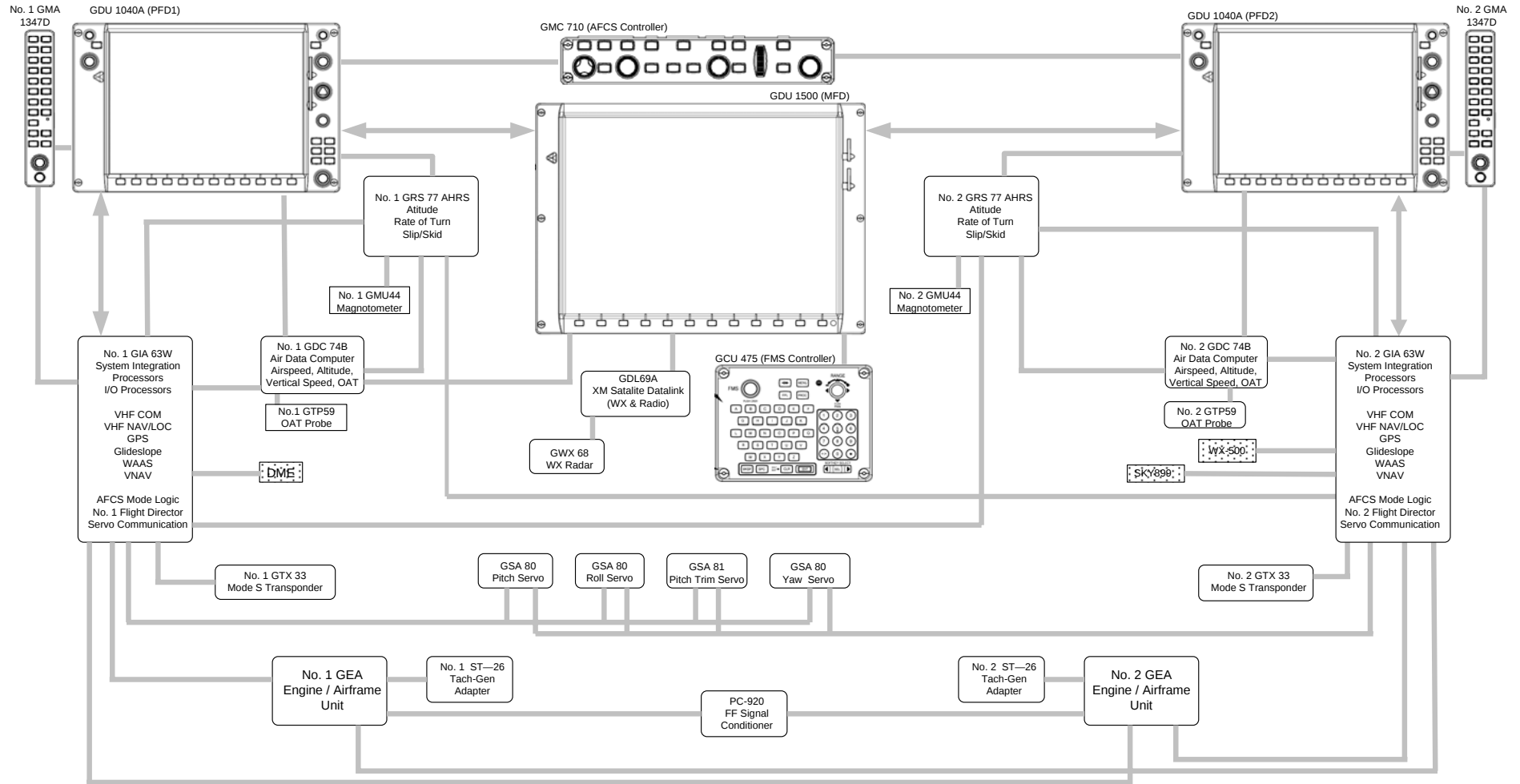
Figure 1-1. G1000 & GFC 700 in King Air C90A/C90GT
