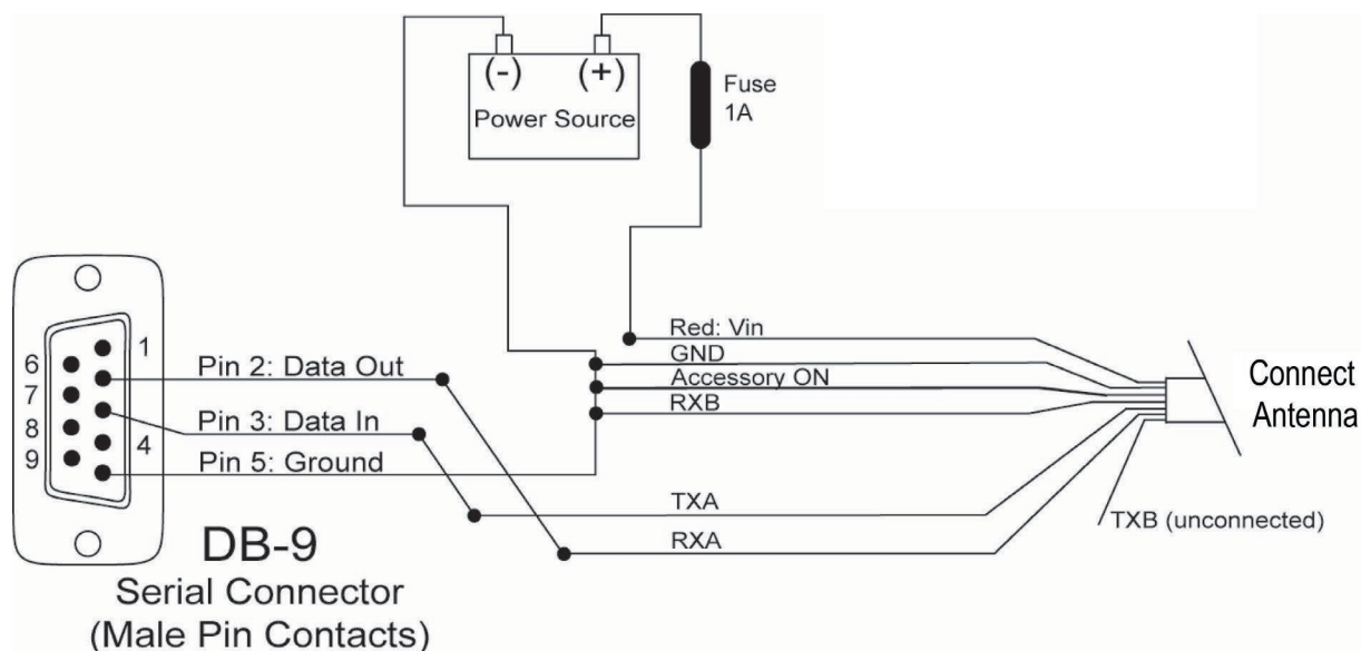
Figure 2. PDA Serial Port Interconnection
