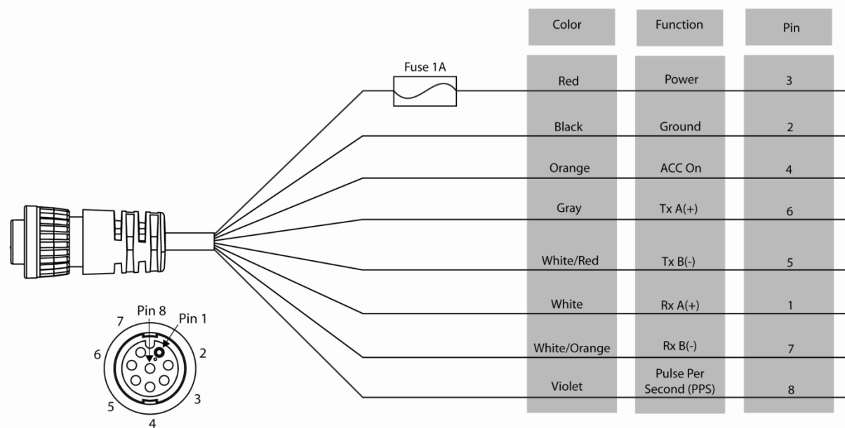
Figure 3b. GPS 24xd NMEA 0183 HVS Power/Data Cable
