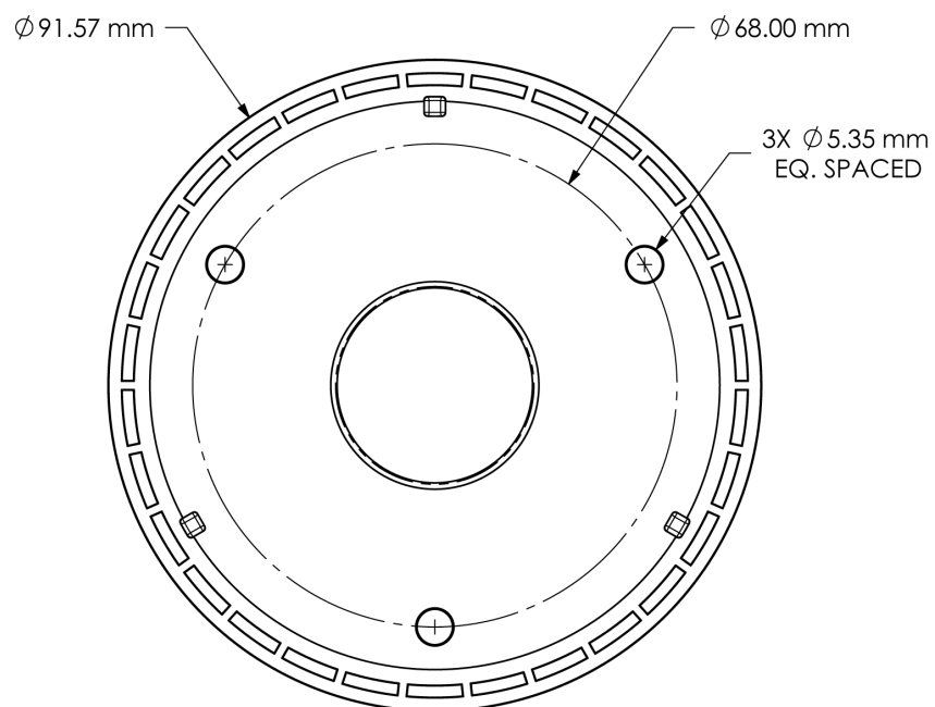
Figure 4. GPS 24xd Bottom Case Dimensions
