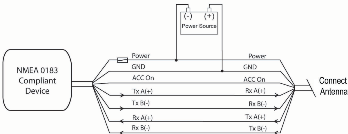
Figure 3a. GPS 24xd NMEA 0183 HVS Wired for Two-Way Communication
