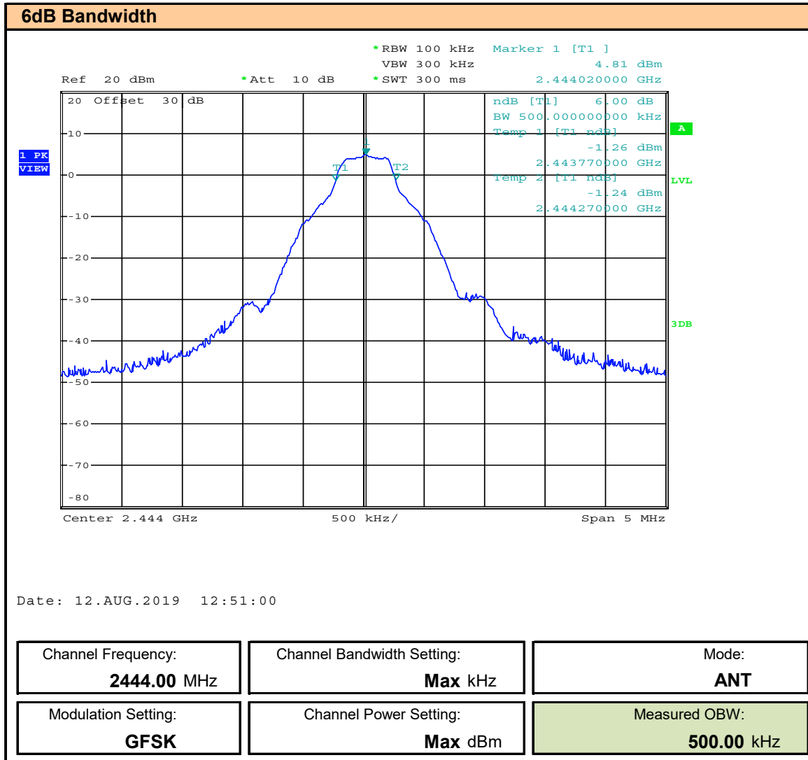
Plot 9.2 – 6dB Bandwidth, 2444MHz, ANT
