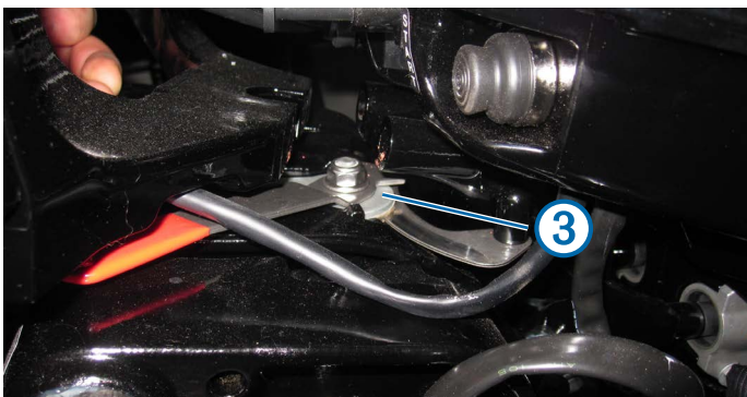
Removing the Tiller Lock
