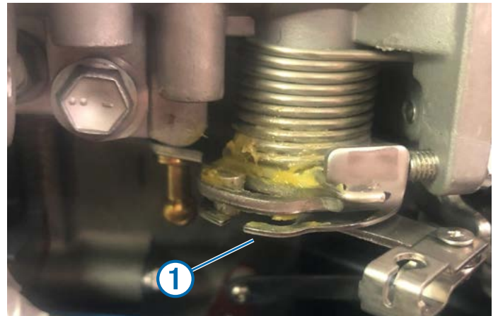
Closeup of Throttle Lever Installed on Yamaha Throttle Shaft
