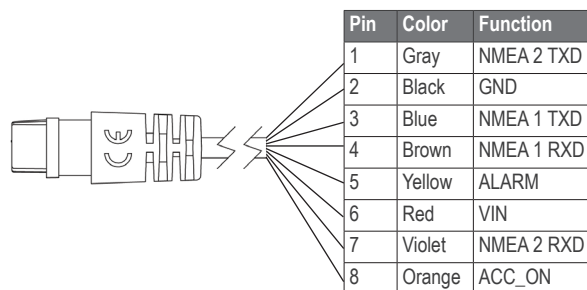
GPSMAP 7400/7600 Series Power Cable
